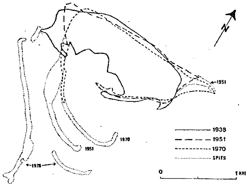
Fig. 8. Shoreline Changes 1938 - 1970. Tuckernuck Island.
