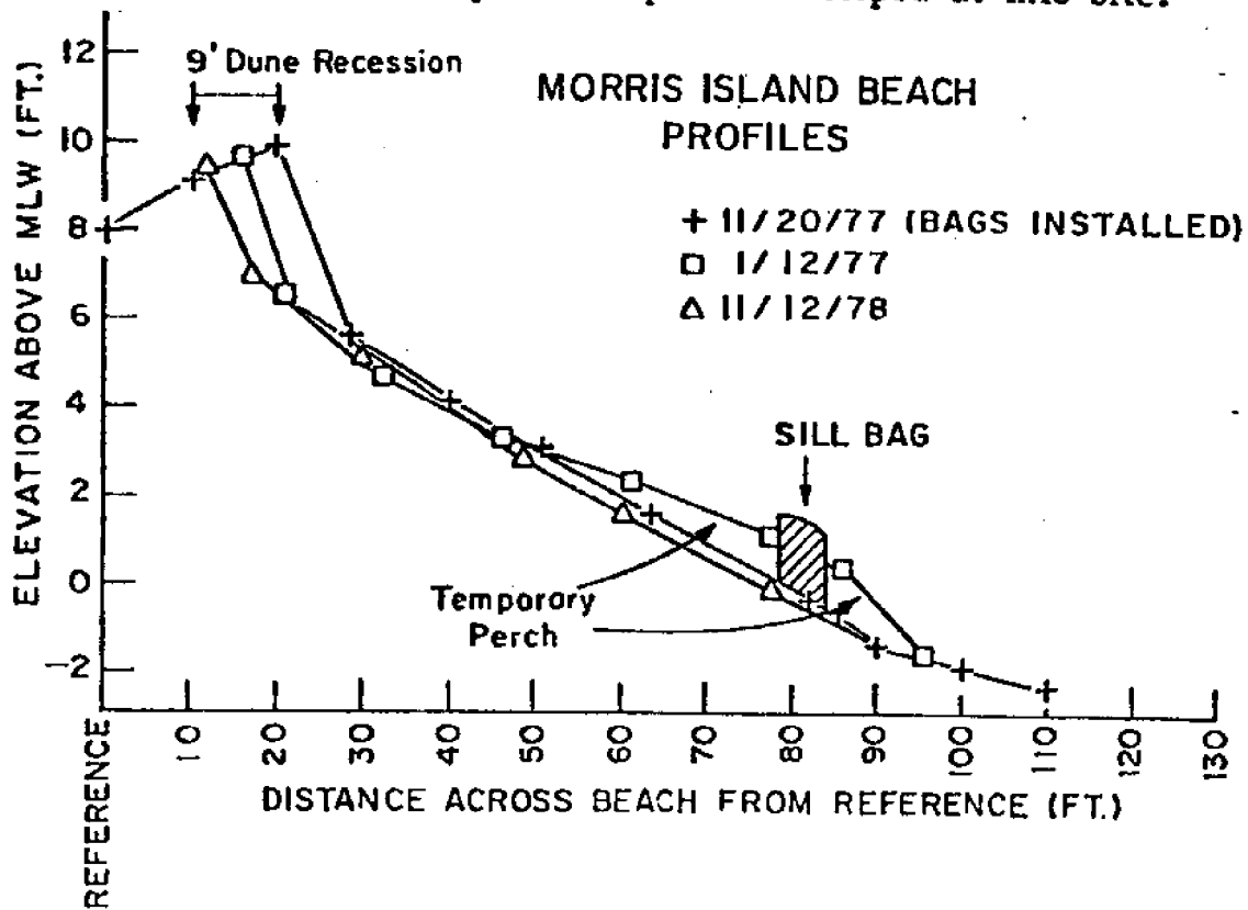
Figure 3. Comparison of beach profiles at Morris Island. This profile runs perpendicular to the beach across the second bag from the bottom
