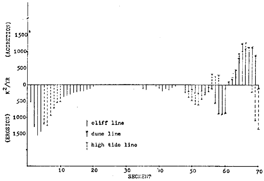
Fig. 3. Annual Change 1939 - 1970. Great Point to Tom Nevers Head.
