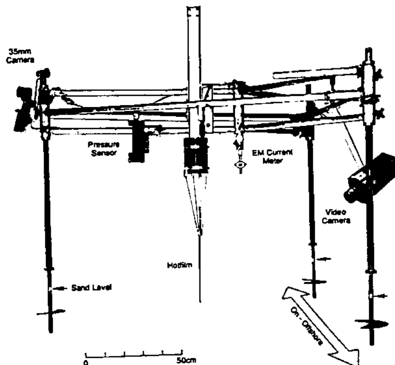
Fig. 1. The surf spider platform used for sensor deployment. The hot film package is mounted on a rack and pinch roller for vertical adjustments in the field.
