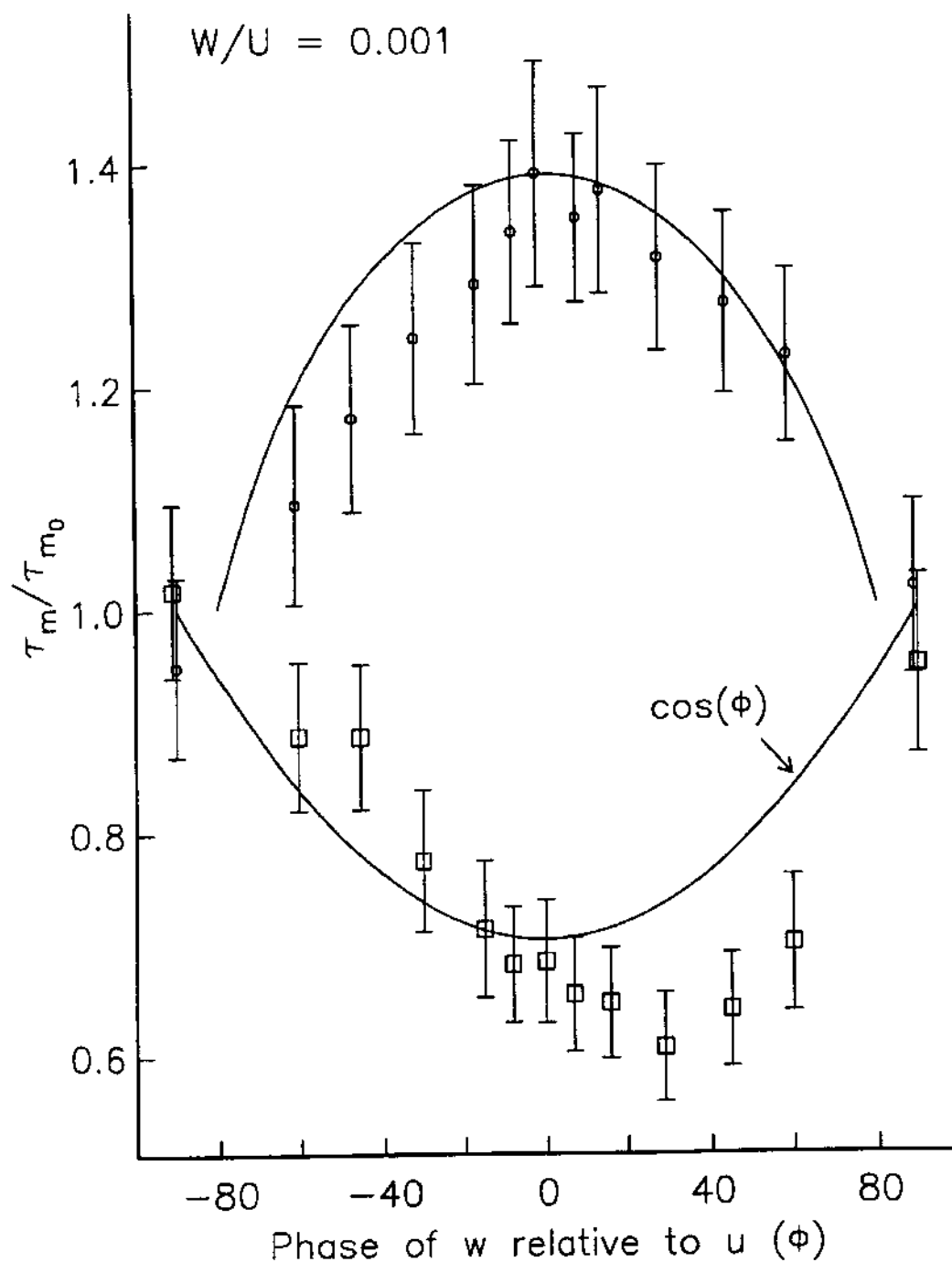
Figure 12: Maximum ventilated bed stress values normalized by maximum unventilated bed stress as a function of ventilation phase \phi . Open circles are for suction, open boxes are for injection. Solid lines are expected response assuming instantaneous response. Brackets represent 95% confidence interval based on variance of ensemble averaged estimate.
