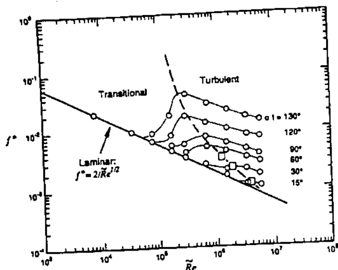
Fig. 8. Temporal friction factor f^* versus Reynolds number Re for constant wave phase \alpha , where 90^\circ corresponds to maximum orbital velocity. The heavy solid line represents laminar Stokes boundary layer, and the heavy dashed line is the limit for fully turbulent flow. Circles are data points. All are from Jensen et al. [1989, Figure 8]. Boxes are points reproduced in our Figure 9.
