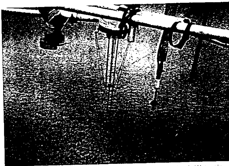
Fig. 6. Photograph of carpet flow under the crest of a wave. Roiled layer is beginning to reorganize and exhibit streamwise periodicity with cross-stream continuity (leg of surf spider in upper right has a diameter of 3.3 cm).
