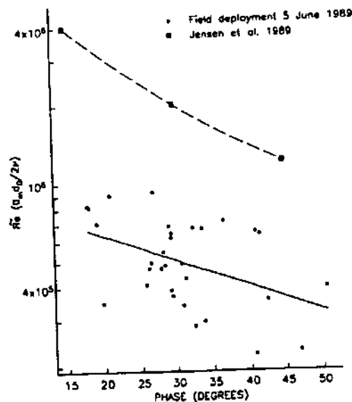
Fig. 9. Wave phase at the onset of roiling versus Re , where a phase of 90^\circ corresponds to maximum orbital velocity. The dashed line represents transition to turbulence from Figure 8. The solid line is a least squares fit of an exponential curve to the values obtained at the onset of roiling.
