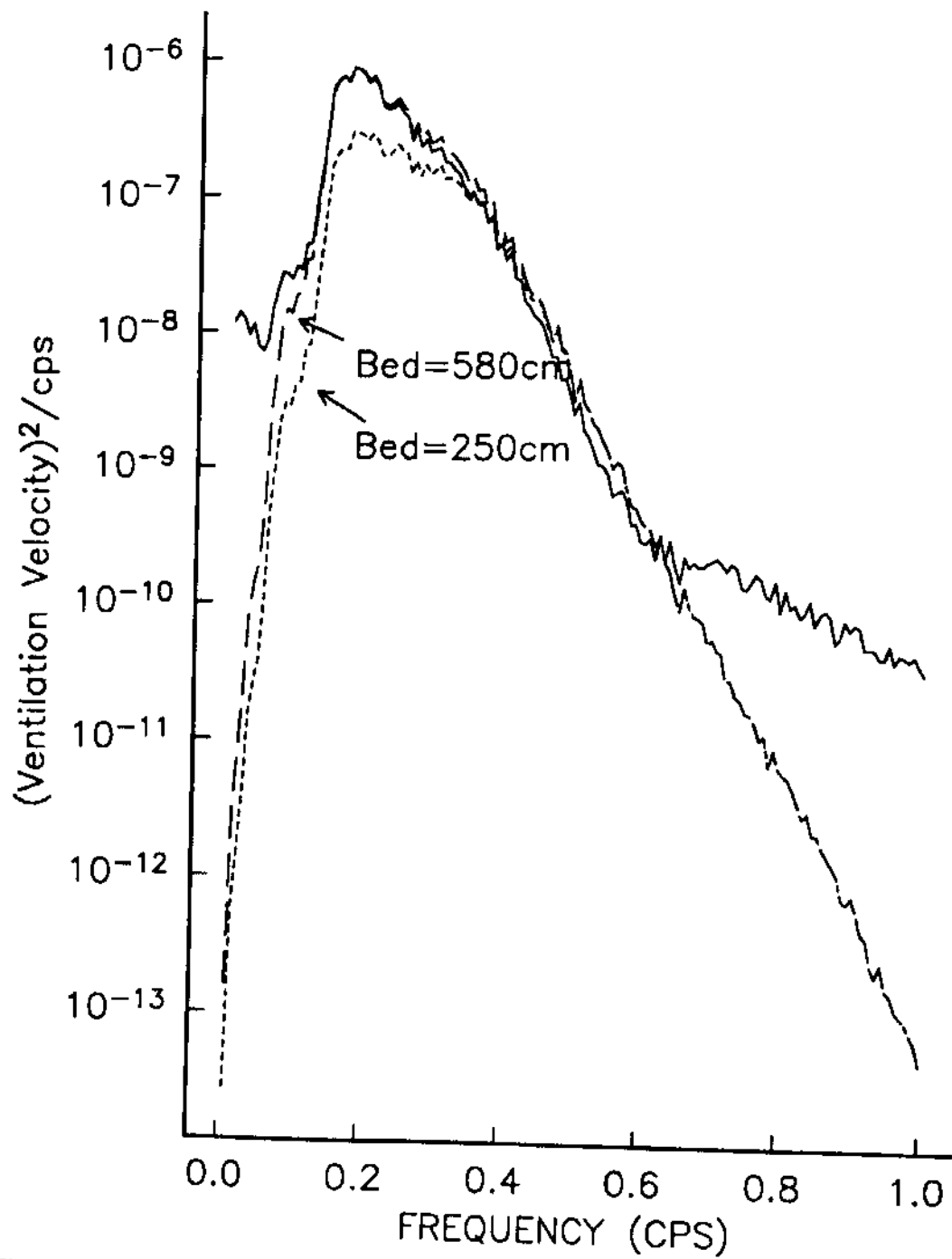
Figure 5: Solid line is ventilation spectra as calculated from differential pressure sensor. Dotted and dashed lines represent ventilation spectra predicted from (11). Dotted line assumes bed thickness of 250 cm and dashed assumes thickness of 580 cm. Units are in (cm/s) 2 /cps.
