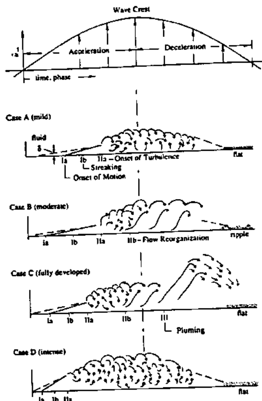
Fig. 12. Schematic drawing of four identifiable sequences in the development of the fluid-granular boundary layer under the crest of near-breaking waves, shown in the order of increasing intensity of motion at the interface. Details of case C are shown in Figure 4.
