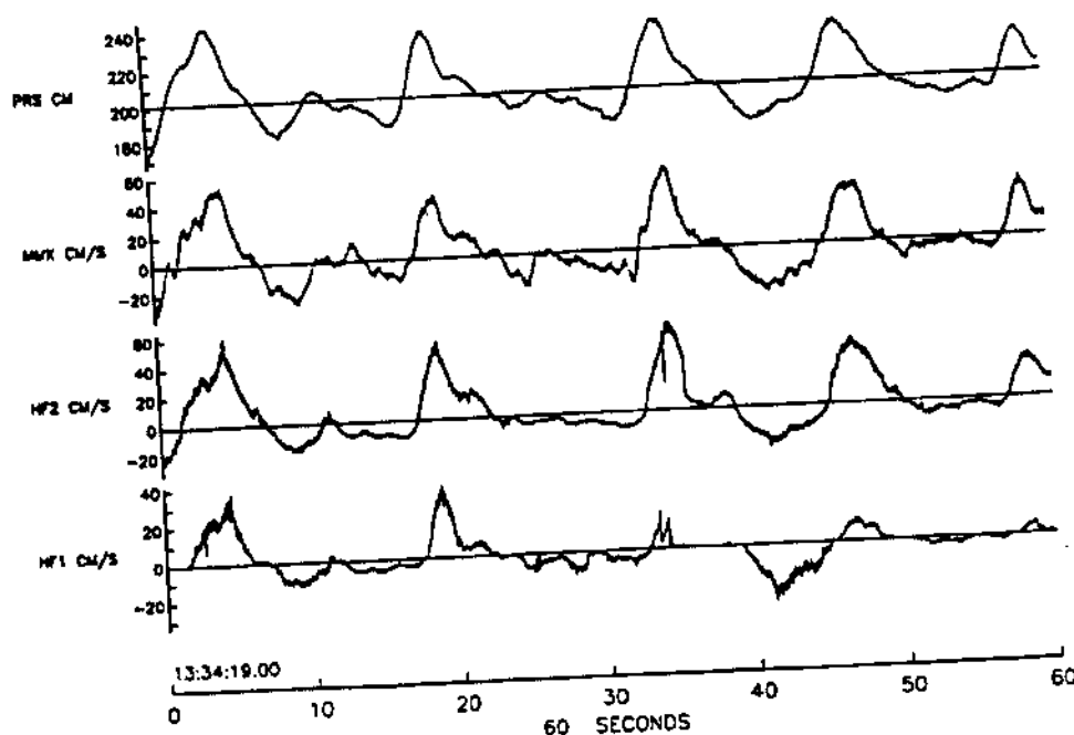
Fig. 2. Typical time series from June 5, 1989, experiment. Sensor outputs (top to bottom) are pressure, mid-depth cross-shore velocity (cm current meter), and bottom velocities (hot films). Hot film probes 1 and 2 were approximately 0.5 cm and 1.5 cm above the "at rest" bed.
