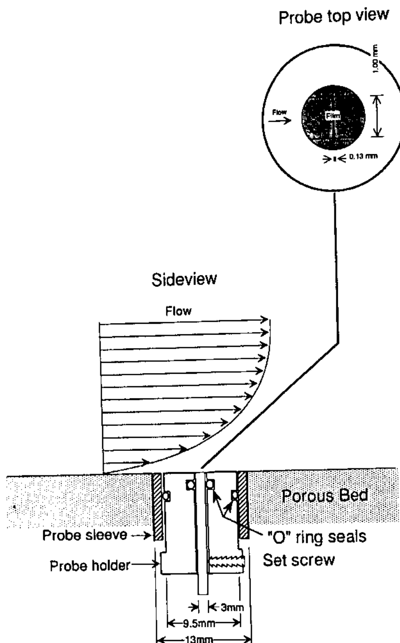
Figure 2: Schematic of the flush mounted hot film shear stress sensor showing emplacement technique. Insert shows face of probe.
