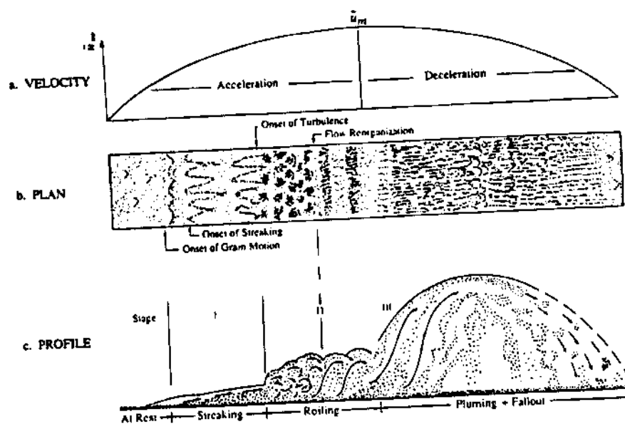
Fig. 4. Schematic illustration of the sequences in the development of the fluid-granular boundary layer for the case of "fully developed" pluming under the crest of a near-breaking wave (case C of Figure 12).
