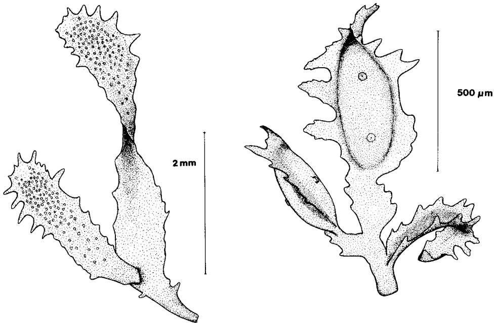
Figs. 2–3. Gelidium rex . Fig. 2. Tetrasporic branchlet. Fig. 3. Cystocarpic branchlet.
