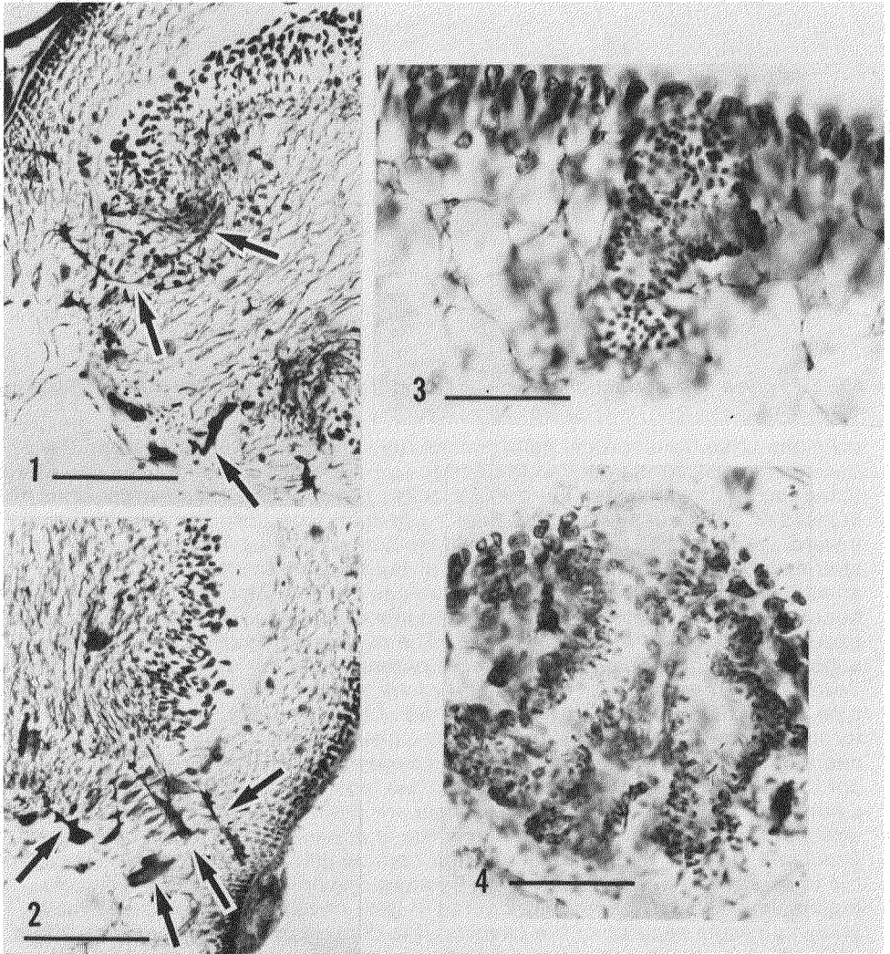
Figs. 1–4. Polycavernosa species. Fig. 1. Median longitudinal section through cystocarp showing basal absorbing filaments (arrowheads) (Doty #32423 from Malaysia, BISH). Fig. 2. Lateral view of basal absorbing filaments (same specimen as Fig. 1, different cystocarp). (Scale bars of both figures = 50 \mu\text{m} .) Fig. 3. Polycavernosa debilis . Developing multiple spermatangial cavities (Belize, US). Fig. 4. Polycavernosa fastigiata . Mature spermatangial caves (Hainan Island, China, AST 80-2335). (Scale bars of both figures = 25 \mu\text{m} .)
