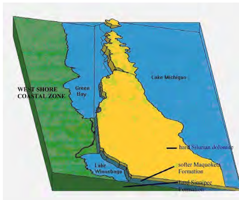
Figure 64: Green Bay post-glacial geology (by Steven Dutch, UWGB). Figure from Rost 2003.
