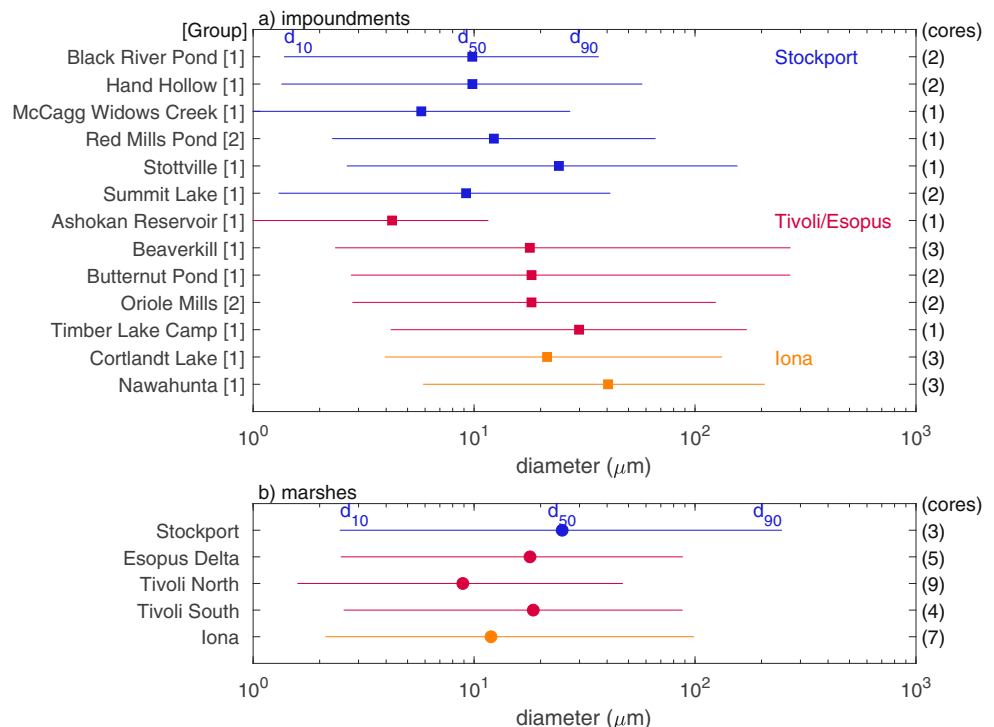
Fig. 6 Particle size distributions from a impoundments and b marshes. Markers show the average d 50 , and lines show d 10 to d 90 . Impoundments are grouped by subwatershed. The impoundment classification group (see the “Methods” section) is in brackets, and the number of cores at each site is in parentheses. Core data are available at https://doi.org/10.7275/dh3v-0x33
