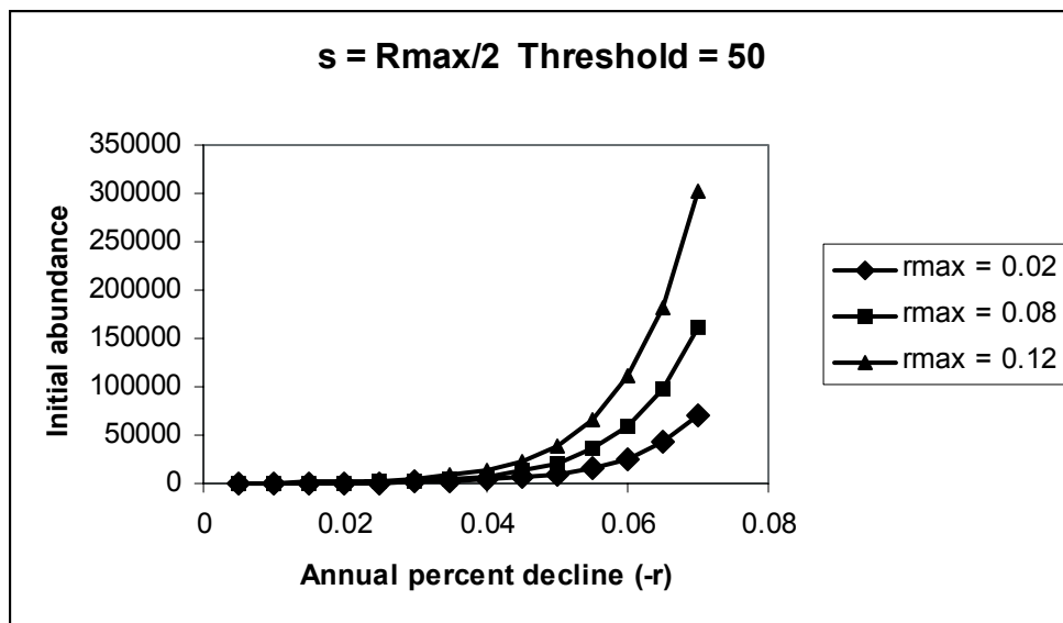
Appendix Figure A4.1a. Initial abundances together with annual percent decline that all result in a 1% chance of reaching an extinction threshold of 50 adults in 100 years assuming that the standard deviation ( s ) is R_{\max}/2 . Any combination of Initial abundance and annual percent decline falling below the appropriate R_{\max} line would qualify for an Endangered listing.
