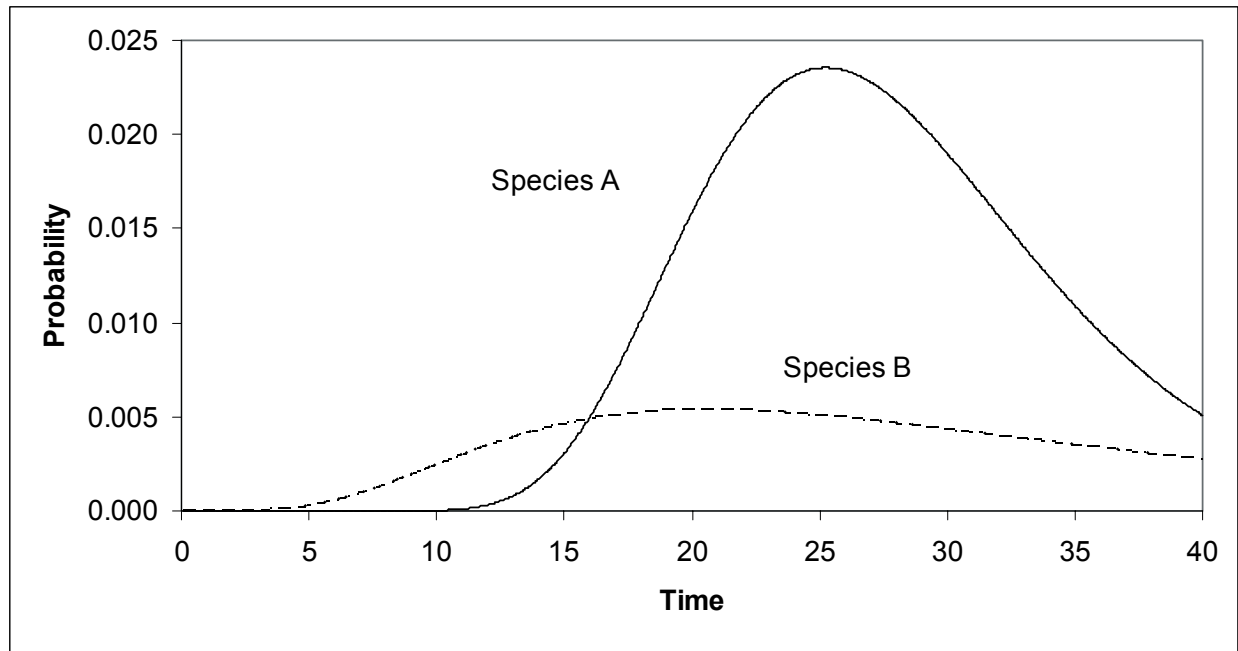
Figure 1. Extinction time probability functions for species A (solid) and species B (dashed).
