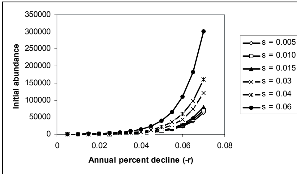
Appendix Figure A4.2a. Initial abundance as a function of annual percent decline for different values of the standard deviation in r ( s ).
