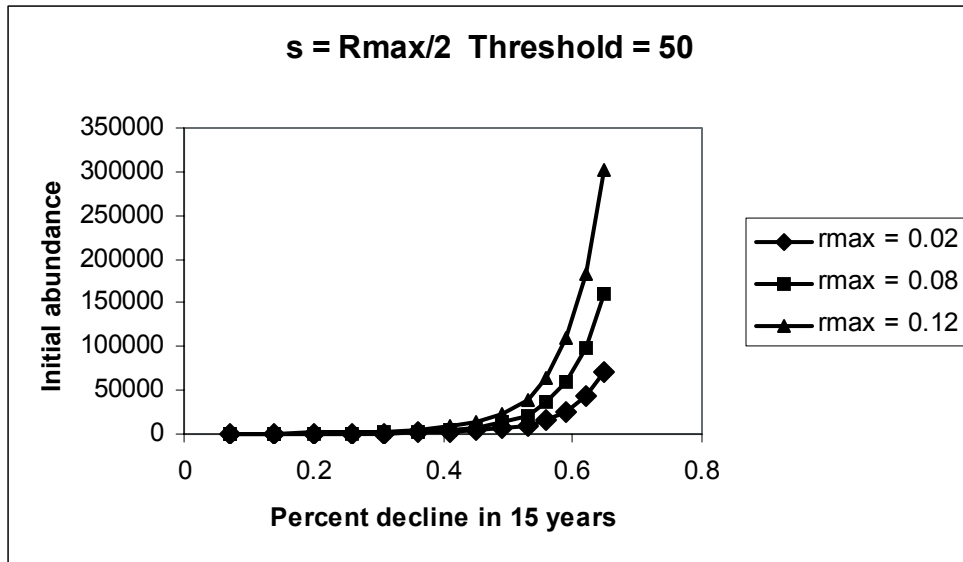
Appendix Figure A4.3a. Given the same threshold for extinction (50) and standard deviation in growth rate ( s = R_{max}/2 ), different EN criteria contours are shown for different R_{max} values. An EN listing would be warranted for cases that fell below the appropriate contour.
