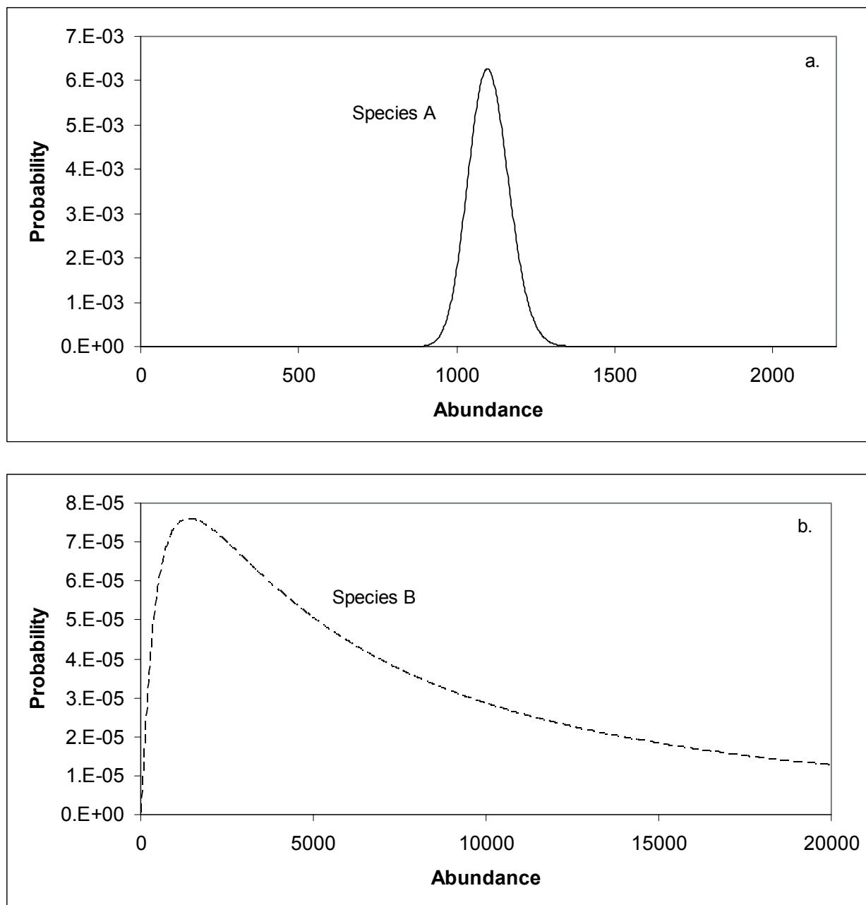
Appendix Figure A3.3. Abundance probability functions. Appendix Figure A3.3a (top): Abundance probability function for Species A. Figure A3.3b (bottom): Abundance probability function for Species B. Note that the scales on the axes differ between the two panels.
