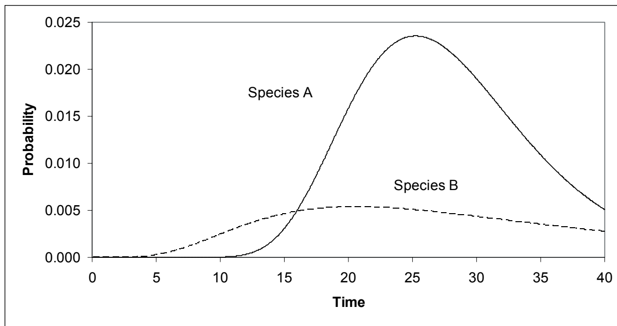
Appendix Figure A3.4. Extinction time probability functions for Species A (solid) and Species B (dashed), adjusted to reflect the uncertainty in abundance shown in Appendix Figures A3.3a and 3b.
