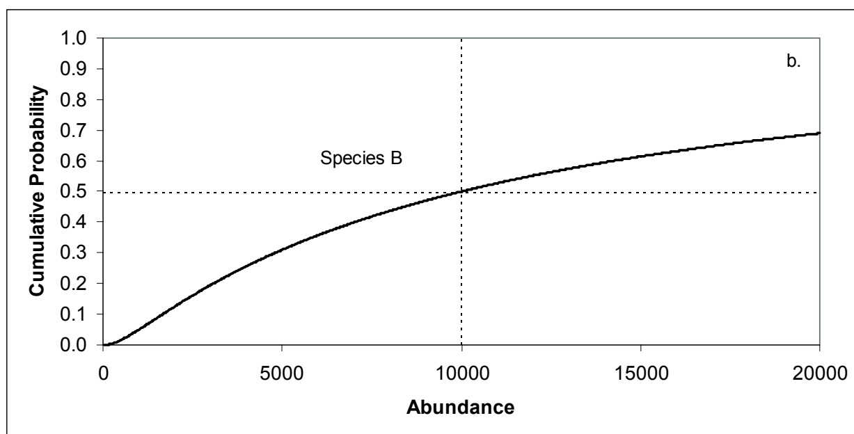
Appendix Figure A3.6. Cumulative probability of abundance. Appendix Figure 6a (top): Cumulative abundance probability for Species A. Figure A3.6b (bottom): Cumulative abundance probability for Species B. Note that the scales on the axes differ between the two panels.
