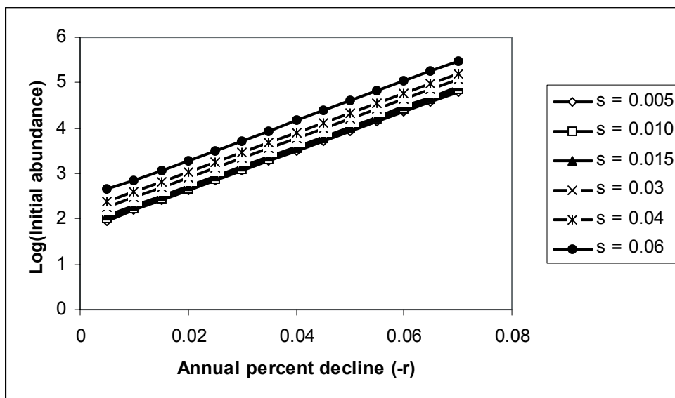
Appendix Figure A4.2b. As in Appendix Figure A4.2a with the log of initial abundance.
