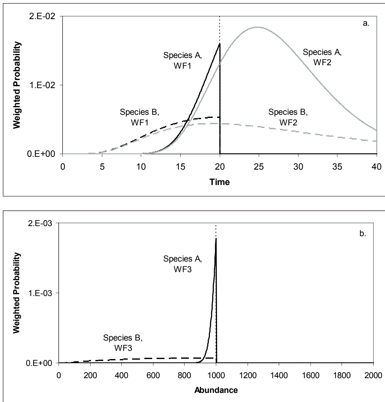
Appendix Figure A3.8. Definitions of extinction risk for three approaches. For each approach and species, the area under the curve is the extinction risk. Appendix Figure A3.8a (top): Traditional (black solid; black dashed) and comprehensive (grey solid, gray dashed) approaches. Appendix Figure A3.8b (bottom): Threshold approach.
