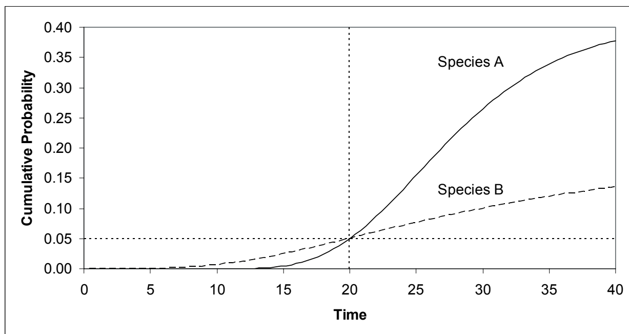
Appendix Figure A3.5. Cumulative probability of extinction as a function of time for Species A (solid) and Species B (dashed).
