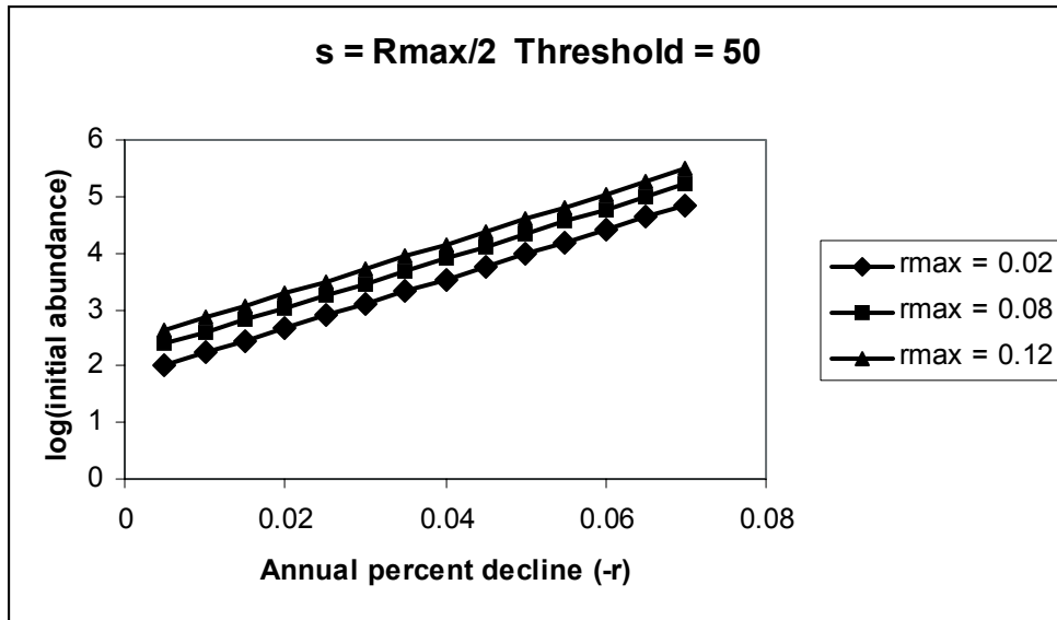
Appendix Figure A4.1b. The same data presented in Figure A4.1a with abundance on a log scale.
