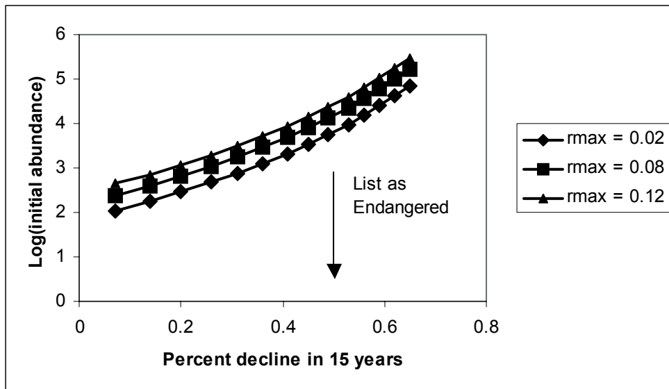
Appendix Figure A4.3b. As in Appendix Figure A4.2a with the log of initial abundance.
