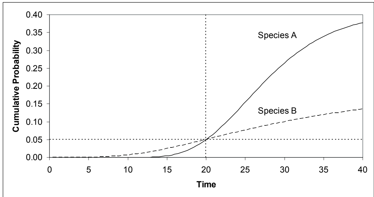
Figure 2. Cumulative probability of extinction as a function of time for species A (solid) and species B (dashed).
