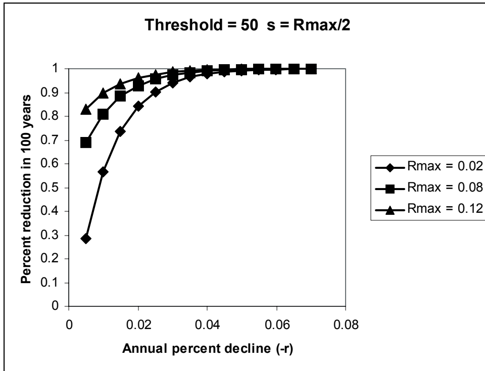
Appendix Figure A4.4. The percent reduction in 100 years for different annual rates of decline and for different levels of variability in growth rate.
