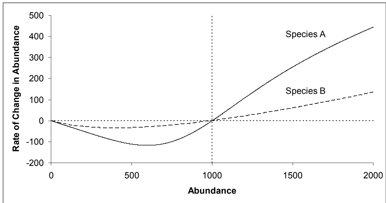
Appendix Figure A3.1. Rates of change in abundance for Species A (solid) and Species B (dashed). A depensatory threshold at 1000 individuals exists for both Species. Below the depensatory threshold, the expected rate of change is negative.
