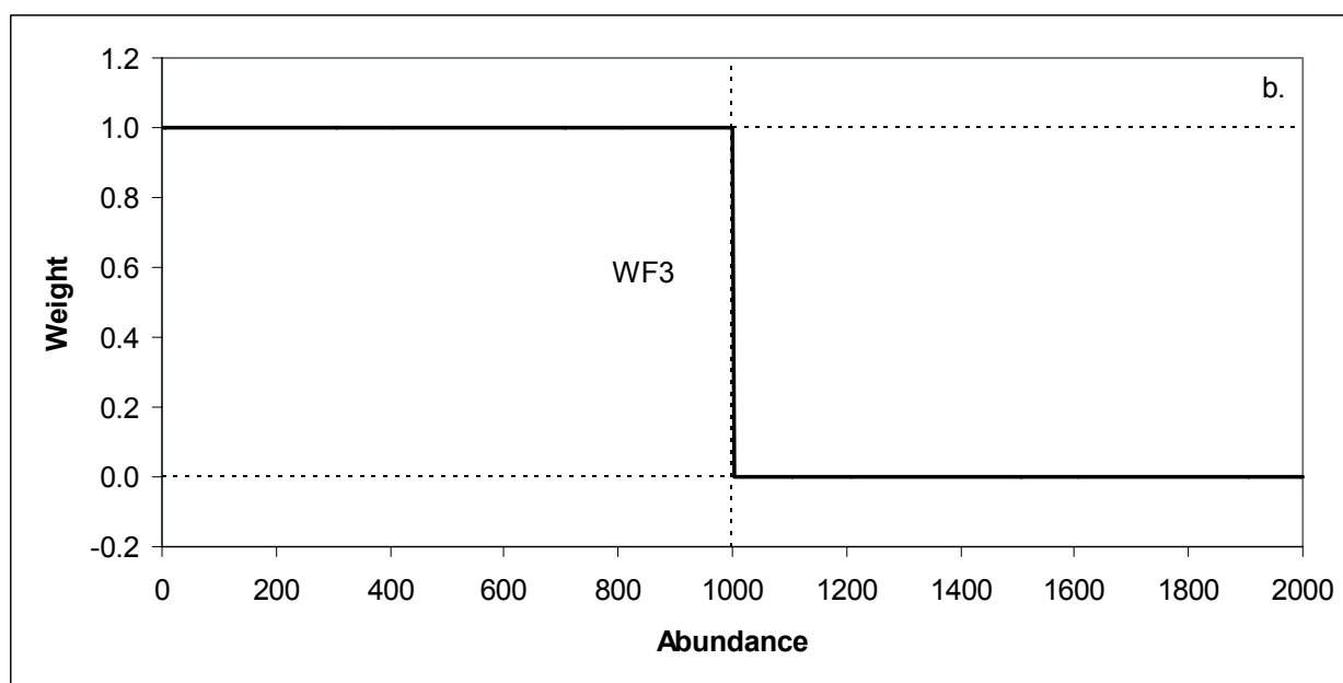
Appendix Figure A3.7. Weighting functions. Appendix Figure A3.7a (top): Two weighting functions with extinction time as the variable. Figure A3.7b (bottom): A weighting function with abundance as the variable.
