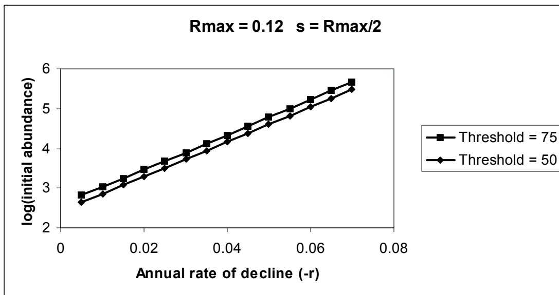
Appendix Figure A4.5b. As in Appendix Figure A4.3a with the log of initial abundance.
