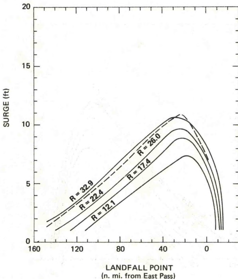
Figure 13.--Same as figure 11 but for Lower Anchorage (point 6). Dashed curve from figure 6.
