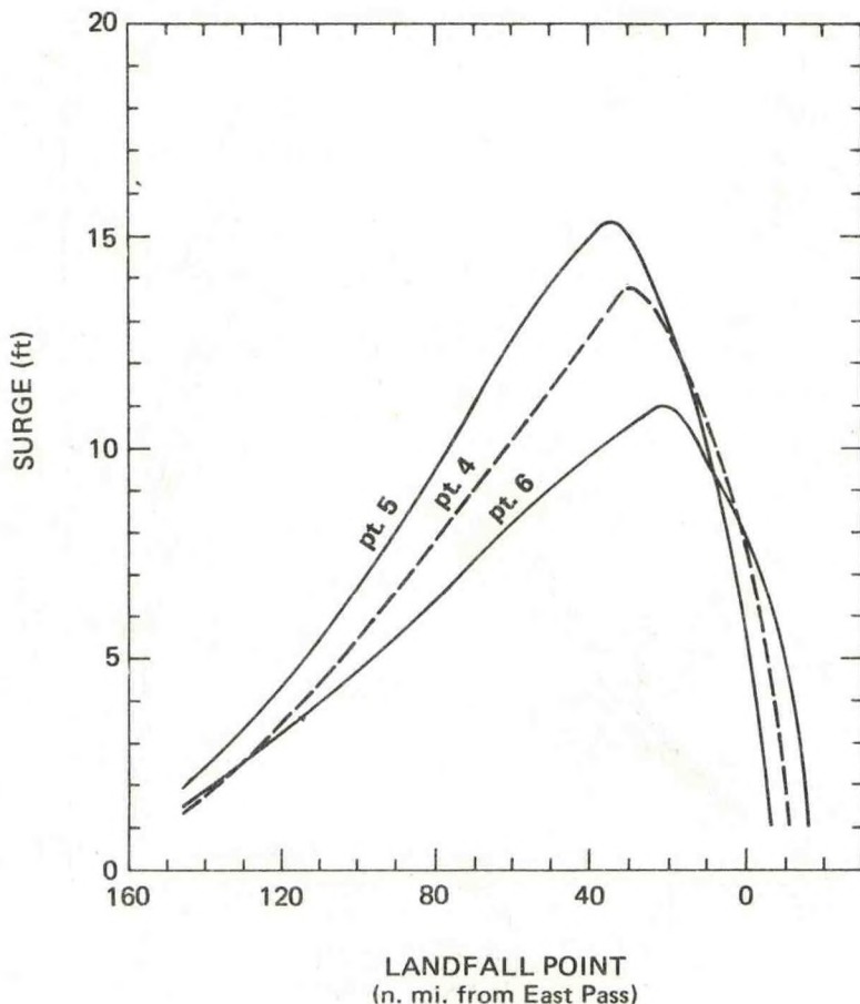
Figure 6.--Same as figure 5 for selected locations inside Apalachicola Bay: Apalachicola (point 4), St. Vincent Sound (point 5), and near Lower Anchorage (point 6).
