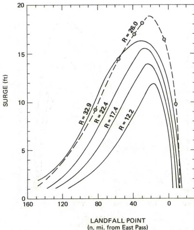
Figure 10.--Maximum surge height at East Pass vs. landfall point and R. Dashed curve for R = 26 n.mi. from figure 5. Hurricanes "standard" except for landfall point and R.
