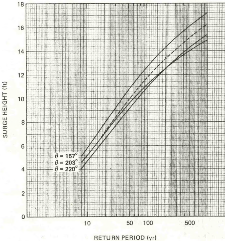
Figure 14.--Surge frequency curves at East Pass for three directions of storm motion (solid lines) and the combined surge frequency curve (dashed line). See text.
