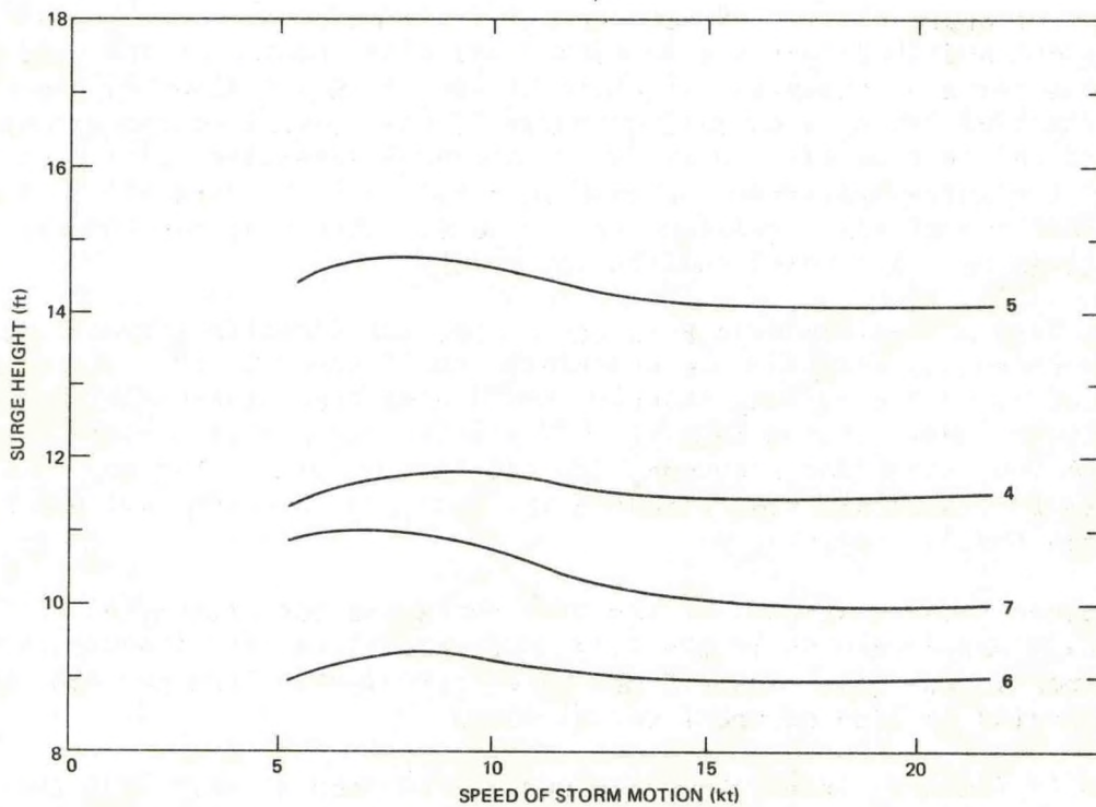
Figure 9.--Variation of surge height with respect to forward speed. Hurricanes "standard" except for forward speed. Upper: for locations 1, 2, 3, and 8. Lower: for locations 4, 5, 7, and 6.
