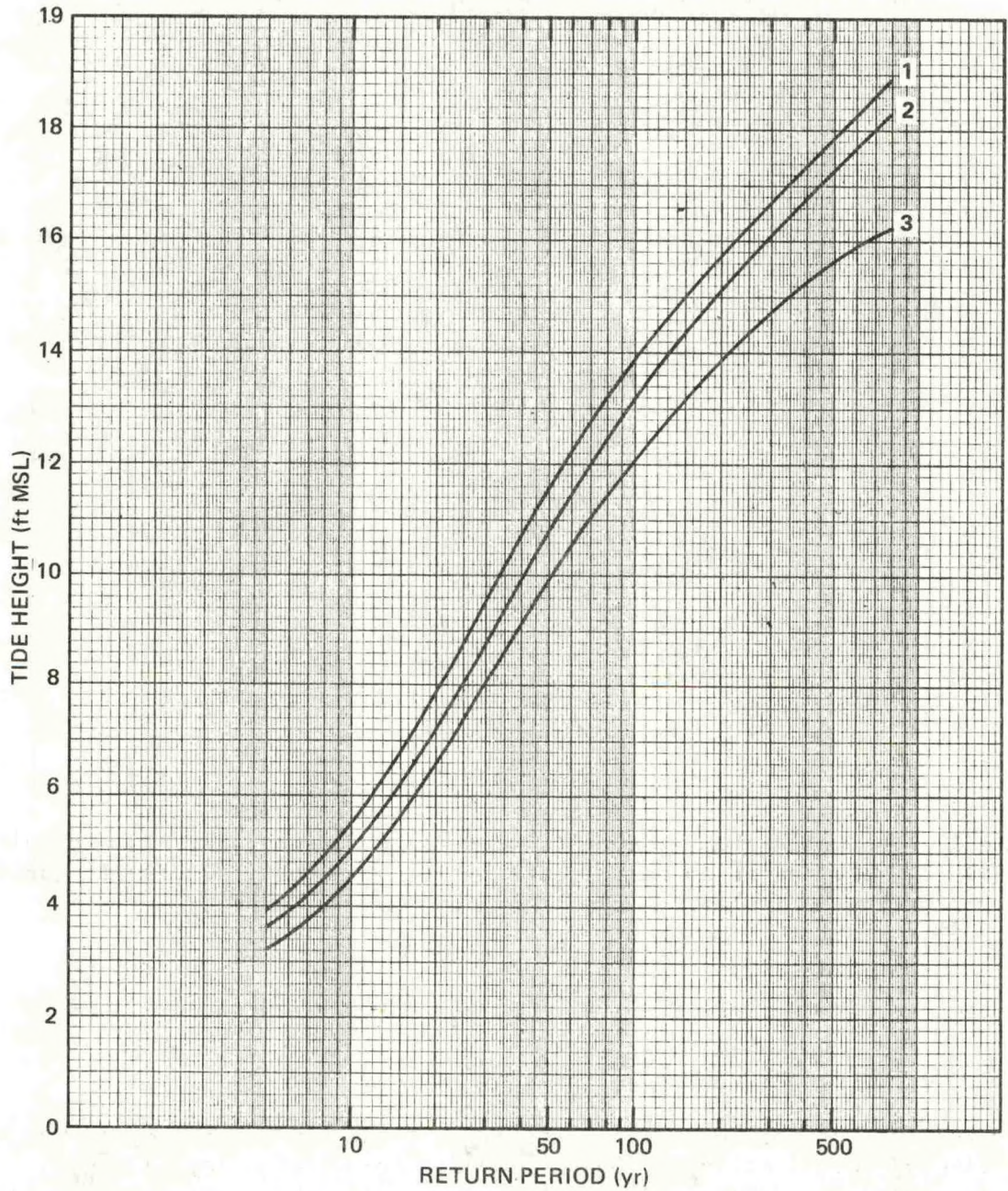
Figure 18.--Total tide frequency curves on the bay shore between Carrabelle and Cat Point, Franklin County, Fla. Datum is local MSL, 1949-51 epoch. See par. 3.6.1 for conversion to National Geodetic Vertical Datum of 1929. Points 1, 2, 3 identified in figure 4.
