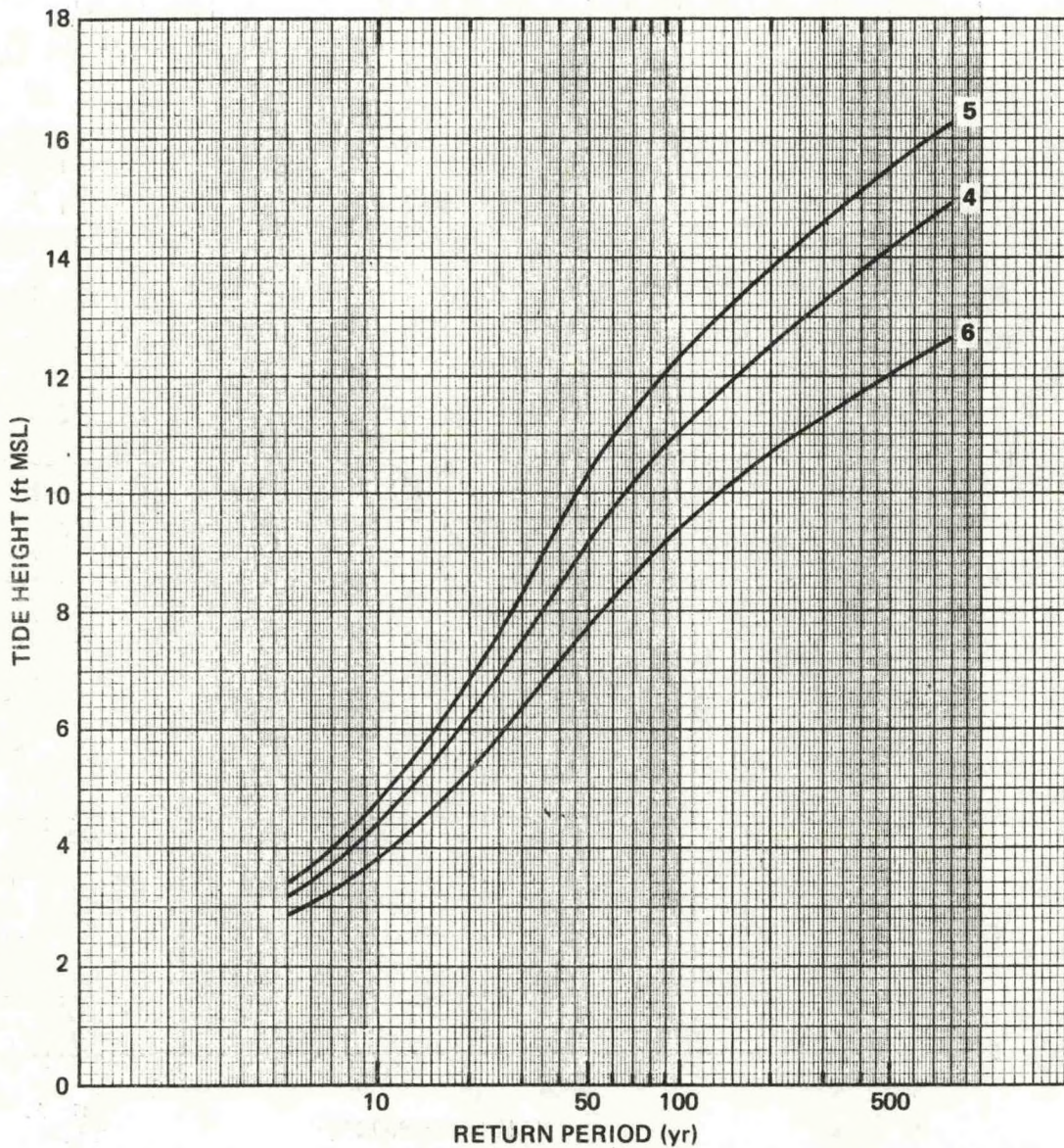
Figure 19.--Same as figure 18 but for locations inside Apalachicola Bay.
