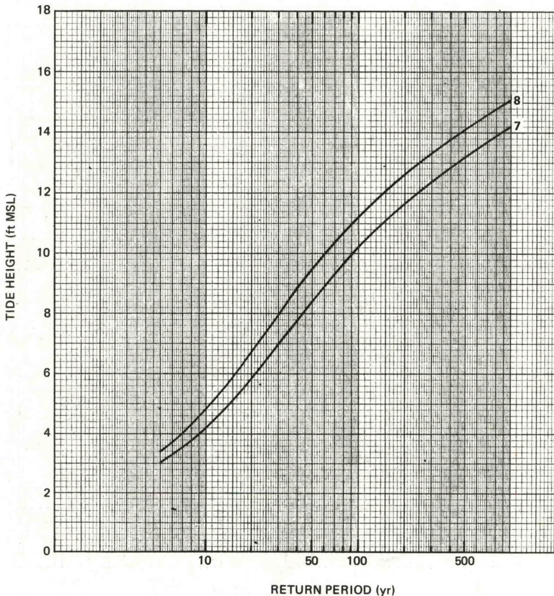
Figure 20.--Same as figure 18 but for locations inside East Bay.
