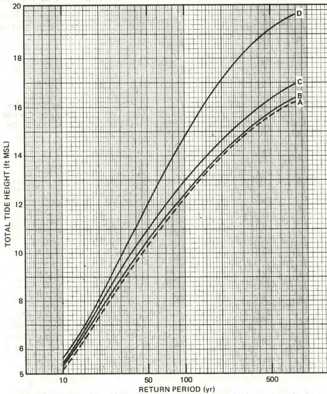
Figure 4.--Total tide frequency curves for the open coast of Franklin County, Fla., at selected locations: (A) Indian Pass, (B) St. George Island (south of Apalachicola), (C) East Pass, and (D) Ochlockonee Point. Locations in figure 2.
