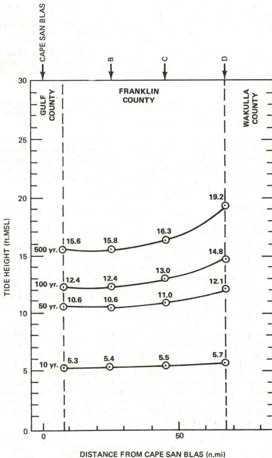
Figure 3.--Tide frequency profiles along open coast of Franklin County (open coast defined in section 2). Datum reference is local MSL, 1941-59 epoch. For differences from National Geodetic Vertical Datum of 1929 see par. 3.6.1.
