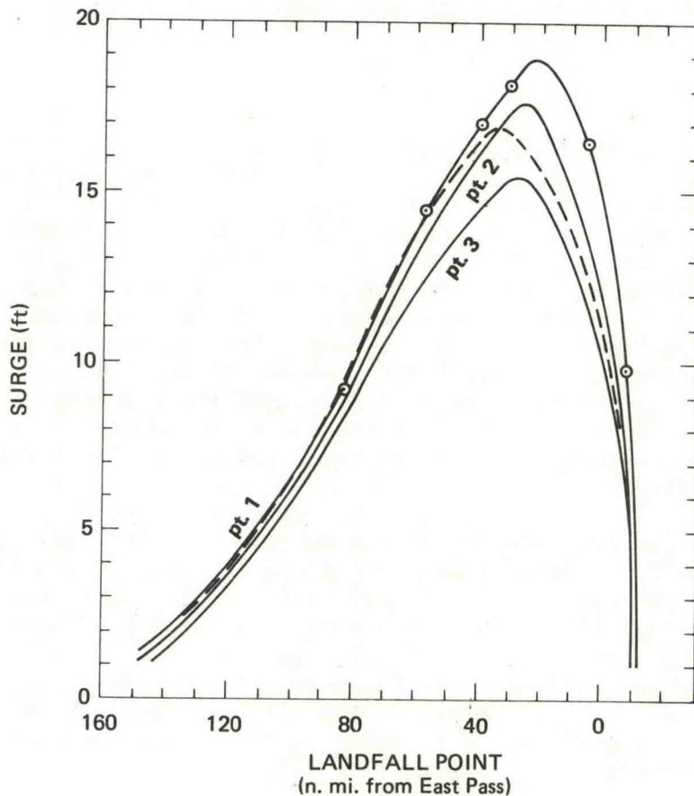
Figure 5.--Maximum surge height vs. storm landfall point at East Pass (dashed curve) and selected locations inside St. George Sound: Carrabelle (point 1), Cat Point (point 3), and about midway between (point 2). Hurricanes "standard" except for landfall point.
