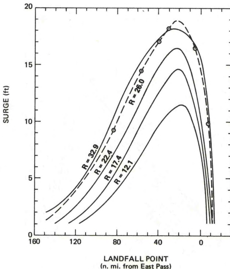
Figure 11.--Maximum surge height at Carrabelle (point 1) vs. storm landfall point and R . Same D , \theta , and f as figure 10. Dashed curve for R = 26 n.mi. from figure 5.
