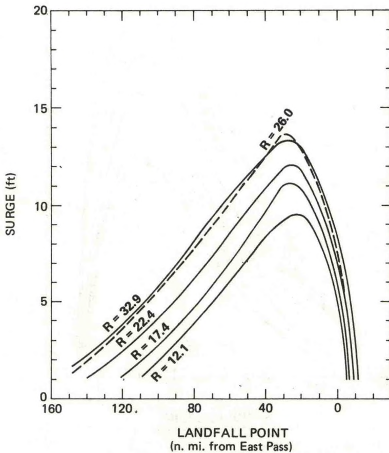
Figure 12.--Same as figure 11 but for Apalachicola (point 4). Dashed curve from figure 6.
