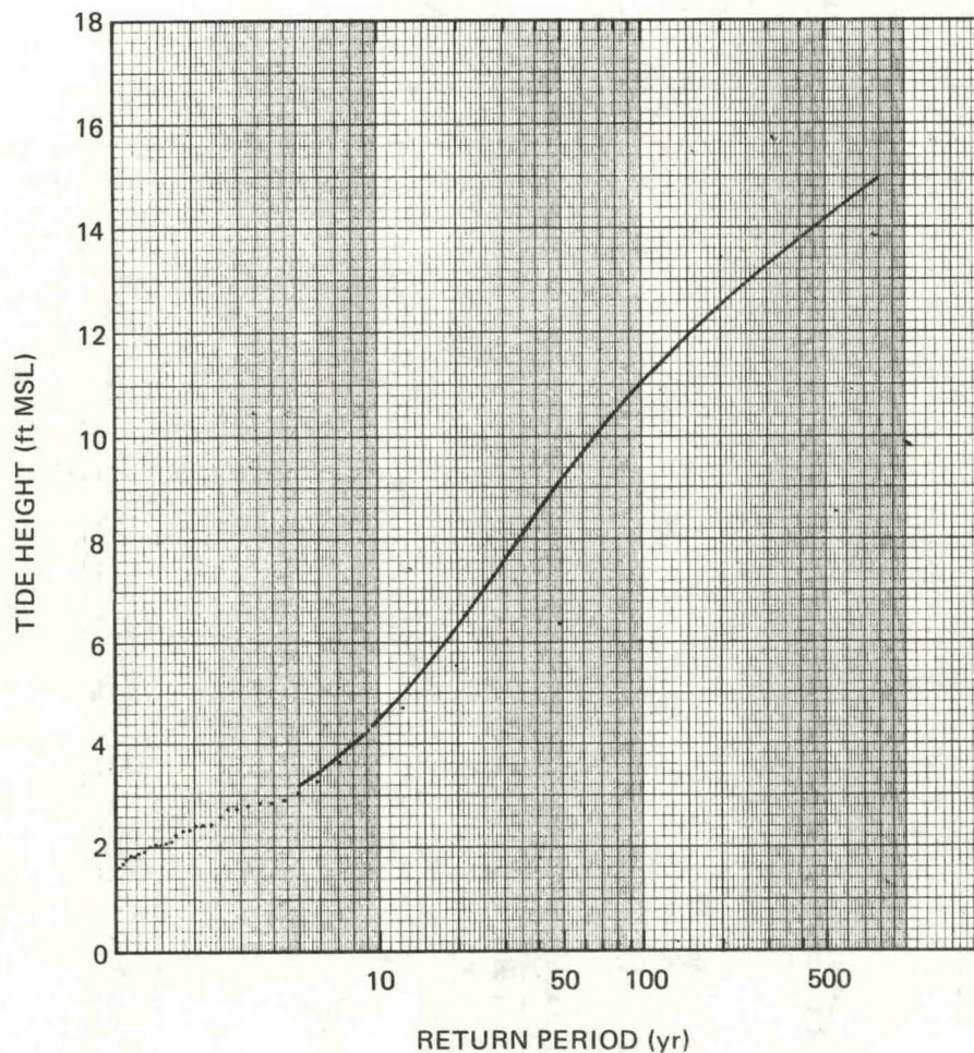
Figure 17.--Annual highest tides at Corps of Engineers gage, Apalachicola (1941-73), plotted as an annual series with adopted total tide frequency curve for Apalachicola.
