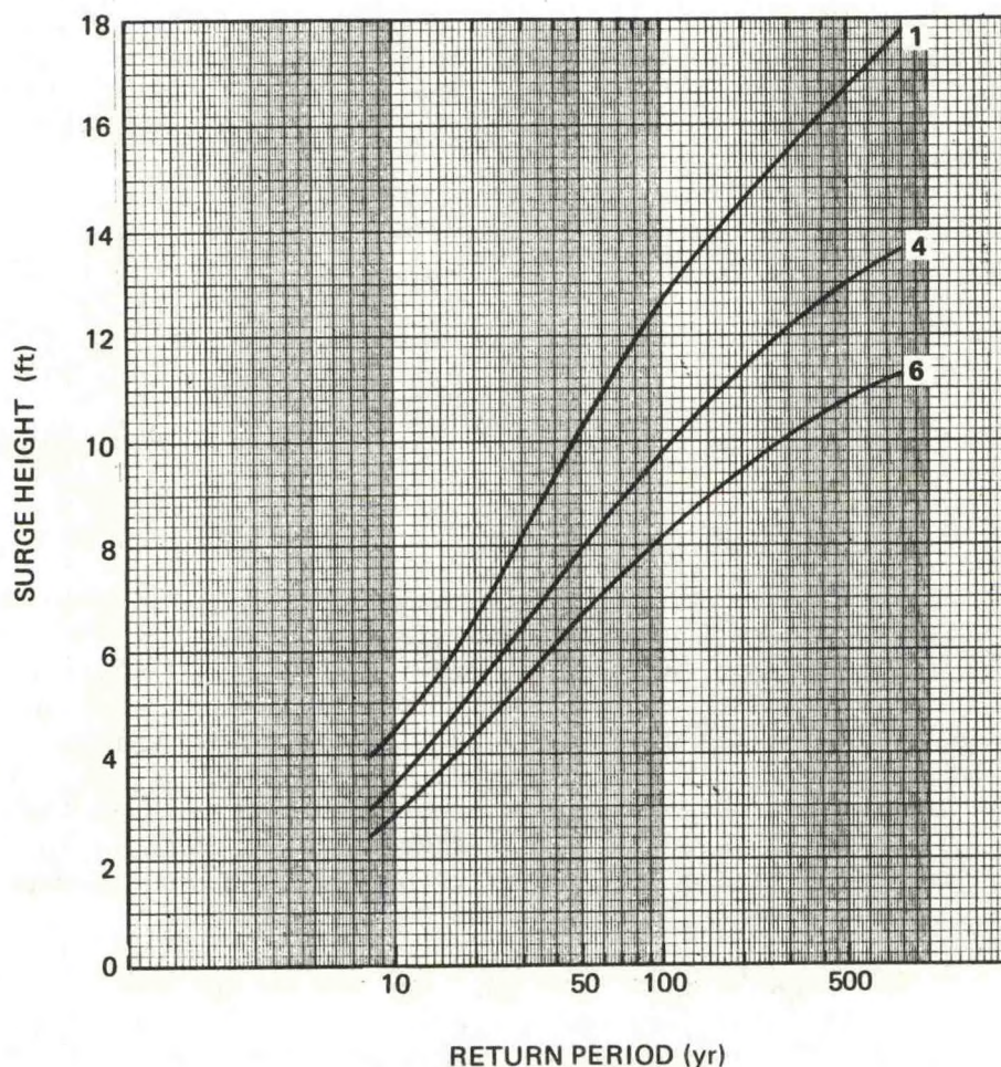
Figure 15.--Surge frequency curves for selected locations: Carrabelle (1), Apalachicola (4) and Lower Anchorage (6).
