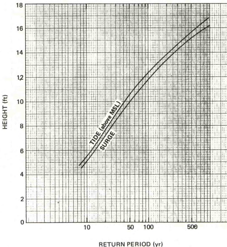
Figure 16.--Surge and tide frequency curves for East Pass.
