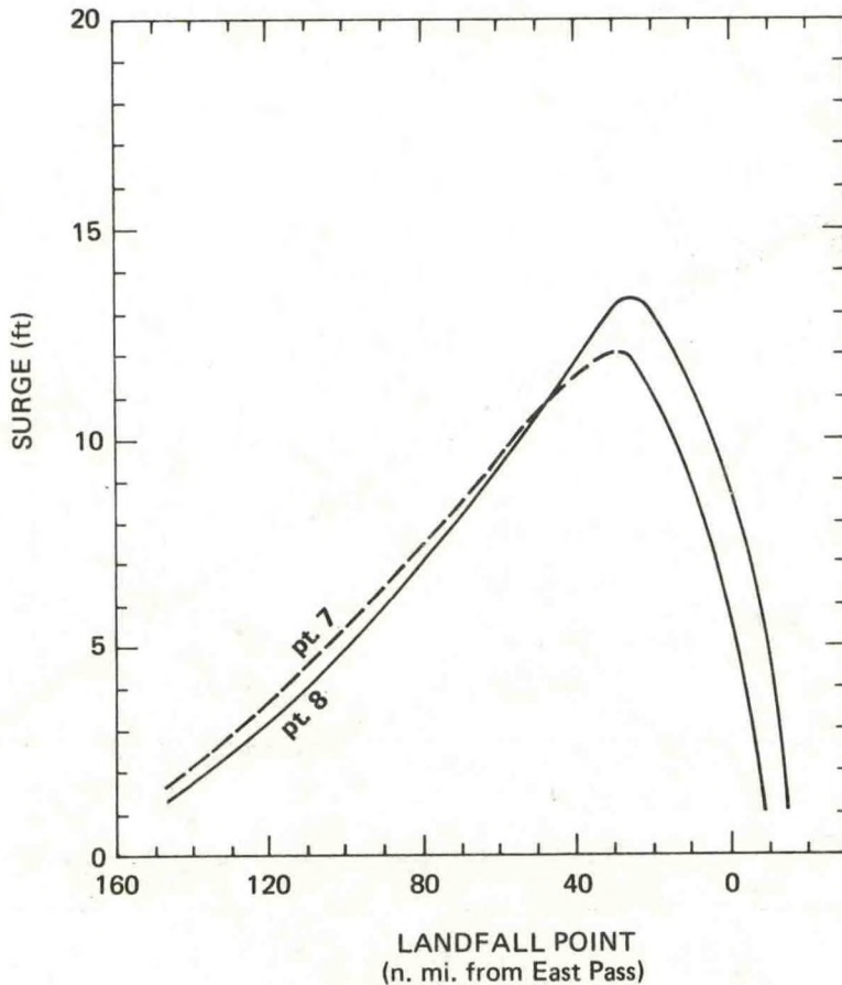
Figure 7.--Same as figure 5 for selected locations in East Bay.
