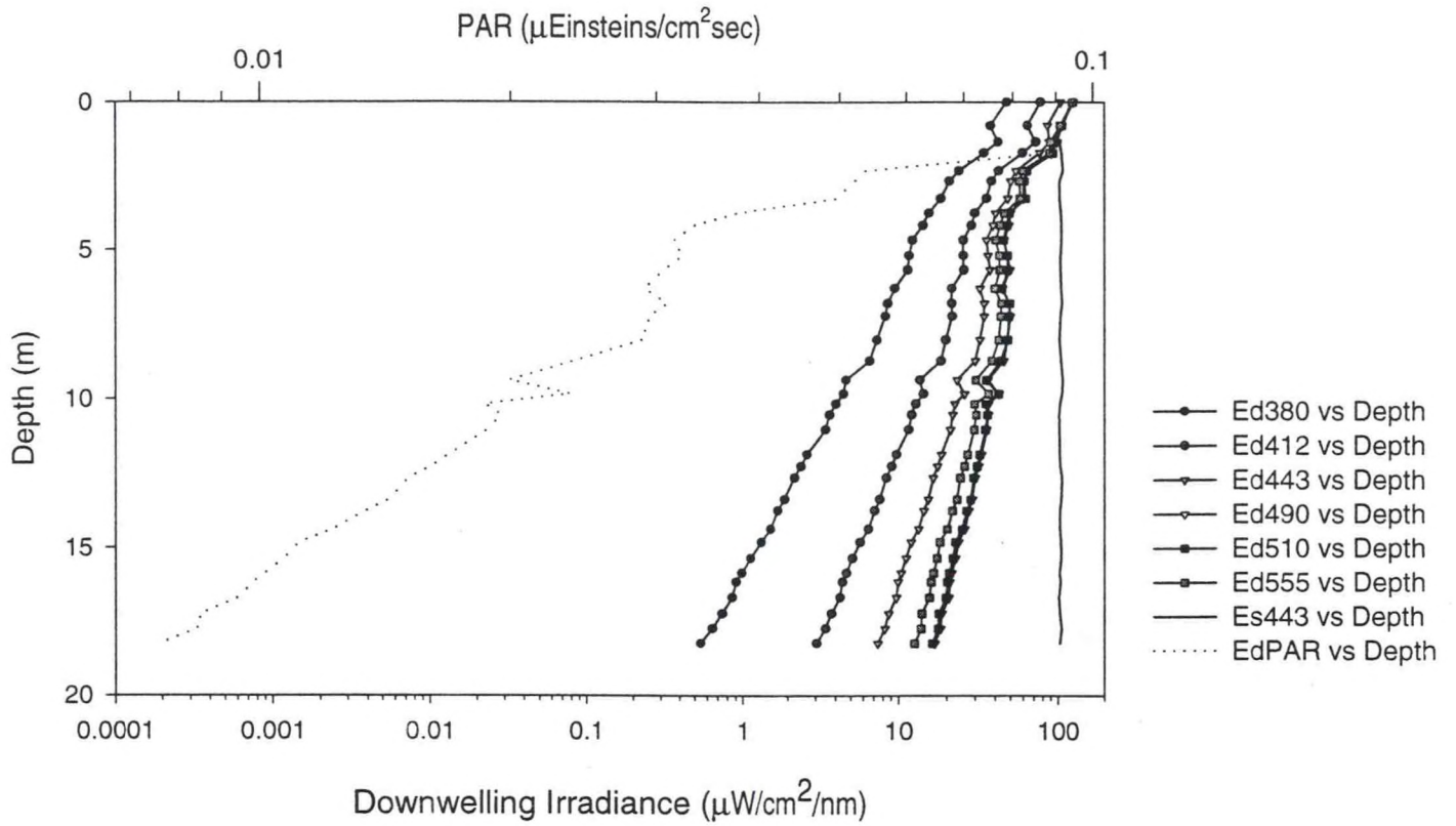
Figure A.1.a - Station 7 Downcast
