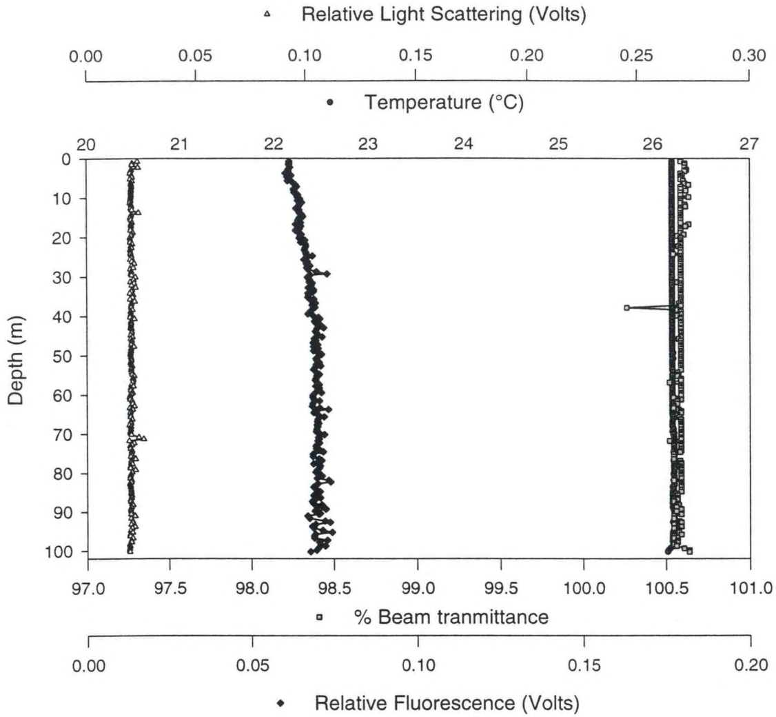
Figure A.8.b - Station 13 Upcast
