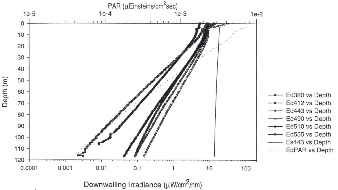
Figure A.11.a - Station 16 Downcast
