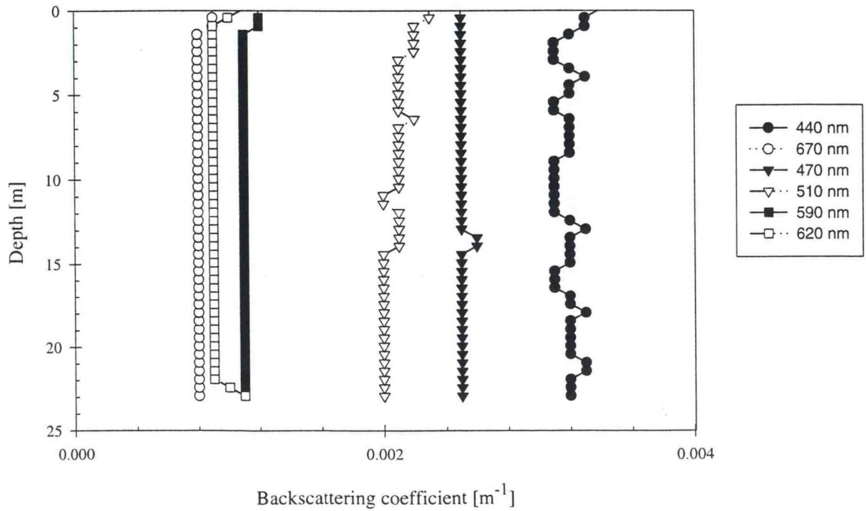
Figure E.6.b - Station 15 Upcast
