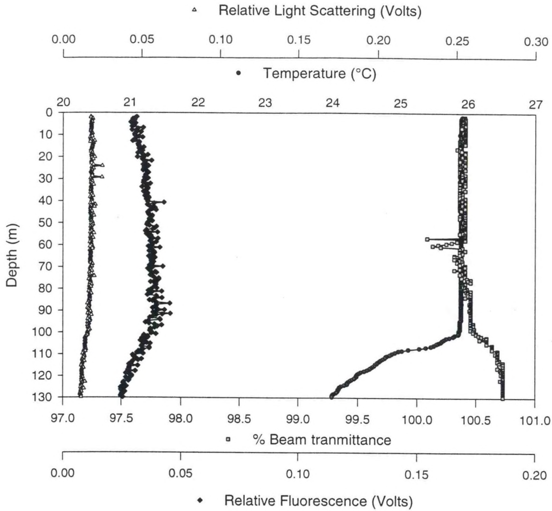
Figure A.9.b - Station 14 Downcast
