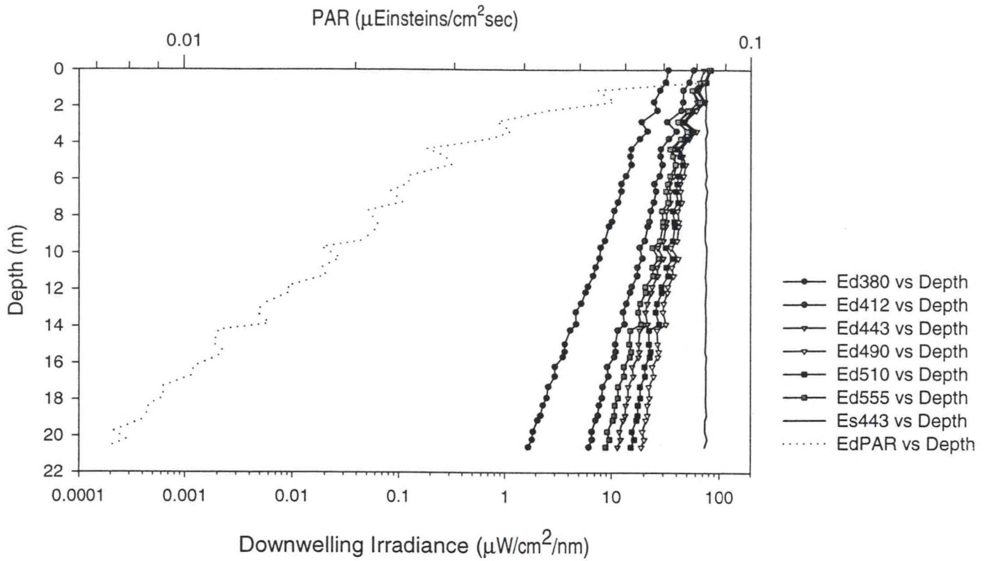
Figure A.4.a - Station 8 Upcast
