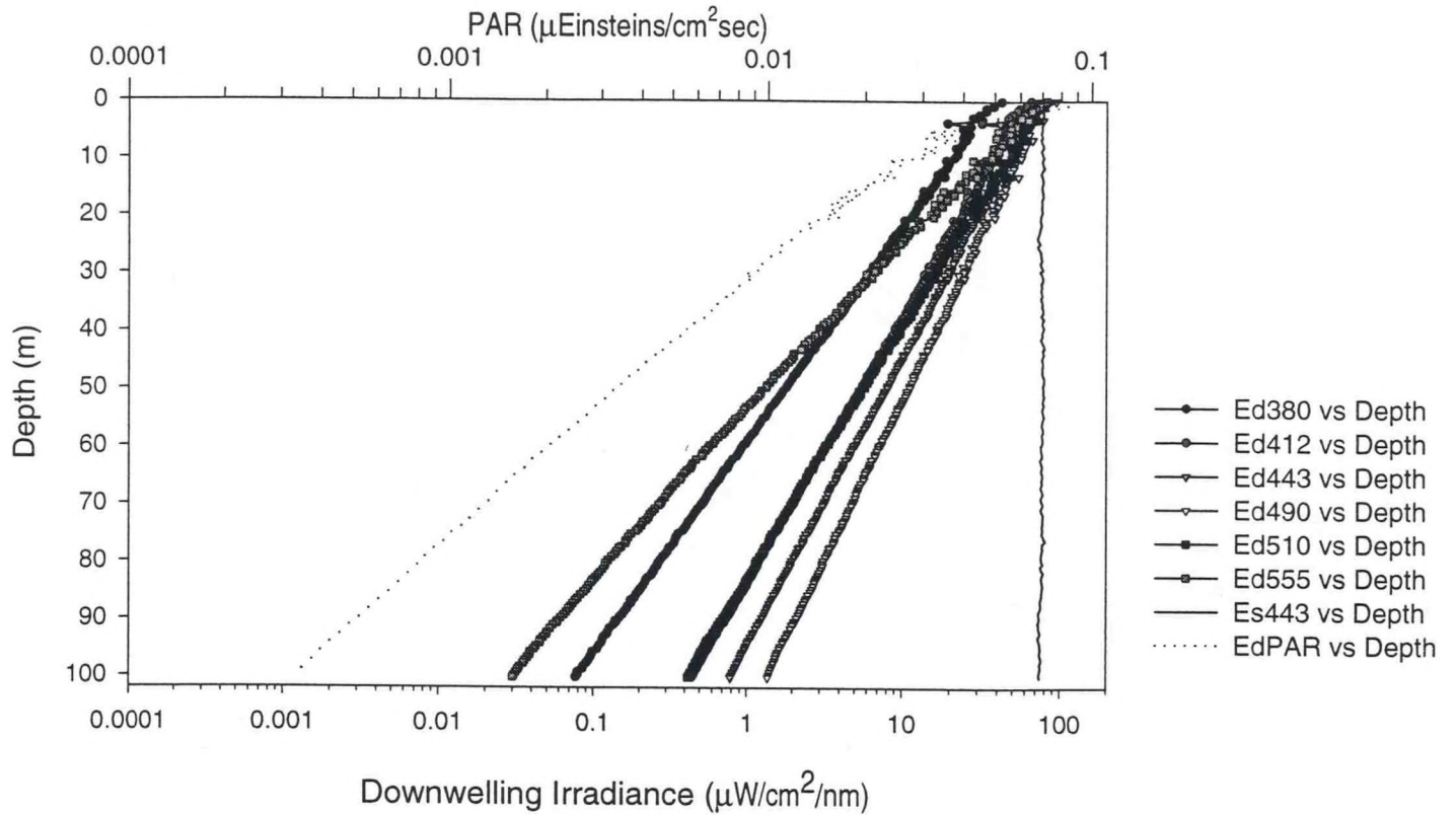
Figure A.8.a - Station 13 Upcast
