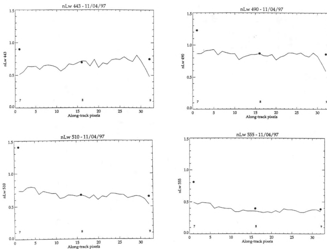
Figure 7. Comparison of in-situ and SeaWiFS derived normalized water leaving radiance
