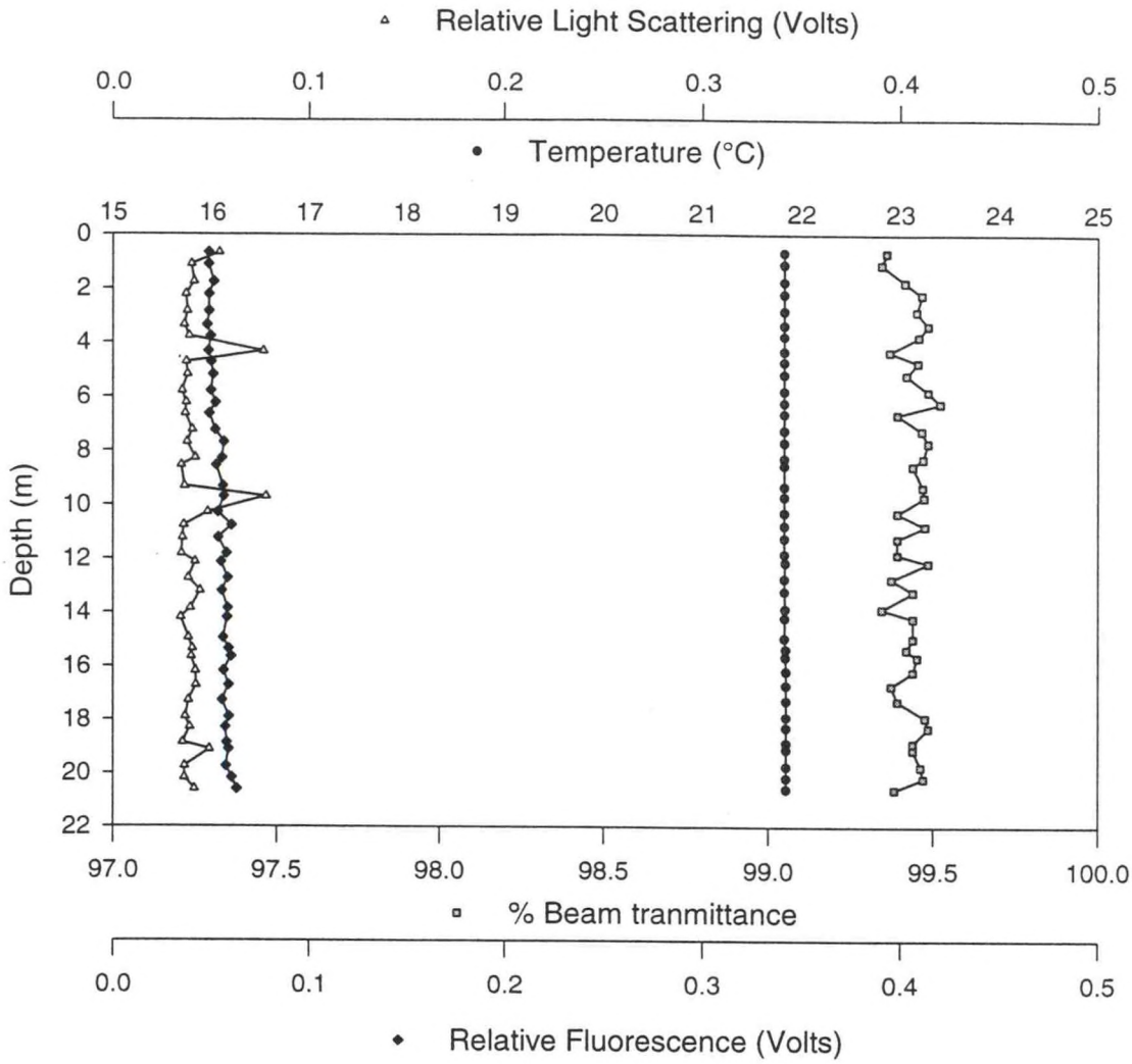
Figure A.4.b - Station 8 Upcast
