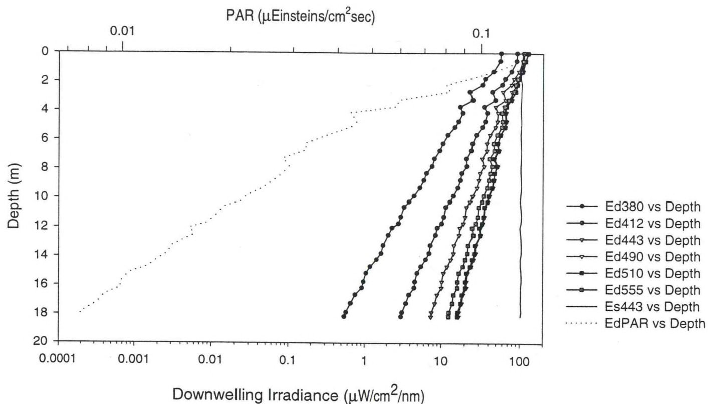
Figure A.2.a - Station 7 Upcast
