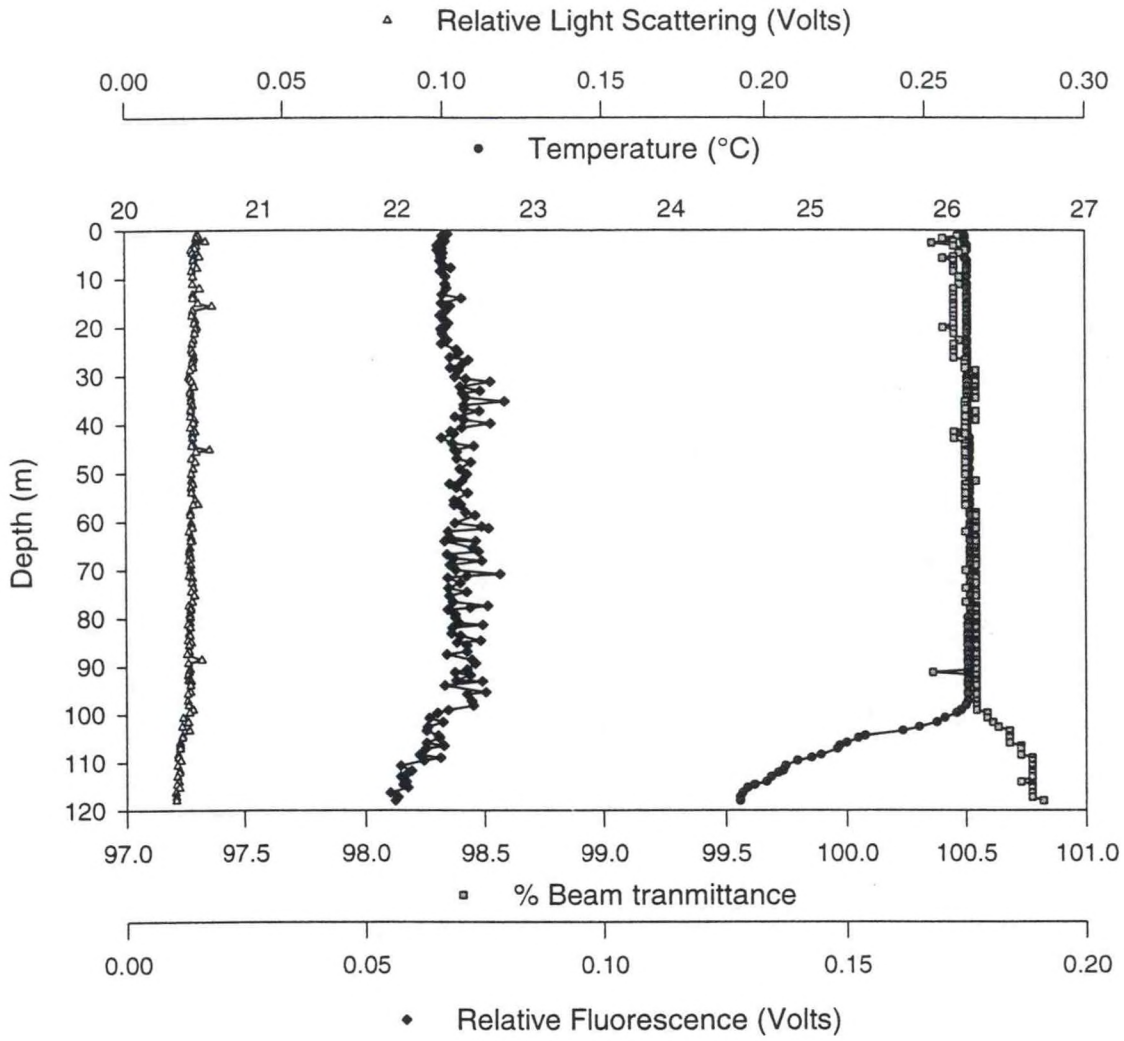
Figure A.12.b - Station 16 Upcast
