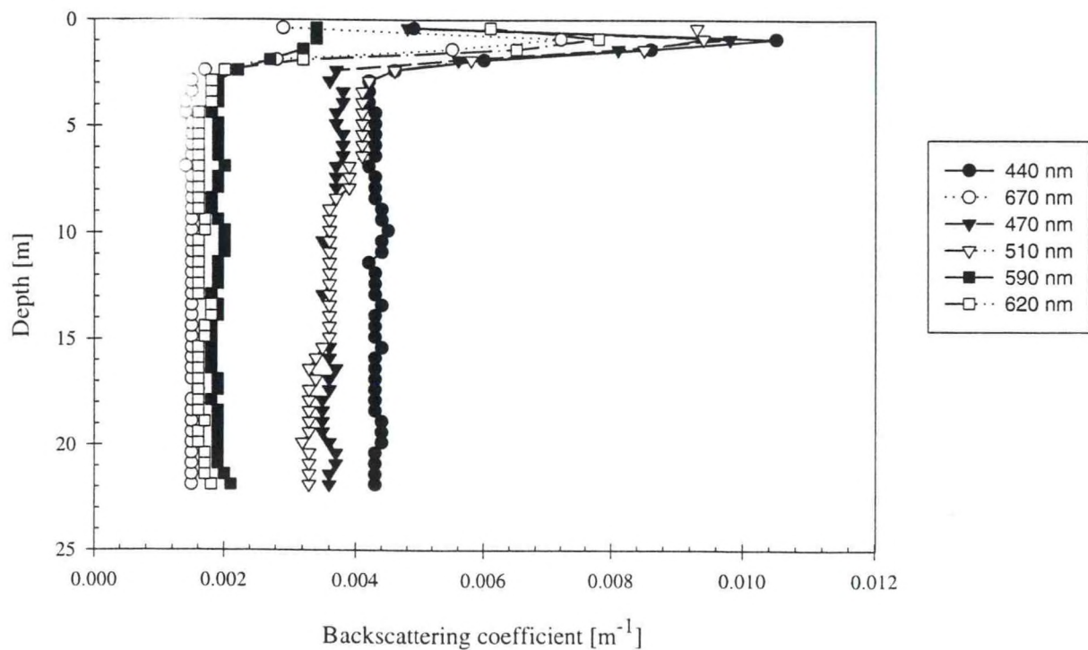
Figure E.3.b - Station 9 Upcast
