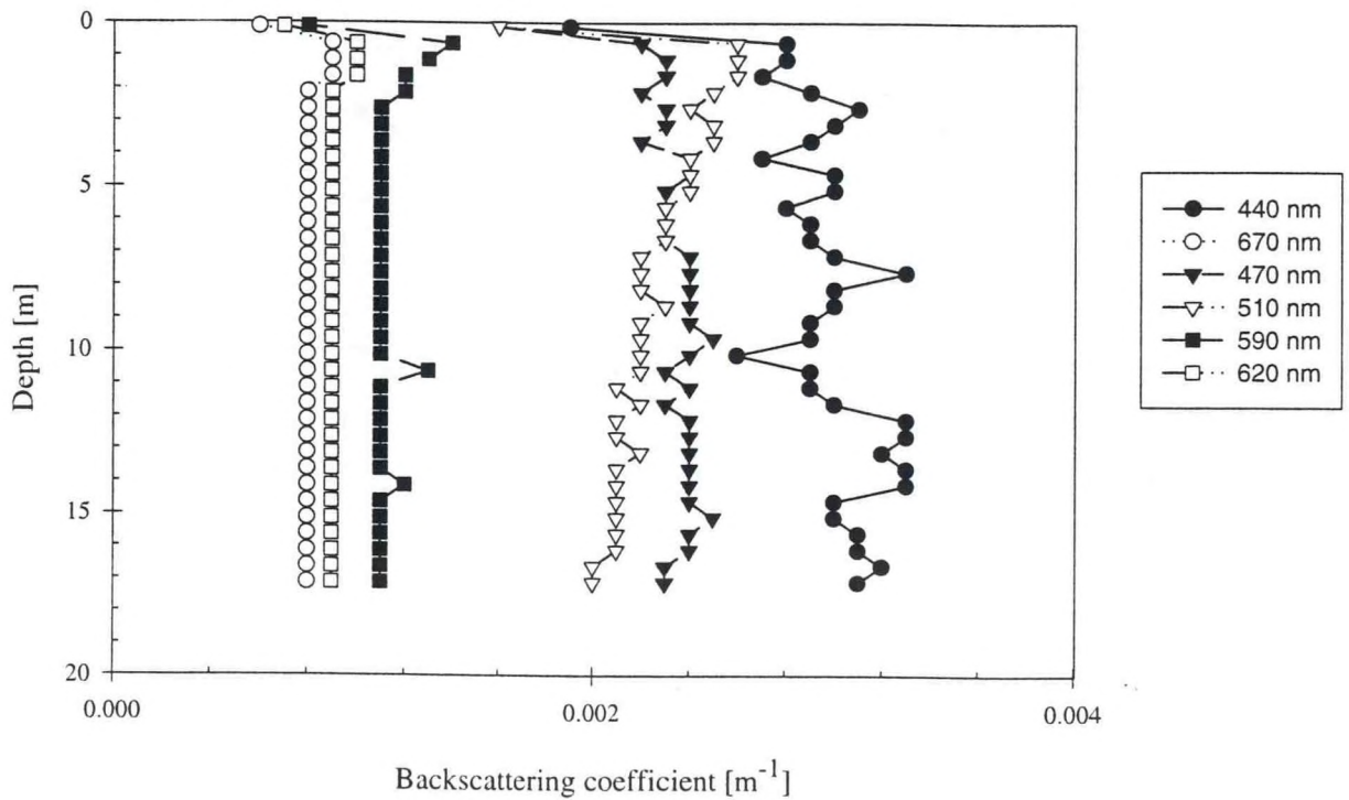
Figure E.5.b - Station 14 Upcast
