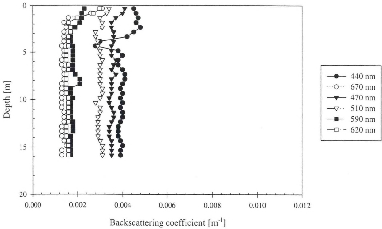
Figure E.2.a - Station 8 Downcast
