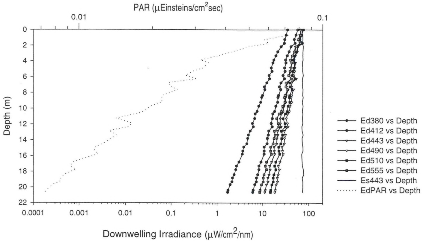
Figure A.3.a - Station 8 Downcast
