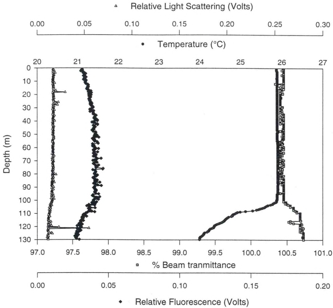
Figure A.10.b - Station 14 Upcast
