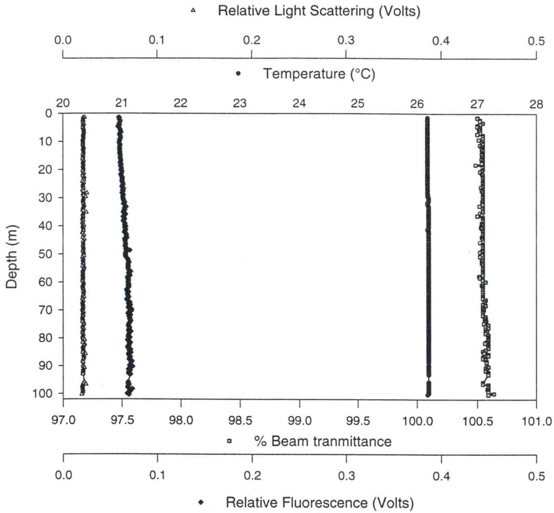
Figure A.7.b - Station 13 Downcast
