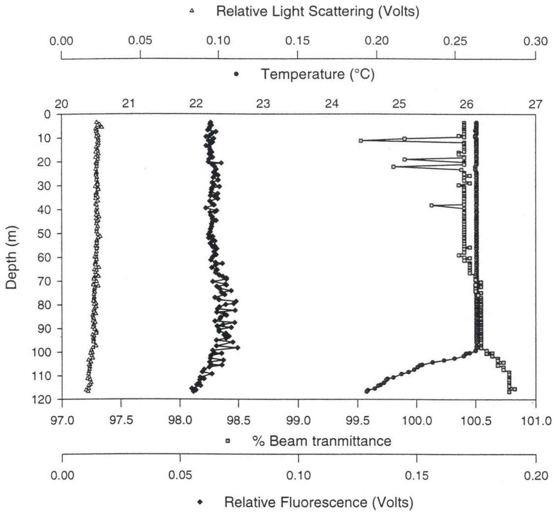
Figure A.11.b - Station 16 Downcast
