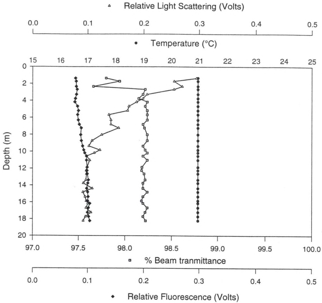
Figure A.1.b - Station 7 Downcast
