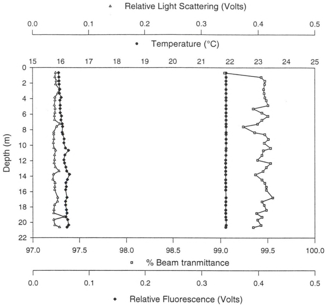
Figure A.3.b - Station 8 Downcast
