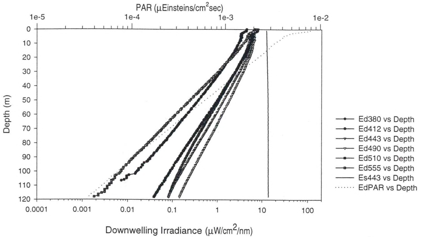
Figure A.12.a - Station 16 Upcast
