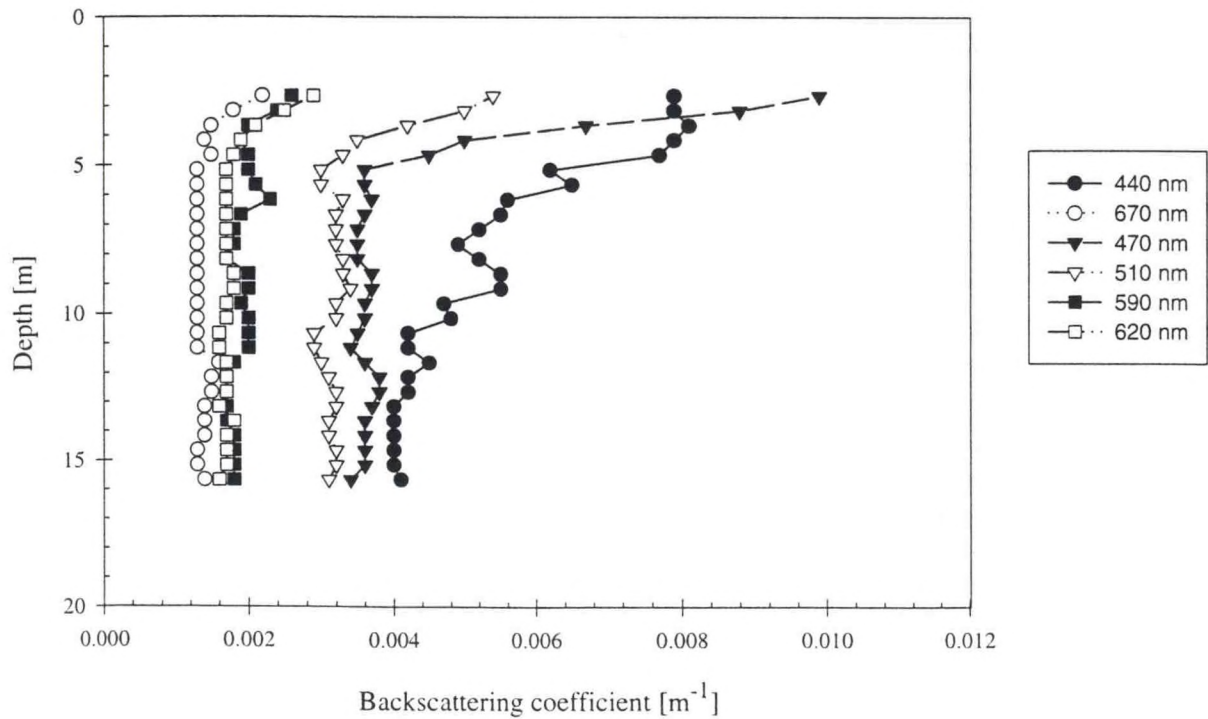
Figure E.2.b - Station 8 Upcast
