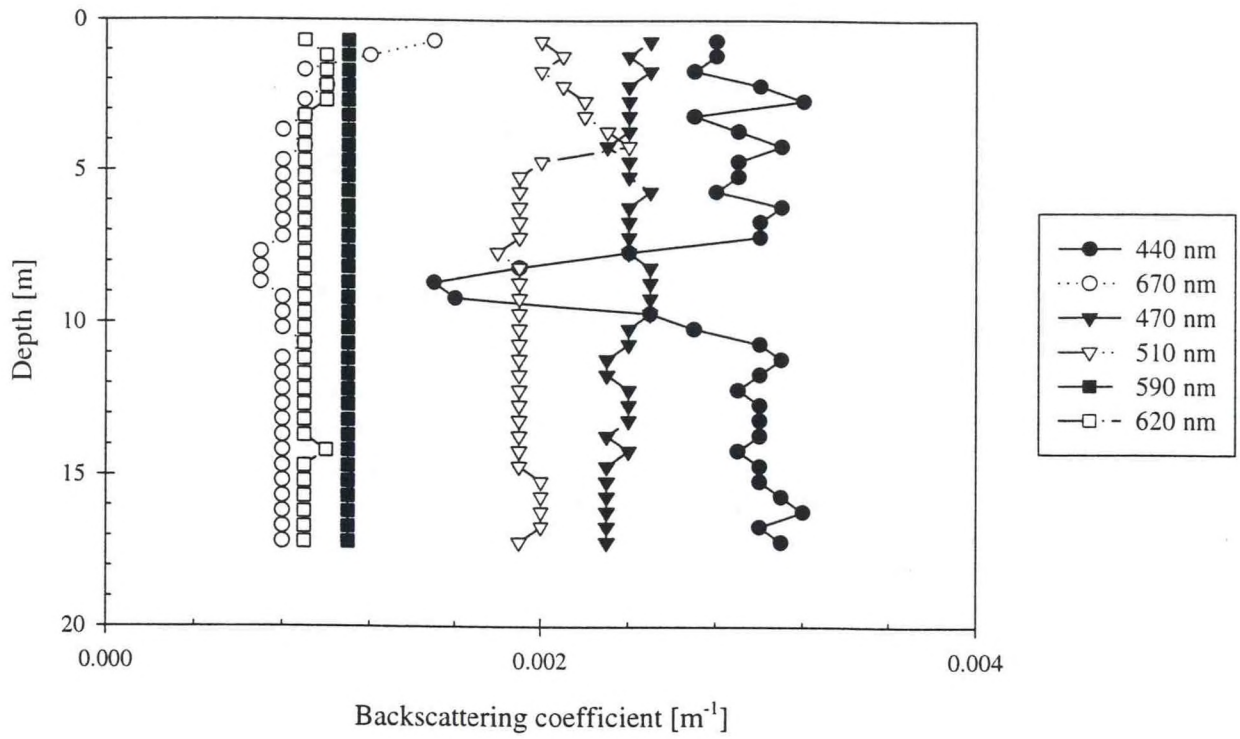
Figure E.5.a - Station 14 Downcast
