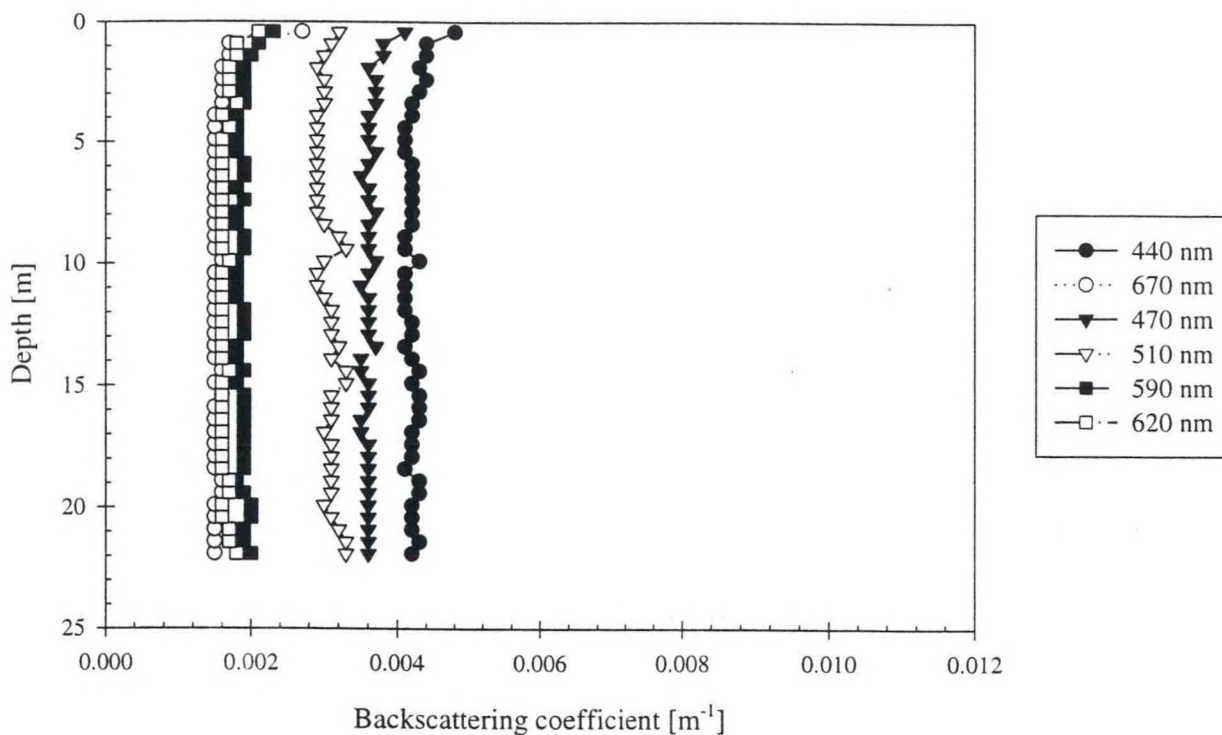
Figure E.3.a - Station 9 Downcast
