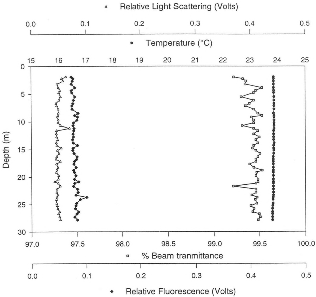
Figure A.5.b - Station 9 Downcast
