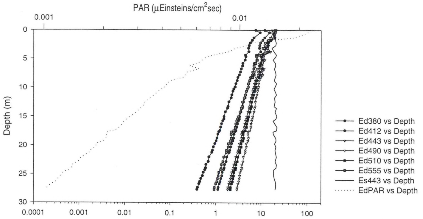
Figure A.6.a - Station 9 Upcast
