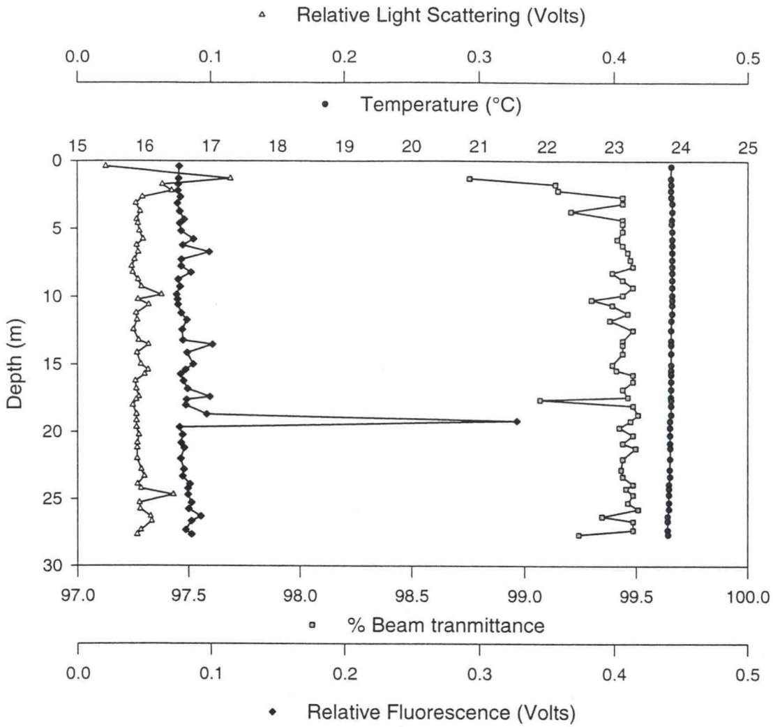
Figure A.6.b - Station 9 Upcast
