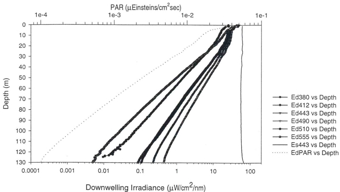
Figure A.10.a - Station 14 Upcast
