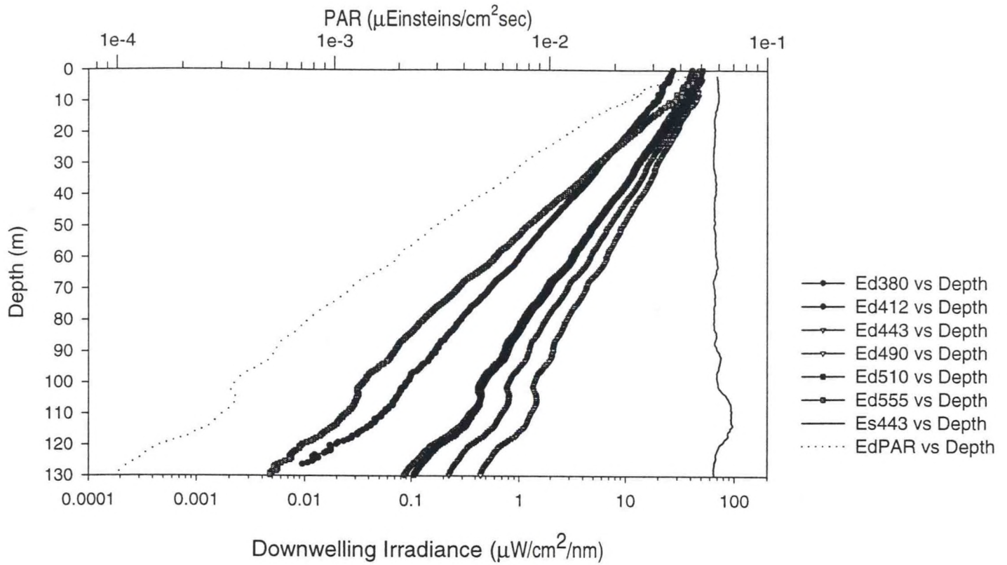
Figure A.9.a - Station 14 Downcast
