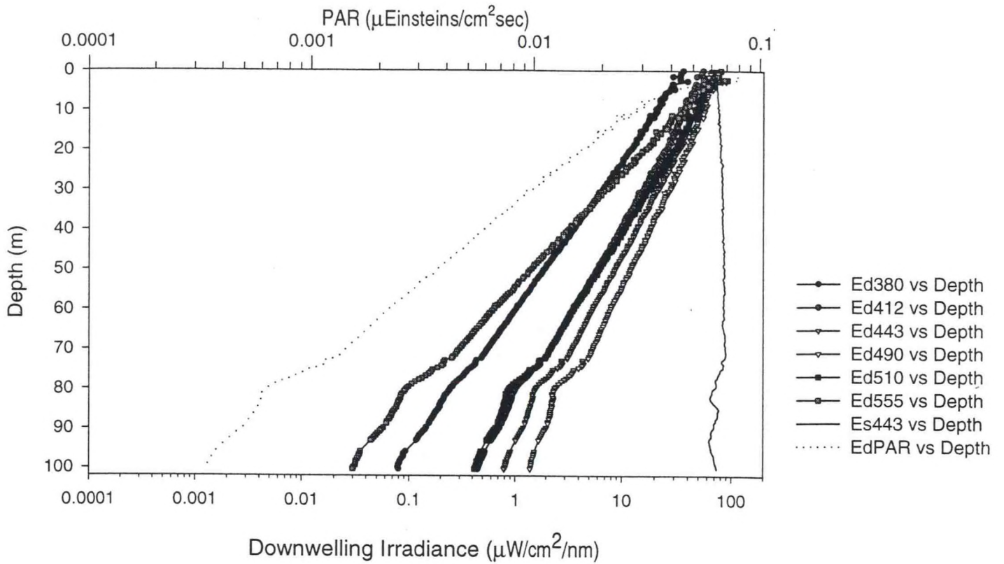
Figure A.7.a - Station 13 Downcast
