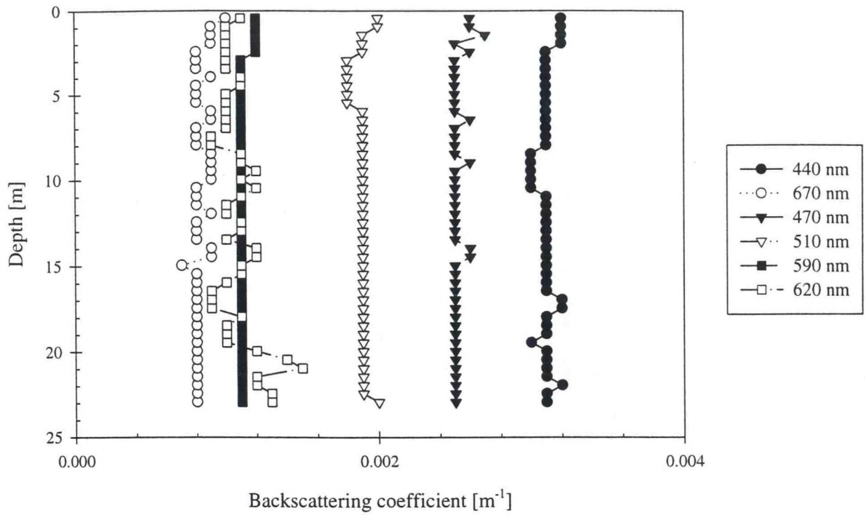
Figure E.6.a - Station 15 Downcast
