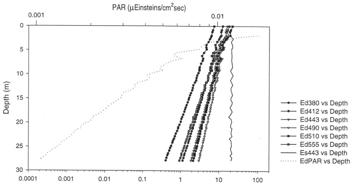
Figure A.5.a - Station 9 Downcast
