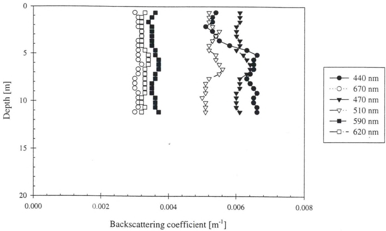
Figure E.1.a - Station 7 Downcast
