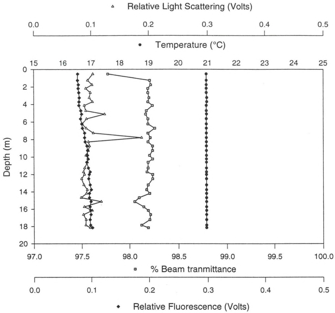
Figure A.2.b - Station 7 Upcast
