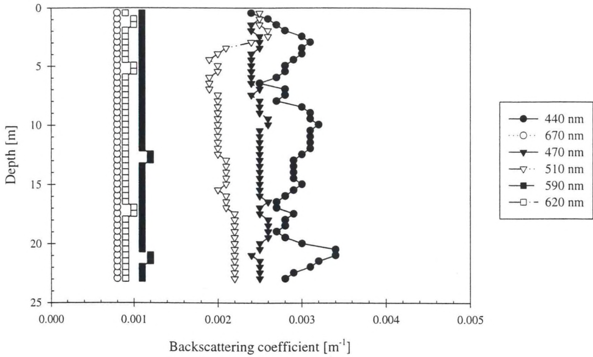
Figure E.4.a - Station 13 Downcast
