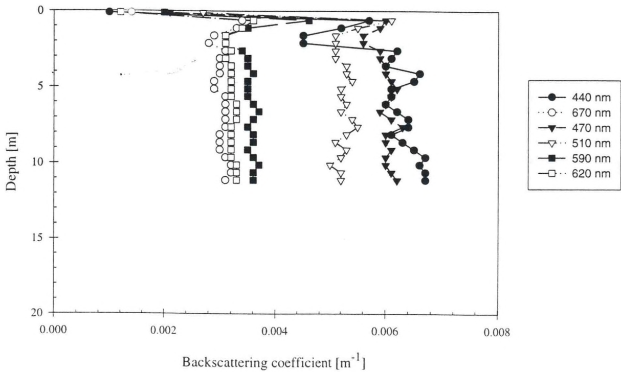
Figure E.1.b - Station 7 Upcast
