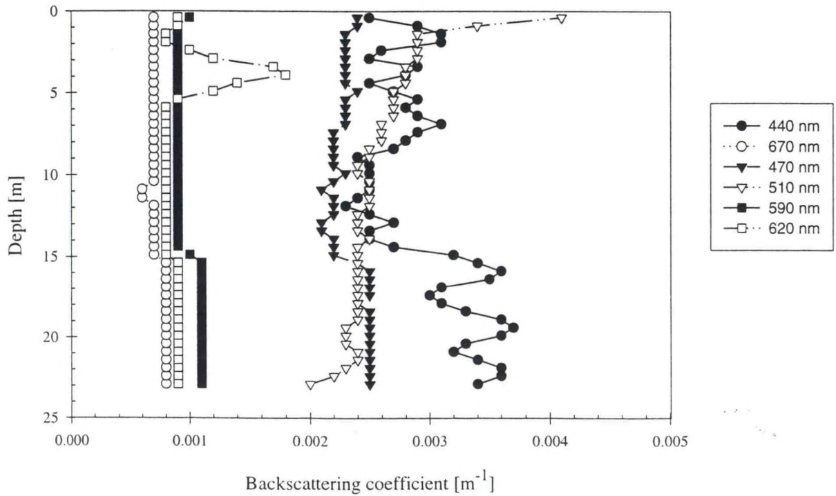
Figure E.4.b - Station 13 Upcast
