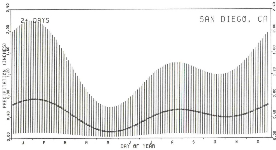
Figure 38. Precipitation amount diagram for San Diego, CA.
