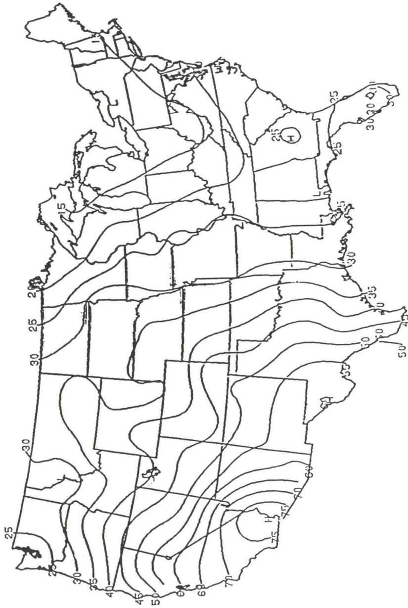
Figure 6. Mean annual relative frequency (%) of entirely dry 5-day periods over the conterminous United States.
