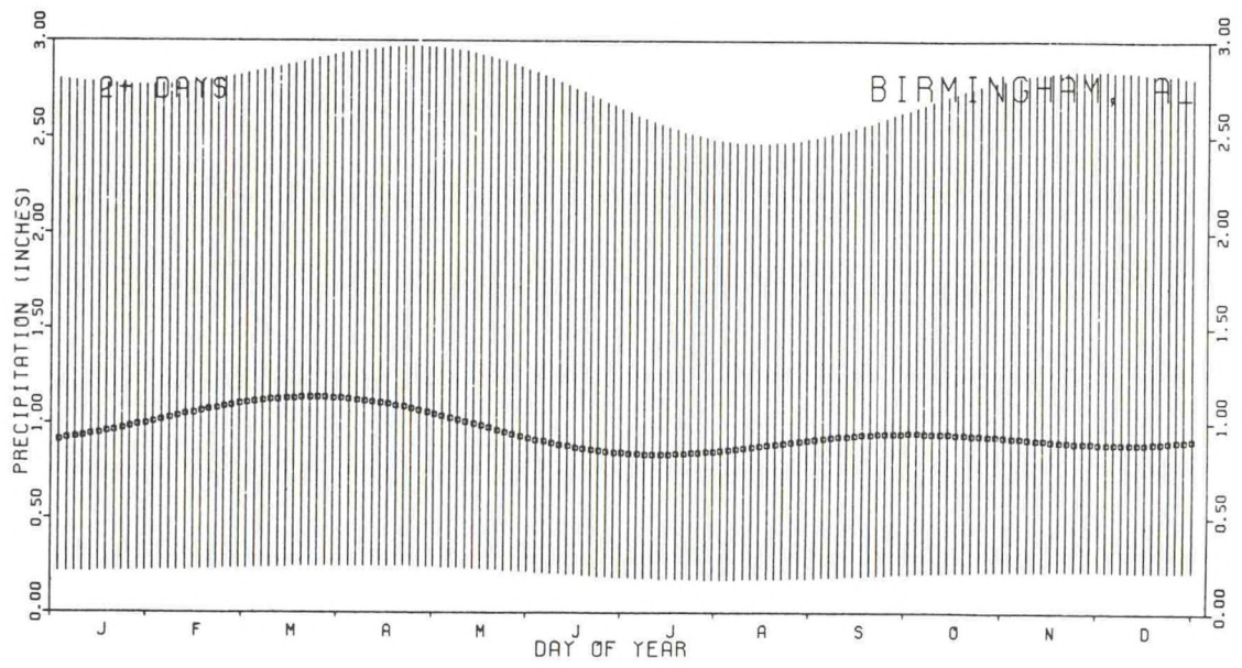
Figure 61. Precipitation amount diagram for Birmingham, AL.
