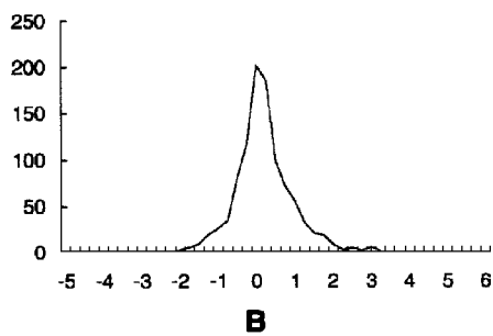
Surface Salinity Middle Atlantic Bight
