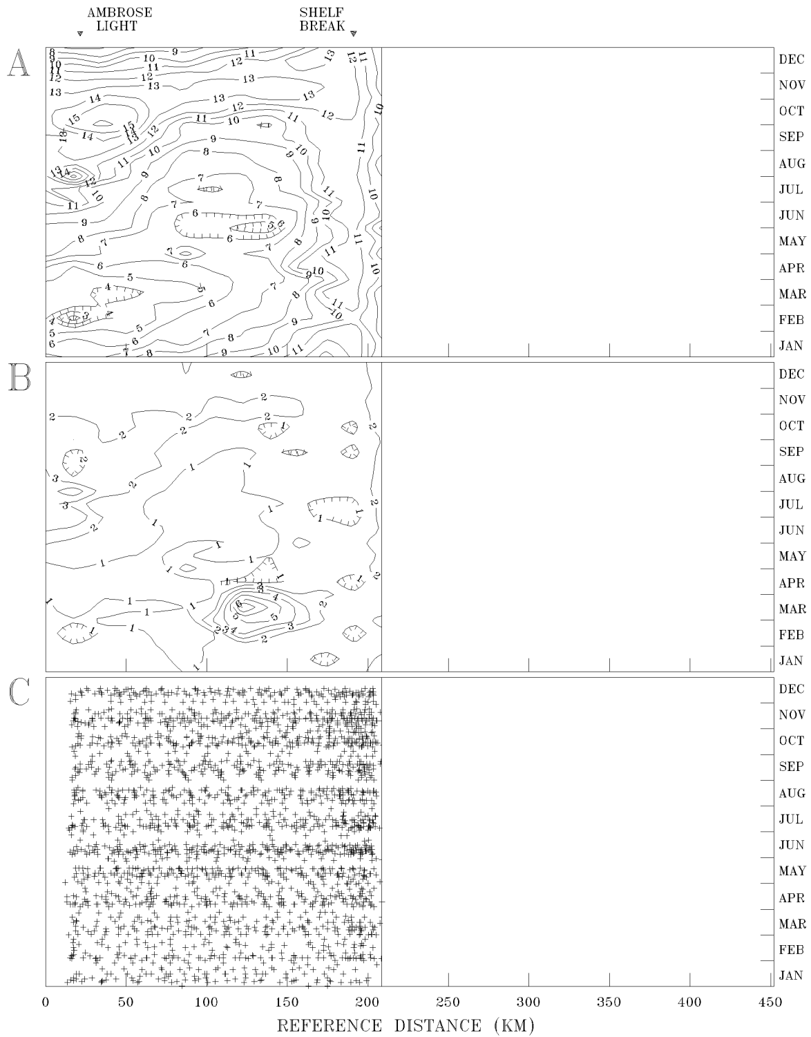
Figure 6. Mean bottom temperature conditions along the Middle Atlantic Bight route during 1978-90. A. Means of measured values (°C). B. Standard deviations of measured values (°C). C. Station locations in time and space. (In panels A and B, values decline on those sides of contour lines with hachures.)
