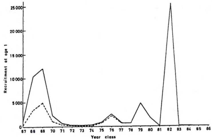
Figure 3.7.—The recruitment at age 1 of horse mackerel, Trachurus trachurus , in the eastern North Atlantic. Recruitment earlier than the 1981 year-class was estimated by back-calculation with the average total mortality rate (Z) of each age group (solid line). Dashed line is back-calculation with only natural mortality rate (M). From ICES (1988).
