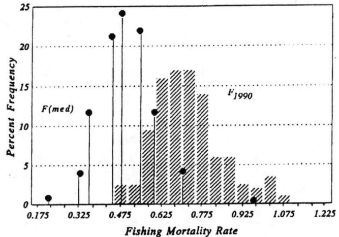
Figure 2.10.—Probability density function for the estimate of fully-recruited fishing mortality rate in 1990 - F_{1990} - (pattern-filled bars); and probability density function for the estimate of F_{med} (vertical lines topped with dots) for Georges Bank cod. Both density functions were estimated using the bootstrap procedure.
