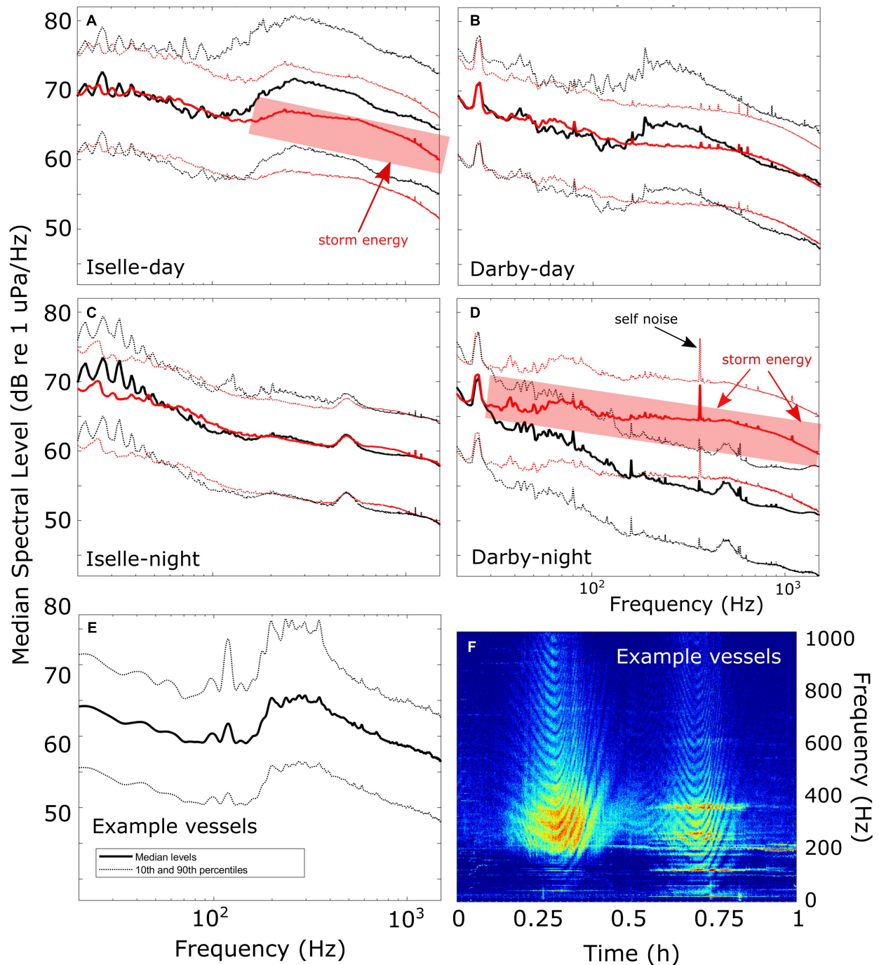
FIGURE 10 | Median spectra (20–1,500 Hz) during the no-vessel periods (red) of Hurricanes Iselle ( A,C ) and Darby ( B,D ) and corresponding day and night from a period 1 week prior to the storms (black), with 10th and 90th percentiles (dotted lines) to indicate variability. Periodic spikes in spectra are due primarily to HARP self-noise and do not represent signals in the broader environment. See ( D ) for labeled example. Elevated spectral levels due to storm energy are indicated by red shaded boxes ( A,D ). Also shown are spectra ( E ) and a spectrogram ( F ) for an example hour with vessel passages that are typical of this data set, having minimal energy below 150 Hz.
