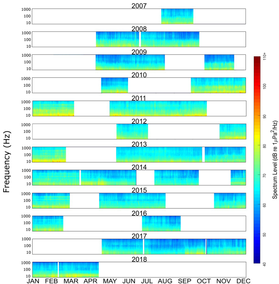
FIGURE 2 | Annual long-term spectral averages over the entire data set from deep water near Kona, Hawai'i. Frequency is along the y-axis (10–1,000 Hz), while time is along the x-axis (Jan–Dec). Sound intensity is shown in color, from lowest (dark blue) to highest (red).
