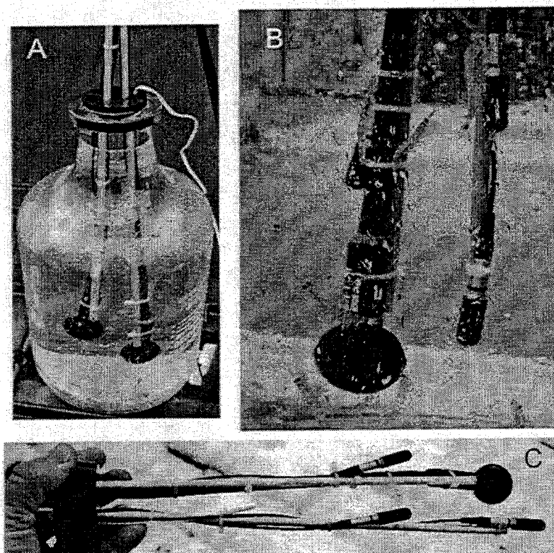
Figure 9.2. (A) 9.3-l carbuoy with transducer, hydrophone, thermocouple, and krill at Cape Shirreff field station; (B) E. superba in the 19.3-l carbuoy during the experiments aboard R/V Yuzhmorgeologiya ; (C) and a rubber stopper fitted with the transducer (projector), three hydrophones, and a thermocouple.
