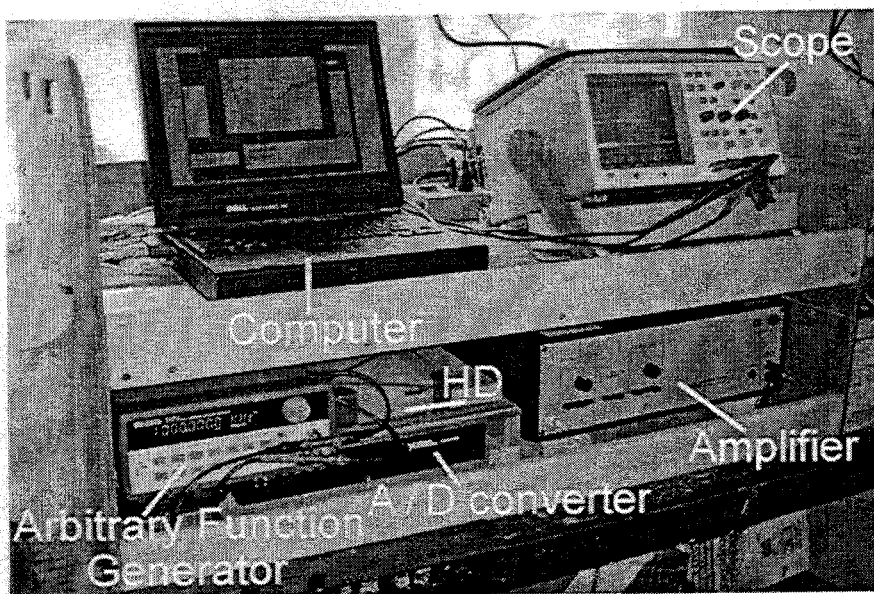
Figure 9.1. Experimental apparatus.
