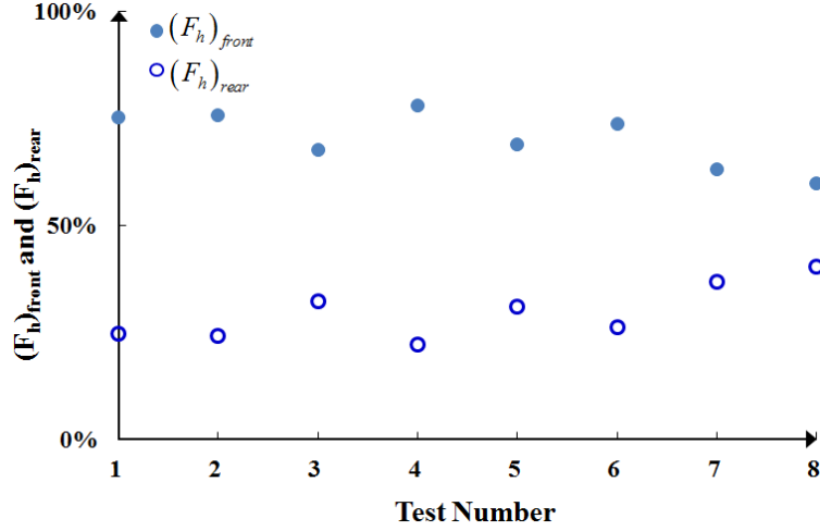
Figure 7. The percentage of contribution from the wave force acting on the front \frac{(F_h)_{front}}{F_{hmax}} (solid circle) and rear wall \frac{(F_h)_{rear}}{F_{hmax}} (empty circle) to the total peak horizontal force (F_{hmax}) = (F_h)_{front} + (F_h)_{rear} for the quarter-circular breakwater.
