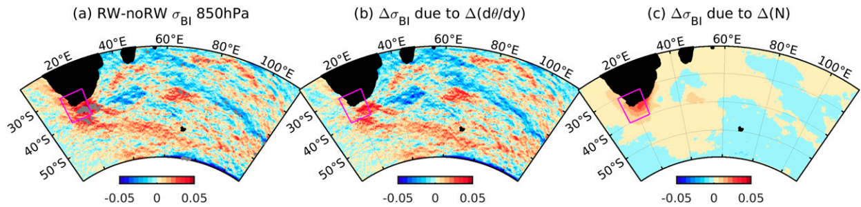
FIG. 10. (a) Annual-mean difference in \sigma_{BI} at 850 hPa ( \text{day}^{-1} ) between RW and noRW, and the differences (b) due to meridional temperature gradient only and (c) due to change in static stability only.
