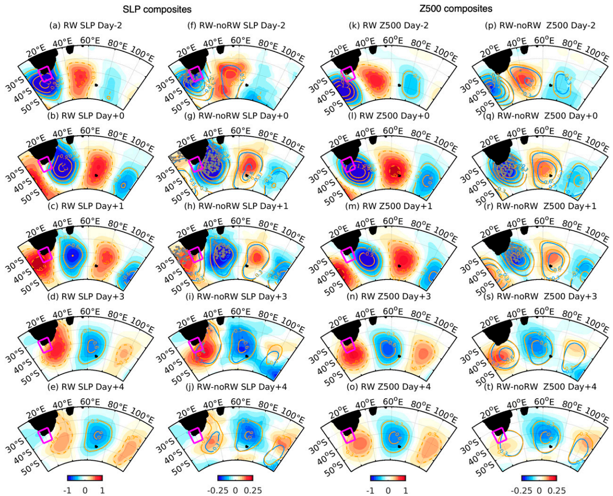
FIG. 11. Lagged composite evolution of the synoptic-scale disturbances associated with the high-THF events in the Agulhas retro-reflection (magenta box): (a)–(j) SLP (hPa) and (k)–(t) Z500 (gpm). Shading in the second and fourth columns show the RW – noRW with the superposed contours denoting the values from RW (orange) and noRW (blue).
