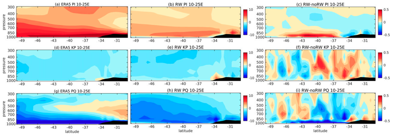
FIG. 13. As in Fig. 12, but showing the latitude–pressure section averaged over 10°–25°E.
