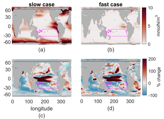
Figure 5. (a, b) Nutrient concentration, \text{mmol N/m}^3 , averaged over a year and the top 100 m. (c, d) Percent change of this field from 2000s to 2100s climate. (a, c) Slow case. (b, d) Fast case.
