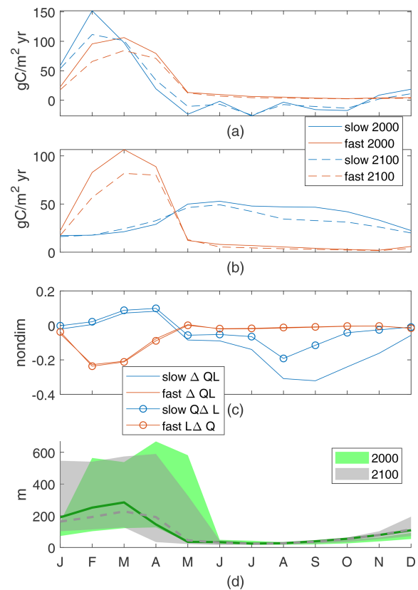
Figure 11. Porcupine Abyssal Plain nutrient supply (a) and production of particles (b). Production controls (c), normalized by maxQL(2000) values for the 2000s: 0.022 for the slow case and 0.015 for the fast case. The discrepancy for the slow case is mainly due to L\Delta Q . Range and mean of monthly-maximum MLD (d).
