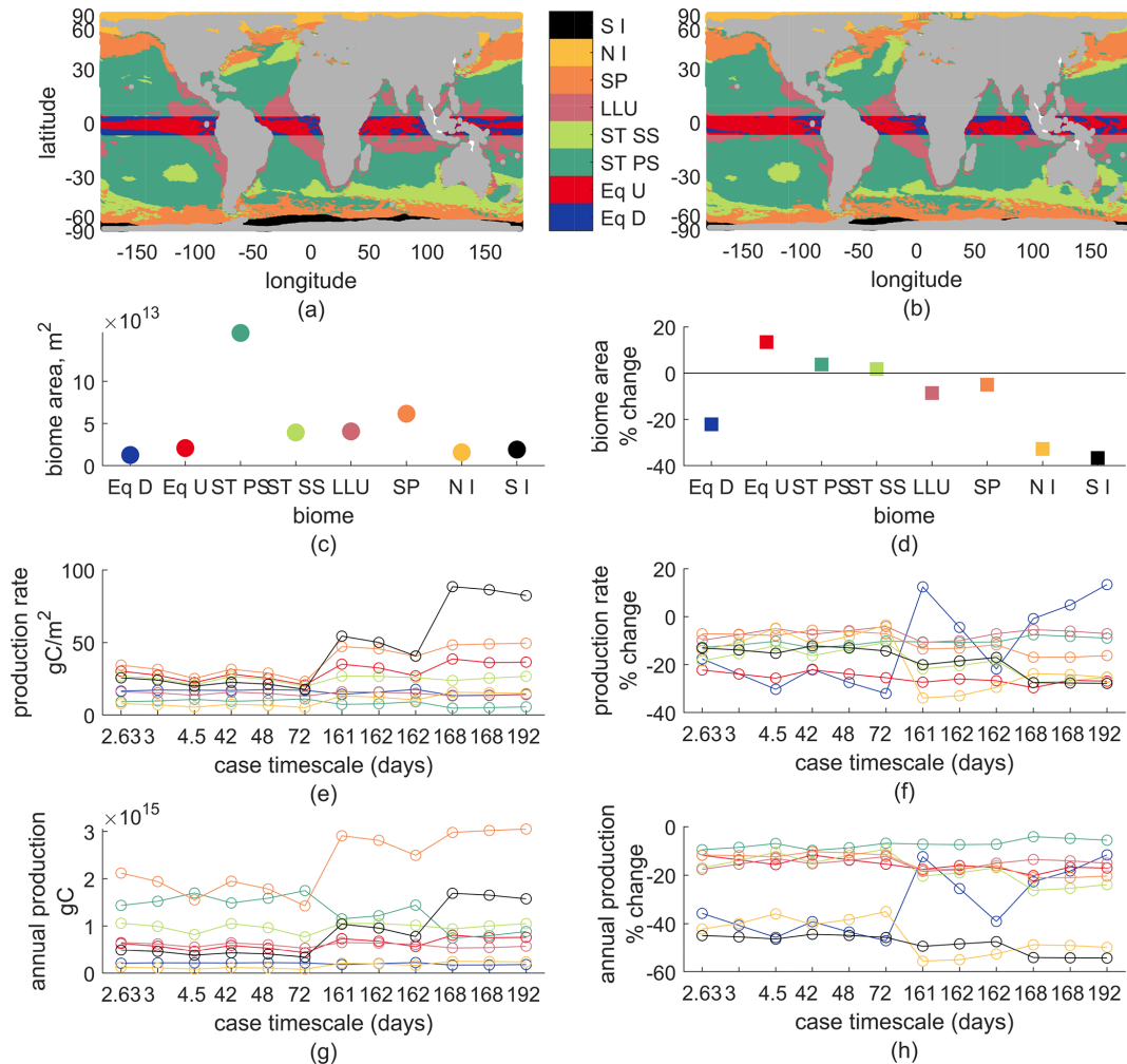
Figure B2. (a) Biomes for 2000, (b) biomes for 2100, (c) biome areas for 2000, (d) percent change in biome area – early–late-21st-century, (e) production rate – annual \text{gC}/\text{m}^2 for each biome (color) and each biogeochemical model parameter ( x axis, case timescale). (f) Percent change in production rate. (g) Total annual production for each biome and biogeochemical model parameter, which is c \cdot e . (h) Percent change in total annual production.
