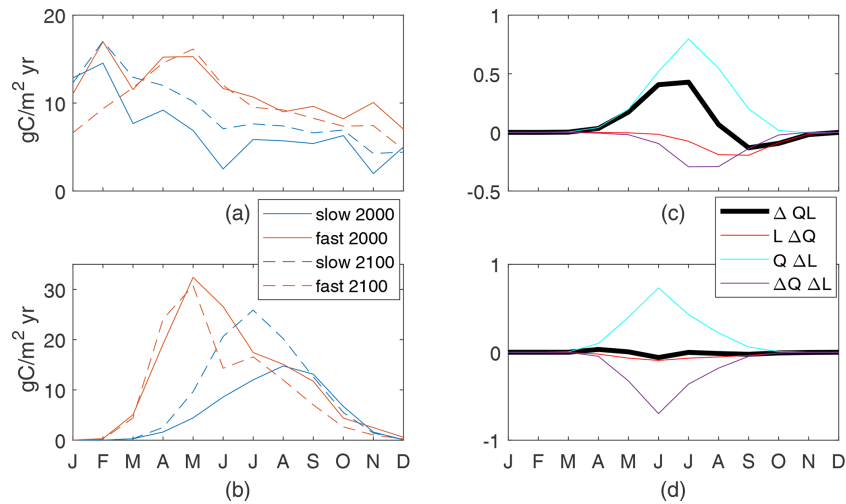
Figure 10. Arctic nutrient supply (a) and production (b). Production controls on the slow (c) and fast (d) cases, normalized by the maximum values of arctic maxQL(2000): 0.021 for the slow case and 0.028 for the fast case.
