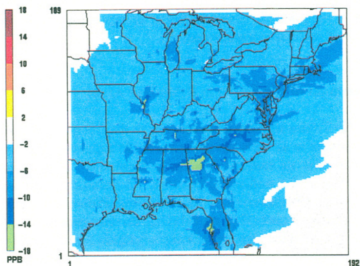
Figure 13. Impact on ozone of Tier-2 Program in 2030 — maximum reduction in peak ozone concentrations.
