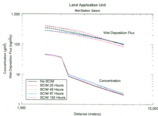
Figure 1a. Maximum concentration and wet deposition estimates at each distance for various sampling intervals using meteorological data for Salem, OR.
