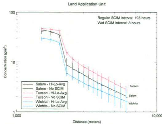
Figure 3a. High, low, and average concentration estimates at each distance from model runs with sampling starting hours 1-24.
