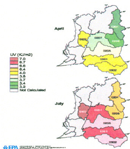
Figure 6. Average daily biologically effective dose of UV by Hydrologic Subregion for 1999. April and July are shown with legend presented in [KJ/m^2] .
