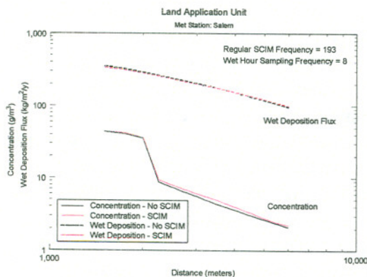
Figure 2a. Maximum concentration and wet deposition estimates at each distance using both separate dry and wet sampling rates and meteorological data for Salem, OR.
