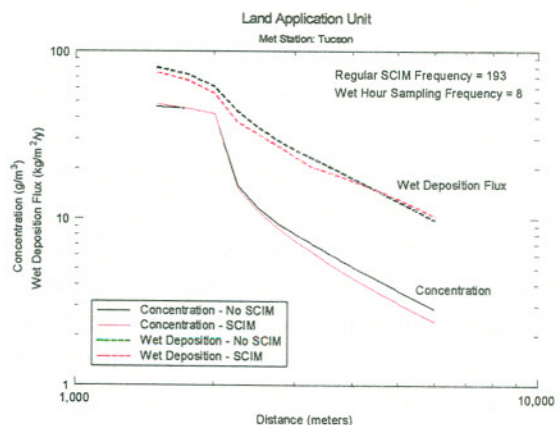
Figure 2b. Maximum concentration and wet deposition estimates at each distance using both separate dry and wet sampling rates and meteorological data for Tucson, AZ.
