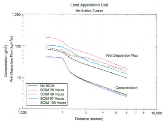
Figure 1b. Maximum concentration and wet deposition estimates at each distance for various sampling intervals using meteorological data for Tucson, AZ.
