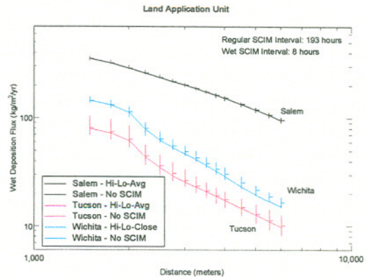
Figure 3b. High, low, and average wet deposition estimates at each distance from model runs with sampling starting hours 1-24.
