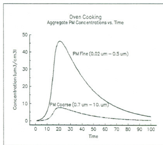
Figure 9. The Particulate Indoor Source Model simulation of fine (0.02um-0.5um) and coarse (0.7um-10.0um) aggregate fractions during oven cooking. The volumetric concentrations are calculated by incorporating the source model into a numerical indoor air model.
