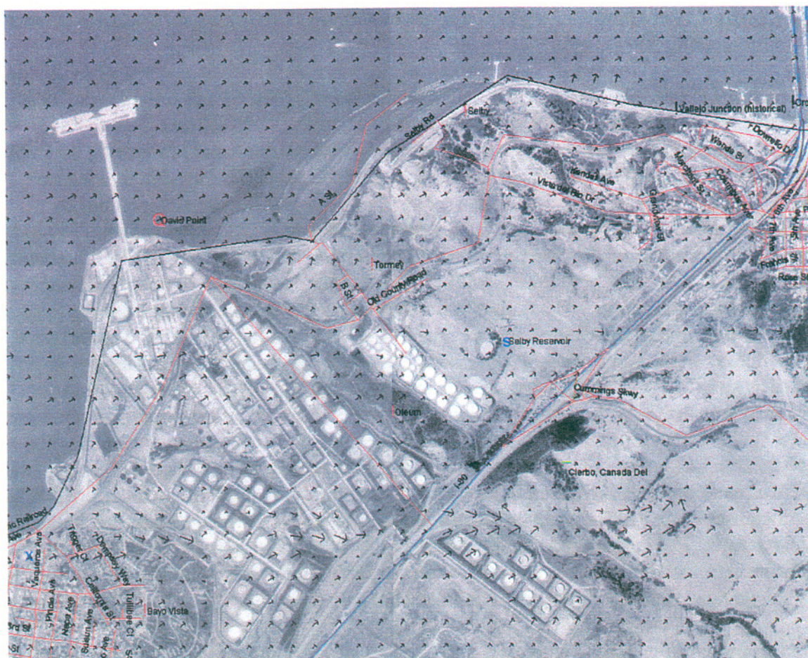
Figure 12. Wind vectors over the refinery produced by the High Resolution Wind Model with initial wind direction from SW.
