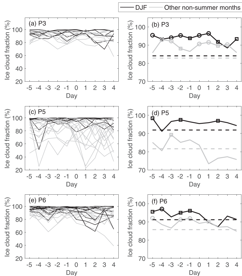
Figure 5. Ice cloud area fractions of one-layer cloud groups from 5 days before to 4 days after the start day of each of the identified MJO phases in DJF (black) and other nonsummer months (gray) over the corresponding subarea. The left panels (a), (c), and (e) include the results for all the identified MJO phases over P3, P5, and P6, respectively; in the corresponding right panels (b), (d), and (f), the solid curves are the composite means, and the dashed lines are the time-average means. The circles and squares in the right panel mark the composite means that are greater than the corresponding time-average means at significance levels of 0.01 and 0.05, respectively, based on a one-tail t test. The daily mean ice cloud fraction data over each subarea was first averaged to get the pentad mean data, and the pentad mean data were then used for calculating the time-average mean and the significance test in DJF and other nonsummer months, respectively.
