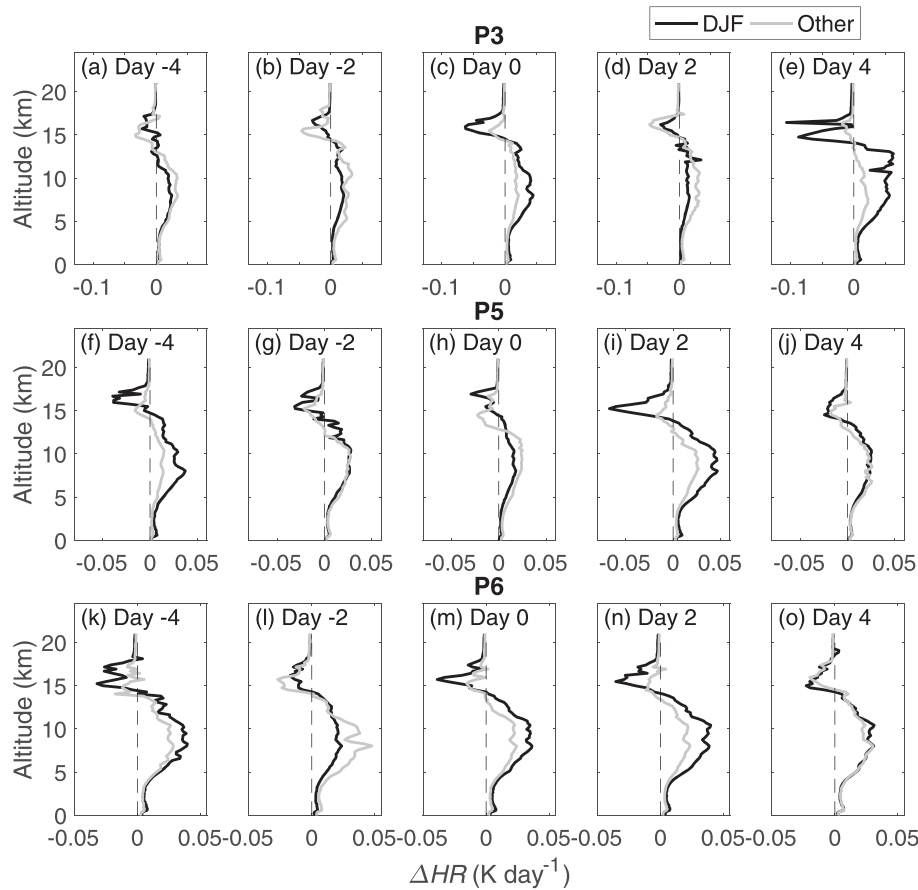
Figure 10. Same as Figure 9 except for the difference between HR calculations ( \Delta HR ; K \text{ day}^{-1} ) with and without longwave scattering. P3 has a larger range in x -axis values.
