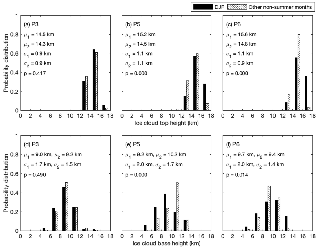
Figure 3. Probability distributions of the heights of the pentad one-layer ice cloud tops (a–c) and bases (d–f) in DJF (black bars) and other nonsummer months (hatched bars) during September 2006 to May 2010 over the three study subareas: P3 (a and d), P5 (b and e), and P6 (c and f). In all panels, \mu_1 and \mu_2 are the mean pentad heights, and \sigma_1 and \sigma_2 are the standard deviations in DJF and other nonsummer months, respectively. In each panel, p is the p value of the two-sided Kolmogorov-Smirnov test between the samples in DJF and other nonsummer months.
