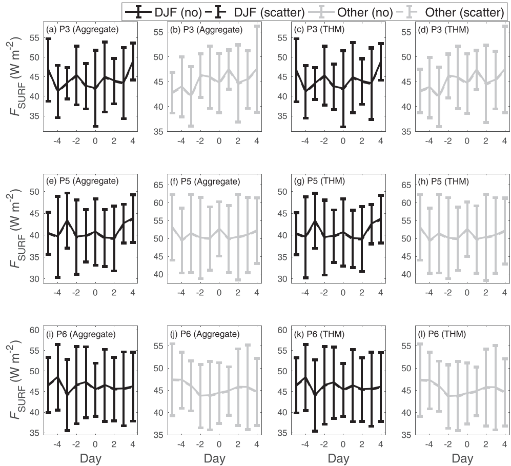
Figure 8. Same as Figure 7 except for F_{\text{SURF}} ( \text{W m}^{-2} ).
