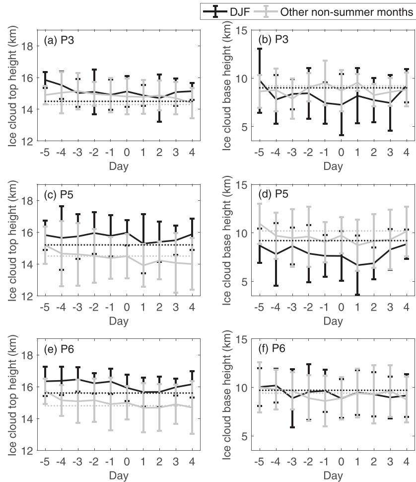
Figure 6. Composite mean one-layer ice cloud top (a, c, and e) and base (b, d, and f) heights from 5 days before to 4 days after the start day of all cases of the specified MJO phase in DJF (black) and other nonsummer months (gray) over the labeled subarea. The error bars mark the standard deviations. In each panel, the dotted lines are the corresponding time-average means shown in Figure 3.
