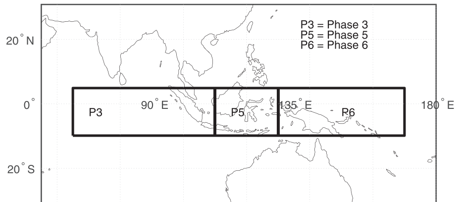
Figure 1. The study area. Each box represents the region where the minimum OLR occurs during a particular MJO phase.
