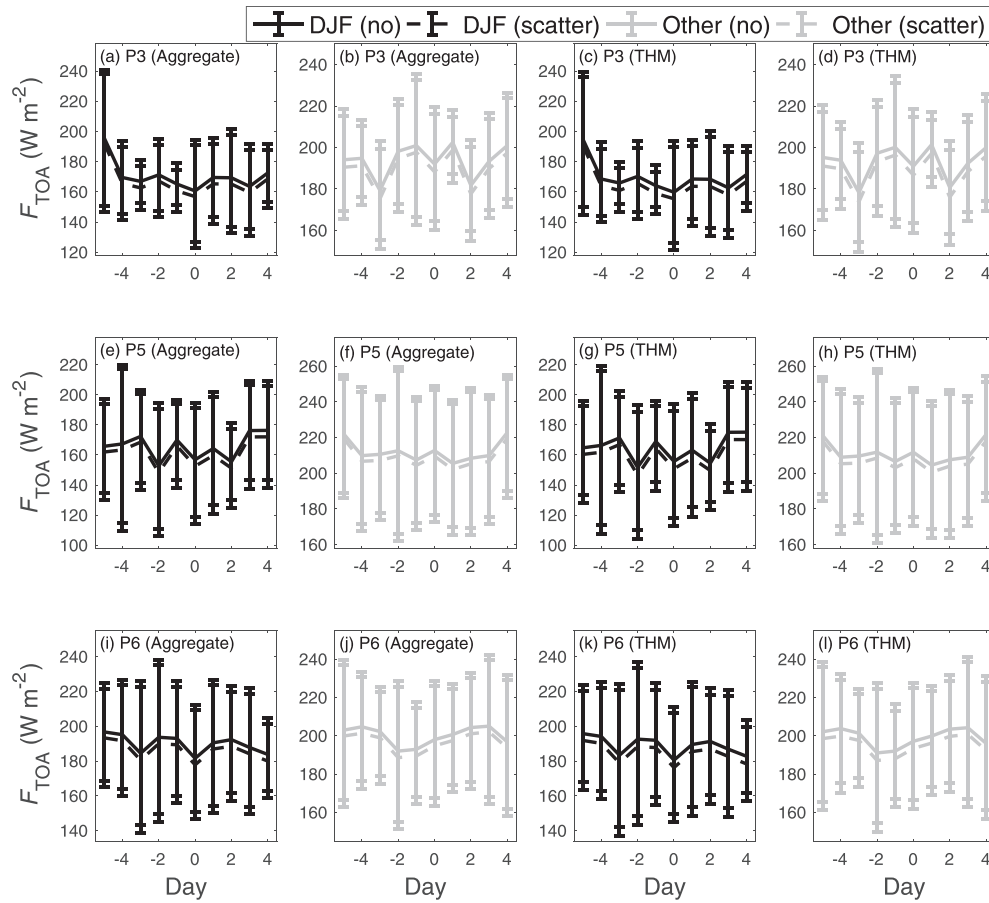
Figure 7. The composite net longwave radiation at the top of the atmosphere ( F_{TOA} ; W m^{-2} ) from 5 days before to 4 days after the specified MJO phase onset in DJF (black) and other nonsummer months (gray) over the one-layer ice cloud area in P3, P5, and P6. In each panel, the solid lines are the composite F_{TOA} means with longwave scattering ignored, and the dashed lines are the corresponding F_{TOA} means with longwave scattering considered; the error bars mark the composite standard deviations. The first (a, e, and i) and second (b, f, and j) columns are based on the aggregate ice cloud particle model, and the third (c, g, and k) and fourth (d, h, and l) columns use the THM.
