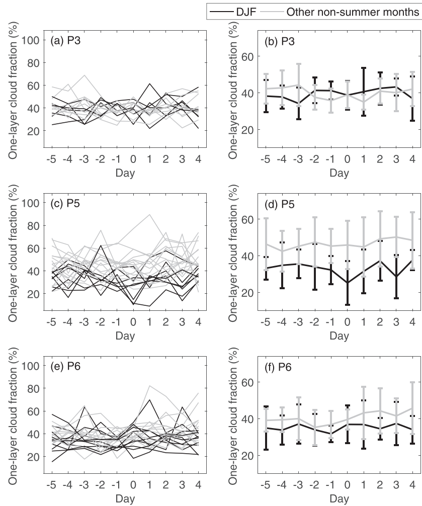
Figure 4. One-layer cloud fractions from 5 days before to 4 days after the start day of each of the identified MJO phases in DJF (black) and other nonsummer months (gray) over the corresponding subarea. The left panels (a), (c), and (e) include the results for all the identified MJO phases over P3, P5, and P6, respectively; in the corresponding right panels (b), (d), and (f), the solid curves are the composite means, and the error bars are the standard deviations.
