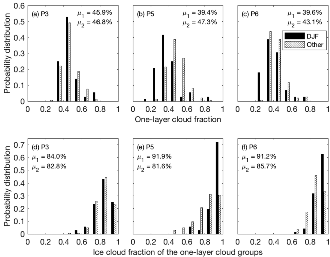
Figure 2. Probability distributions of the one-layer cloud area fraction (a–c) and ice cloud area fraction of the one-layer cloud groups (d–f) in DJF (black bars) and other nonsummer months (hatched bars) during September 2006 to May 2010 over the three study subareas: P3 (left panels), P5 (middle panels), and P6 (right panels). In the upper panels, \mu_1 and \mu_2 are the means of the pentad one-layer cloud fraction in DJF and other nonsummer months, respectively. In the lower panels, \mu_1 and \mu_2 are the means of the pentad ice cloud fraction of the one-layer cloud groups in DJF and other nonsummer months, respectively.
