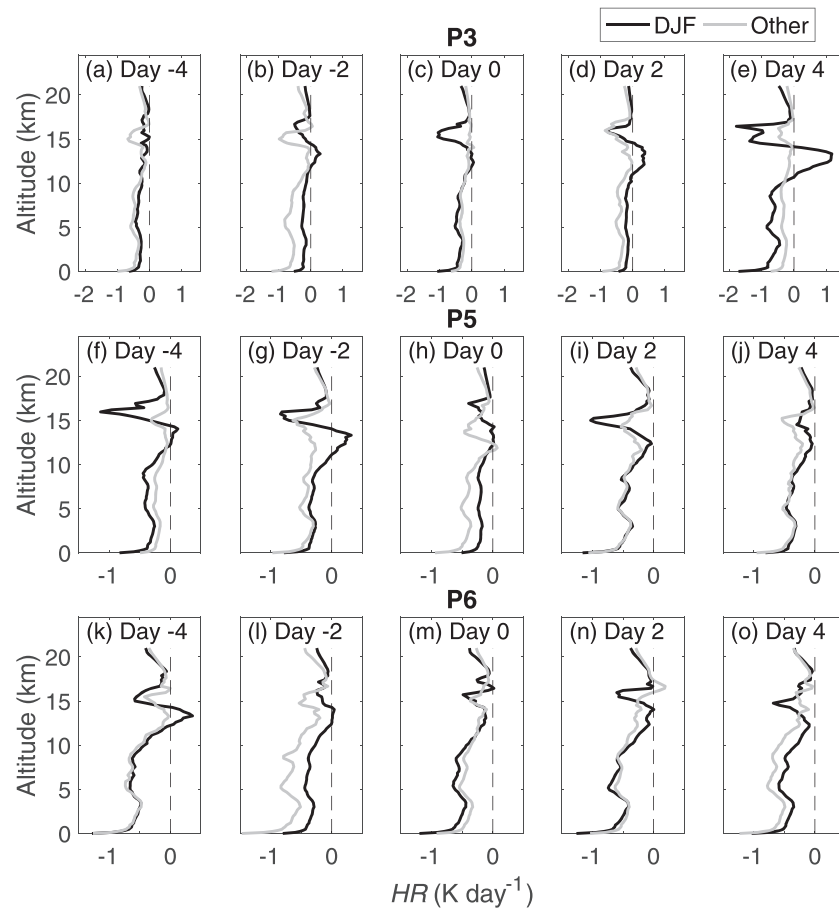
Figure 9. Composite mean area-weighted HR calculations ( K \text{ day}^{-1} ) with longwave scattering considered on days -4 (a, f, and k), -2 (b, g, and l), 0 (c, h, and m), 2 (d, i, and n), and 4 (e, j, and o) in DJF (black) and other nonsummer months (gray) over the one-layer ice cloudy area in the three subareas. The aggregate model is used in the calculations. P3 has a larger range in x -axis values.
