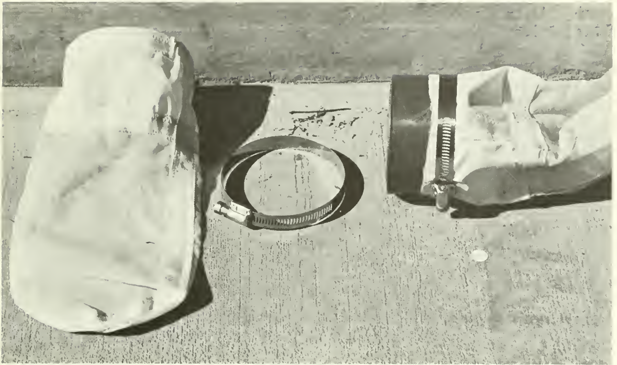
Figure 7.—Cod end (left)—(see Table 1 for source of specifications) used to concentrate plankton collected by net, detached from plankton net (right). Both are fastened with hose clamps to an adapter made of polyvinyl chloride (PVC) pipe. The pipe is approximately 4 inches (127 mm) long, 3-1/2-inches (95 mm) O.D. with 1/4-inch (6.5 mm)-thick wall. It is turned down about 3/32 inch (2.5 mm) along its length leaving flanges at each end to keep hose clamps from slipping off during tow; dimensions are not critical when turning the pipe.
