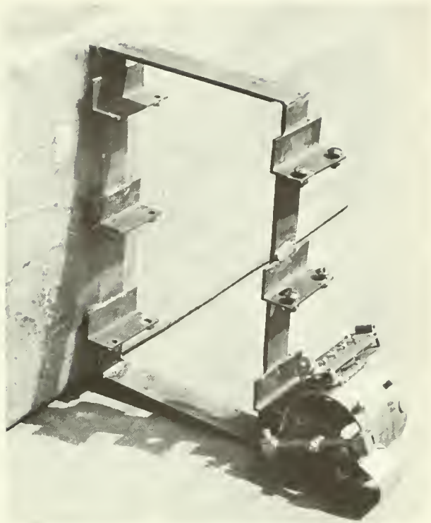
Figure 34.—Brass frame under calibration board (see Fig. 33) on which to hang flowmeters. Only three meters are calibrated at one time, the hangers nearest the board are not used; meter readings were found to be erratic because of the turbulence in that area. The brass frame is 8 inches \times 14 inches (20.3 \times 35.5 cm) made of four pieces of brass welded at their ends. The brass material is 3/16 inch \times 2 inches (5 \times 51 mm). The brass angles on which to hang the meters are cut from 1/8-inch (3 mm) stock, 1-1/4 inches (32 mm) each side, 3 inches (72 mm) long. Holes are bored to conform to distance on centers of holes in meter lugs. Nuts are welded in position to take bolts that slip fit through meter lugs. Meters just hang on the bolts.
