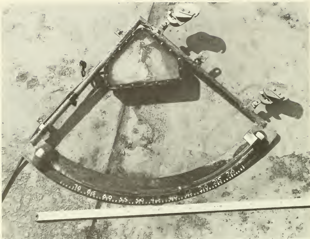
Figure 8.—Inclinometer used to measure the angle of stray, wire angle, of towing cable during plankton net tow (also see Figure 3 where pendulum indicator is more clear; see Table 1 for source of specifications).
