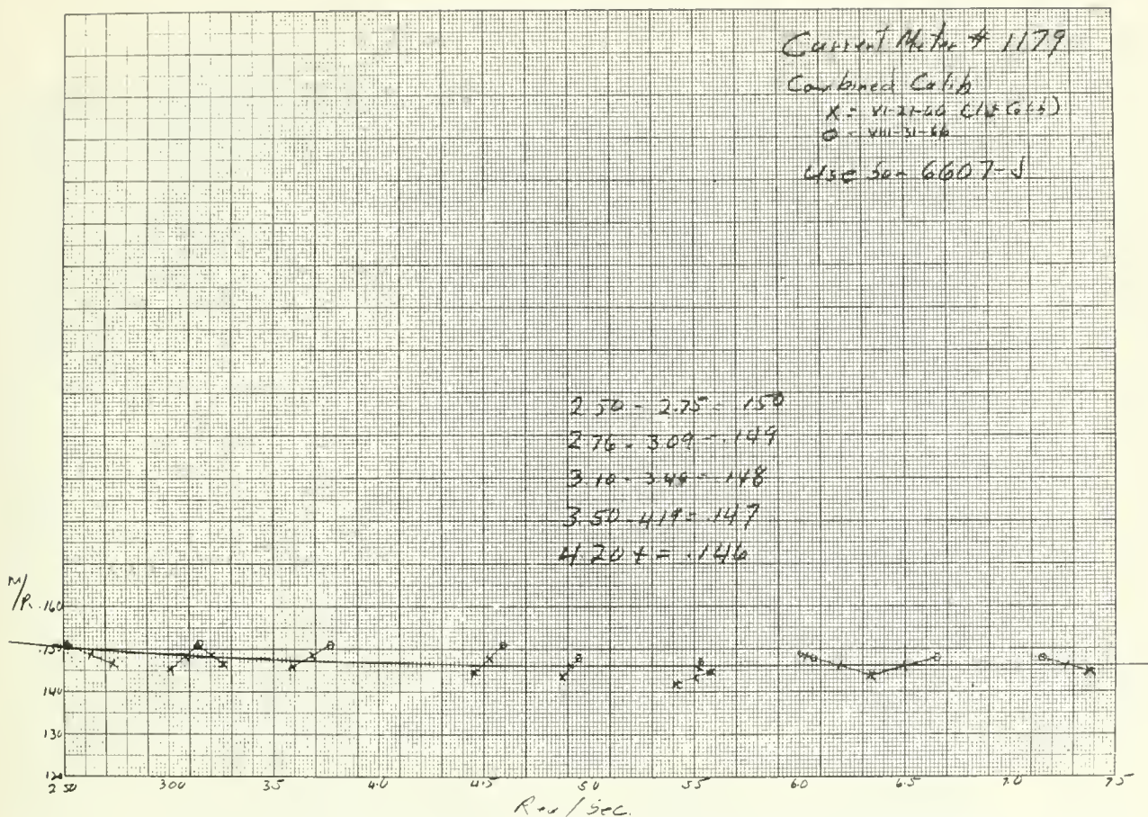
Figure 36.—Calibration curve for flowmeter #1179 obtained by plotting two sets of calibrations and drawing the curve on the average of the calibration points. The data of the first calibration are shown in Figure 35, the second, a similar set, made after cruise 6607-J are not illustrated.
