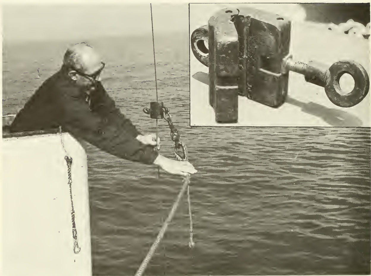
Figure 12.—Cable clamp attaching plankton net lead line to towing cable. Clamp is tightened (and loosened) with a steel rod (suspended in bucket) inserted into bolt eye. Insert: cable clamp, opened, showing grooves to accommodate cable. (See Table 1 for source of supply). Note swivel between the two shackles (see legend for Fig. 6). Small line hanging below man's right hand is the safety line to be hooked to the towing cable above the clamp. Line with hook hanging at side of bucket is used to retain the towing cable, after the weight is lowered, if the ship has a slight way-on so that clamp and inclinometer can be attached.
