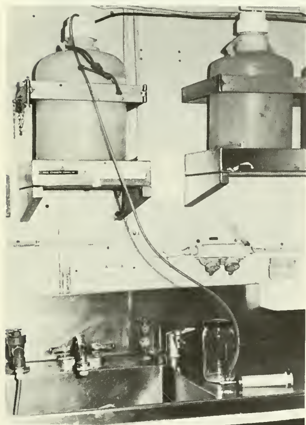
Figure 16.—Installation of 5-gal (18.91 liters) heavy-gauge plastic carboys (see Table 1 for source of supply) of concentrated formaldehyde aboard R/V David Starr Jordan —carboy, upper right is reserve supply. Metal straps are hinged to release carboys and locked at one corner by metal pin through the hinge. Screw-top plastic cap is holed to allow siphon action. Siphon is started by pulling formaldehyde with action of automatic double valve on 50-ml syringe, bottom right (see Fig. 17). At middle right is 20-mm plastic syringe with cannula (see Table 1 for source of supply) and a 1-quart jar containing saturated solution of sodium borate in seawater (see text for buffering plankton samples).
