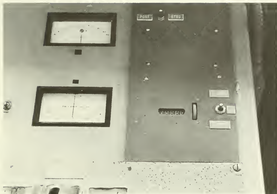
Figure 9.—Microammeter (lower left) on console in wheelhouse to indicate angle of stray registered by the telemetering inclinometer shown in Figures 3 and 8 (see Table 1 for source of specifications). “0” indicates the desired 45° wire angle. “200 left” is 5° increase — 50° on inclinometer. “200 right” is 5° decrease — 40° on inclinometer.
