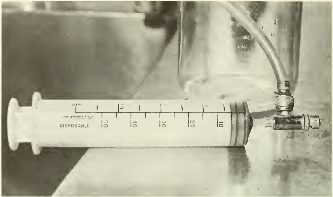
Figure 17.—Two-way, double action valve on syringe (see Table 1 for source of supply). Usually the valve is fixed to the syringe by a screw-on action. In this illustration, the valve is fitted tightly by friction to a disposable plastic syringe.
