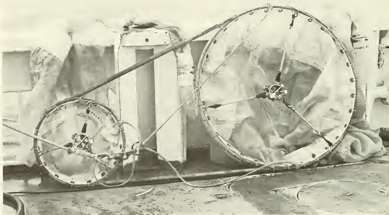
Figure 6.—Standard CalCOFI nets, 1-m mouth opening, 505- \mu mesh throughout, and 0.5-m mouth opening, 333- \mu mesh throughout (see Table 1 for source of specifications). Detachable cod ends are described in Figure 7. Flowmeters (see Table 1 for source of supply) are suspended in the mouth opening (also see Figures 13 and 15) by cloth-covered rubber shock cord. The cord is permanently attached to small metal eyes welded to the mouth rings.
