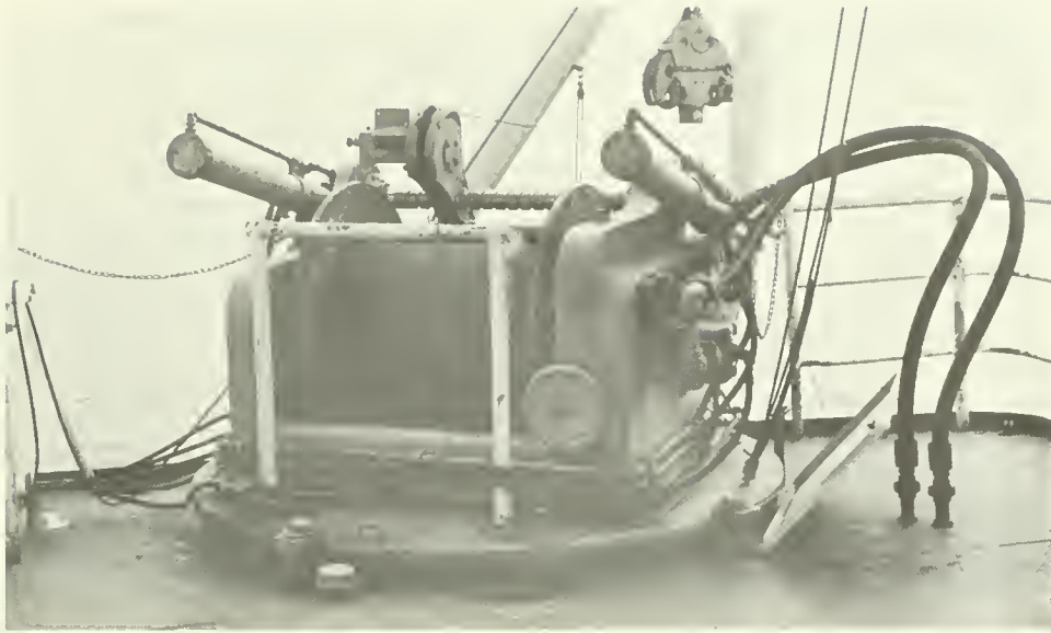
Figure 2.—Starboard winch on NMFS research vessel David Starr Jordan used for plankton tows and Nansen bottle casts (see Table 1). Details on drum size, wire, boom, and block are described in the text.
