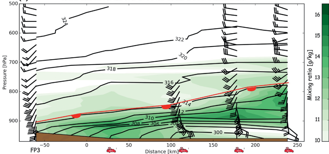
FIG. 10. (a) Surface map at 0600 UTC 24 Jun following CI, with sea level isobars (solid black), wind barbs (in knots; full barb is 10 kt) and radar reflectivity from relevant WSR-88Ds (red dots). (b) Vertical cross section from SW to NE across the warm front, based on five radiosondes released at 0300 UTC 24 Jun from the fixed or mobile sites shown in (a). Contours are potential temperature (K), color shades indicate mixing ratio ( \text{g kg}^{-1} ), and wind barbs are plotted at each sounding location (full barb is 10 kt).
