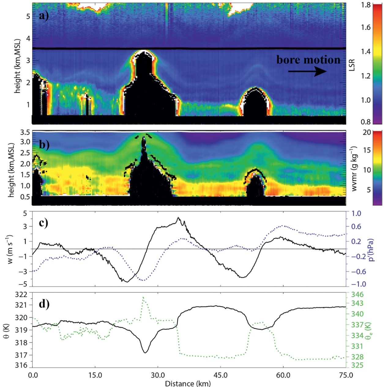
FIG. 9. Transect of a bore encountered by the UWKA on 20 Jun. (a) Lidar scattering ratio obtained from WCL above flight level (3.55 km MSL) and CRL below flight level; (b) CRL water vapor mixing ratio; (c), (d) flight-level data, including air vertical velocity w , perturbation pressure p' , potential temperature \theta , and equivalent potential temperature \theta_e .
