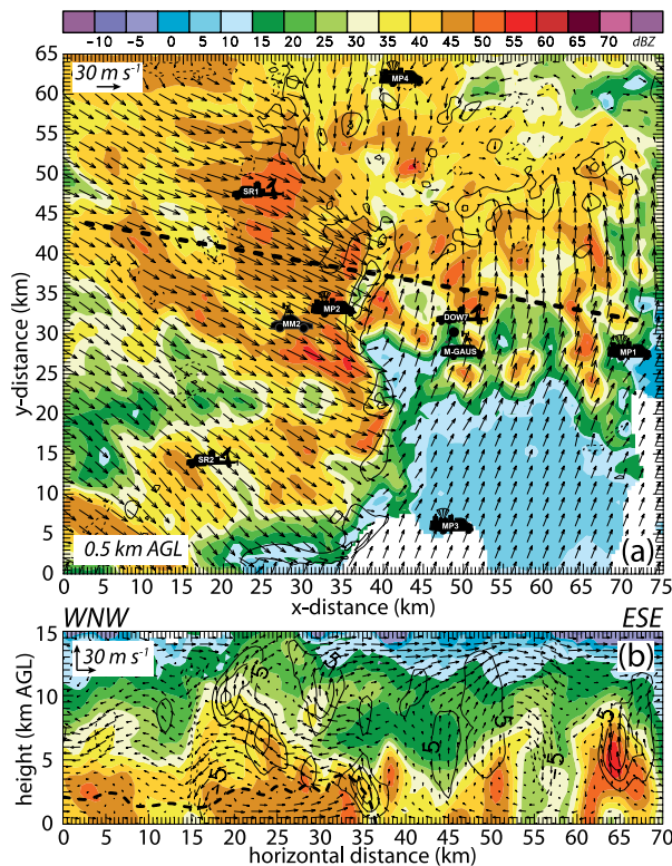
Fig. 5. Triple-Doppler analysis (combining SRI, SR2, and DOW7 mobile radar observations) of reflectivity (dBZ) and wind vectors at 0445 UTC 6 Jul 2015. (a) Horizontal section with ground-relative winds at 0.5 km AGL, within the inset box in Fig. 4 and (b) vertical cross section with MCS-relative winds along the dashed line in (a). Contours are updraft (solid) and downdraft (dashed) magnitudes and have the following contour interval and starting contour values, respectively: (a) 2 and \pm 2 m s -1 and (b) 5 and \pm 5 m s -1 . The locations of four mobile PISAs (MPI–4), three mobile radars, a mobile sounding unit (M-GAUS), and a mobile mesonet (MM2) are also shown in (a). The dashed curve in (b) is the estimated cold pool top based on thermal continuity principles (Ziegler 2013).
