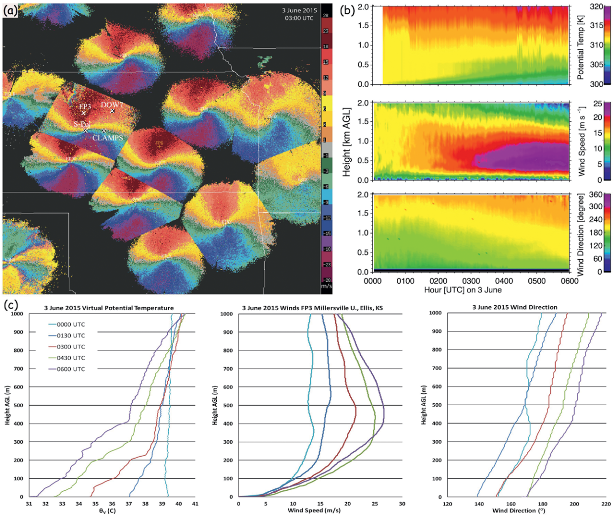
FIG. 11. (a) Mosaic base-elevation Doppler velocity field composed of the NEXRADs and S-Pol in the central Great Plains at 0300 UTC 3 Jun. (b) Time–height sections of virtual potential temperature \theta_v (from an AERI probe), wind speed, and wind direction (from a Doppler lidar) measured by CLAMPs [location shown in (a)], for 0000–0600 UTC on the same day. (c) Radiosonde profiles of \theta_v , wind speed, and direction in the 0–1-km AGL layer for the same period, at nearby FP3 [location shown in (a)].
