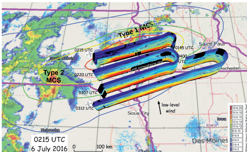
FIG. 7. 3D LASE water vapor distribution upstream of the MCS shown in Fig. 4. The LASE data were collected aboard the NASA DC-8 between 0145 and 0400 UTC 6 Jul, from a flight level of 8.5 km, descending to 6.7 km MSL on the last flight leg. The background image is NEXRAD composite base reflectivity at 0215 UTC. The colored closed contours are subjectively estimated probabilities of an MCS between 0300 and 0600 UTC, as produced by the PECAN field forecasters based on data available at 1600 UTC 5 Jul, ranging from low (outer blue contour) through moderate (inner green and yellow contours) to high (inner red contour). The black LASE sections lack data owing to lidar beam extinction by cloud.
