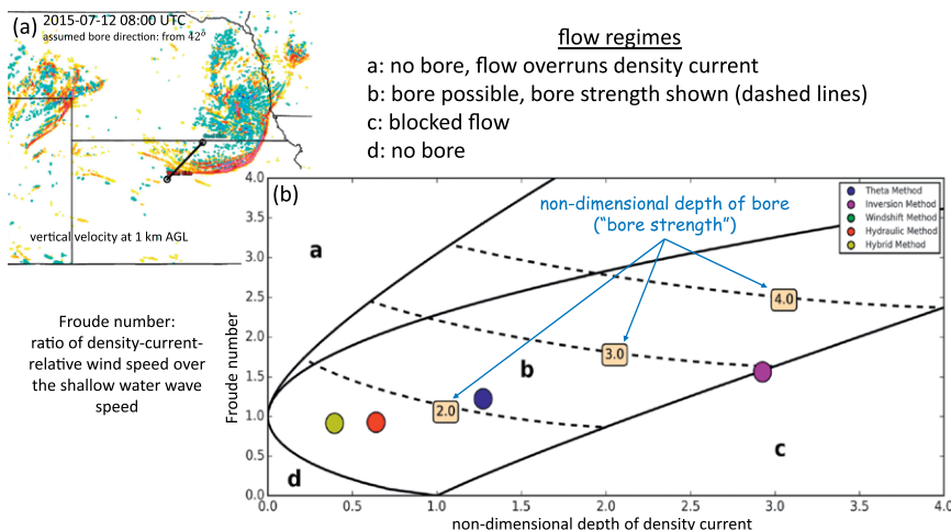
FIG. 8. Demonstration of the methodology behind forecasting atmospheric bores for a bore event on 12 Jul: (a) model vertical motion at 1 km AGL (red is positive, blue is negative) and (b) bore diagnostic tools calculated from values at the two user-selected end points shown in (a).
