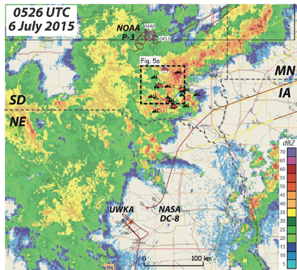
FIG. 4. Deployment of mobile radars, mesonet, and sounding vehicles, plus three aircraft at 0526 UTC 6 Jul 2015, as shown by the real-time Catalog Maps tool. The background map is NEXRAD composite base reflectivity. Aircraft tracks are in yellow, except for the most recent hour of flight, which is shown in red, and except for a section of the NOAA P-3 flight track shown in pink, during which hydrometeor observations shown in Fig. 6 were obtained. The dashed black box locates the domain shown in Fig. 5a.
