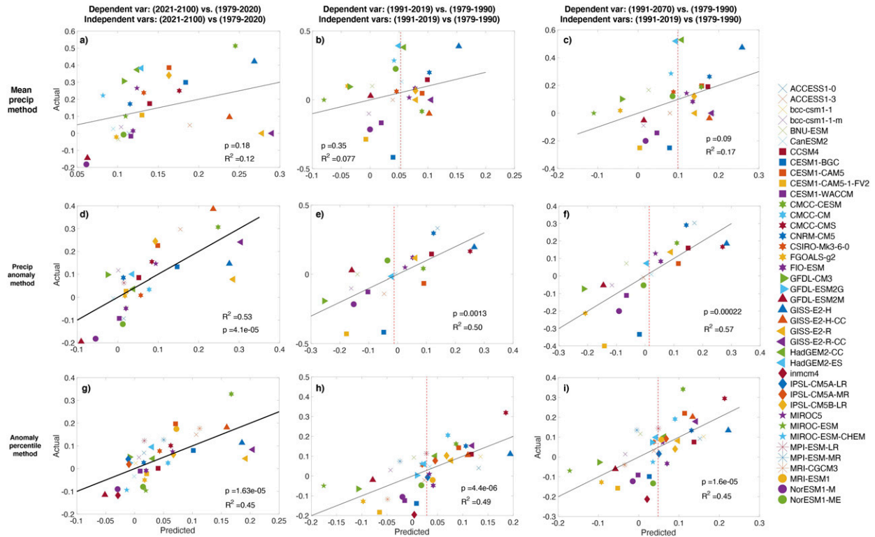
FIG. 13. Prediction of change in extreme El Niño fraction using observable metrics over the modern era: the zonal equatorial gradient of SST ( \Delta T/dx ), and the sensitivity of precipitation to SSTA ( \Delta P/dT ; regression of precipitation on SSTA over Niño-3). (a) Prediction of changes to extreme El Niño identified using the mean precipitation method, for both independent and dependent variable differences computed between 2021–2100 and 1979–2020. (b) As in (a), but for independent and dependent variables differenced between 2001–19 and 1979–2000. (c) As in (a), but for independent variables differenced between 2001–2019 and 1979–2000, and dependent variables differenced between 2001–2070 and 1979–2000. (d)–(f) As in (a)–(c), but for extreme El Niño events identified using the precipitation anomaly method. (g)–(i) As in (a)–(c), but for extreme El Niño events identified using the anomaly percentile method. Black solid lines indicate best-fit regressions; bold indicates a statistically significant relationship. Vertical red dashed lines indicate the predicted value generated using observational data.
