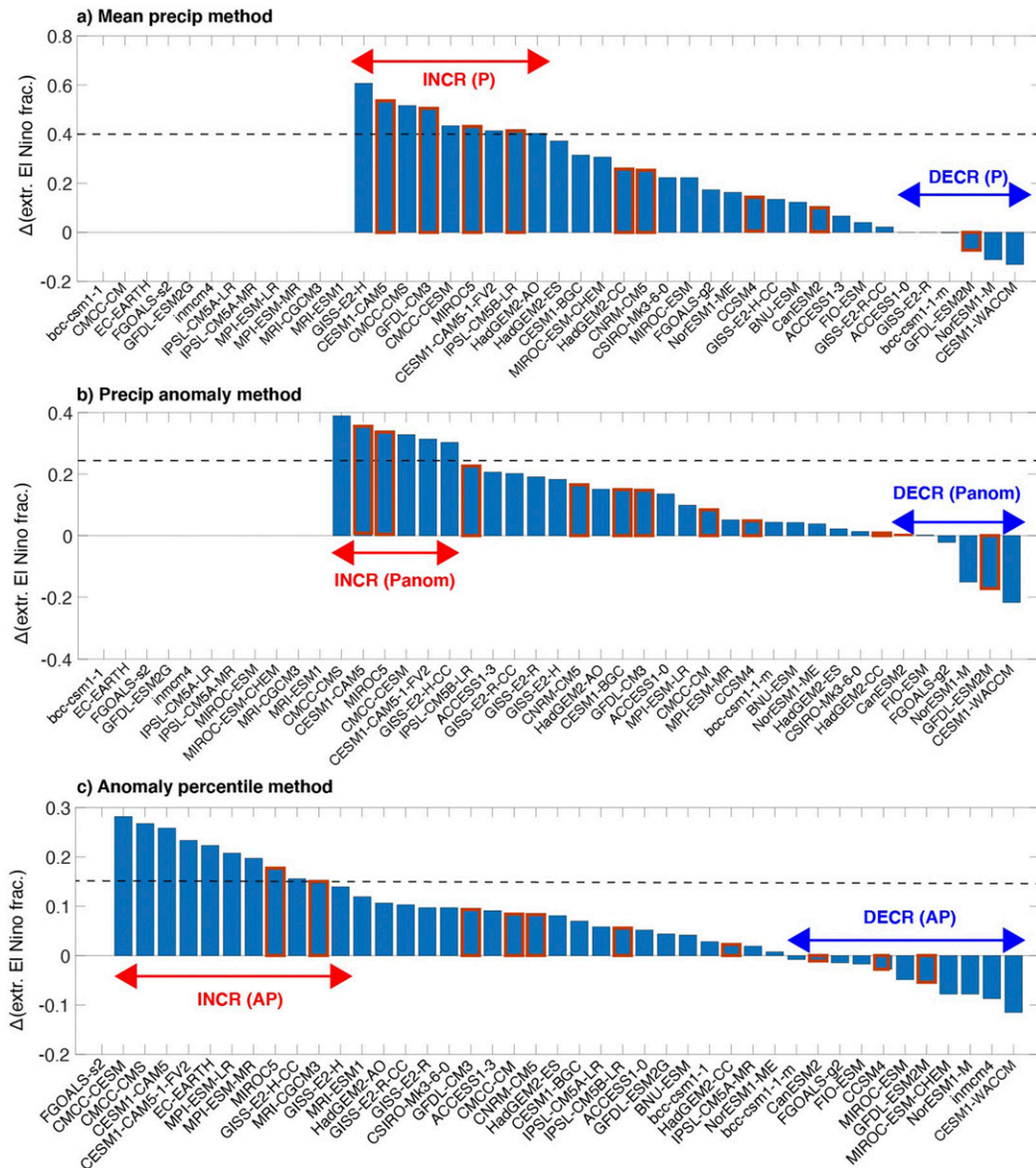
FIG. 3. Changes in proportion of extreme El Niño events over Niño-3, using the (a) absolute precipitation ( P ), (b) precipitation anomaly (Panom), and (c) anomaly percentile (AP) definitions. Red outlines indicate models selected by Cai et al. (2014) as having the capacity to best simulate El Niño rainfall and rainfall skewness. Dashed horizontal lines indicate thresholds used to select the INCR subsets of models according to all three definitions. In (a) and (b), fewer models are included since the absolute precipitation or precipitation anomaly for some models fell below the appropriate threshold for all El Niño events. Models with larger overall precipitation variability will tend to show smaller changes in (c), since the percentile changes will tend to be smaller.
