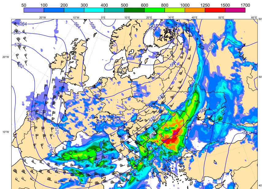
FIG. 10. ECMWF analysis at 1200 UTC 18 Jun 2016. Blue solid lines depict isohypses (dam) of geopotential height at 500 hPa. CAPE–shear values above 50 \text{ m}^2 \text{ s}^{-2} are shaded. Flags represent 200-hPa winds above 30 \text{ m s}^{-1} .
