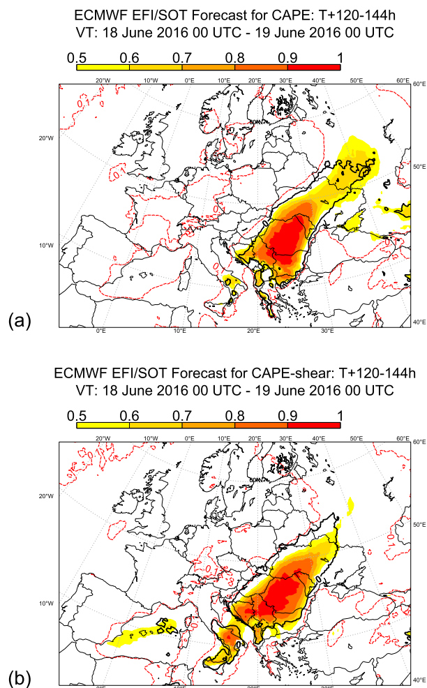
FIG. 12. ECMWF EFI/SOT T + 120 – 144 -h forecasts for (a) CAPE and (b) CAPE–shear. Dashed red line represents EFI of 0.1. The values of the EFI above 0.5 are shaded. The solid black line is the SOT zero line enclosing positive SOT values.
