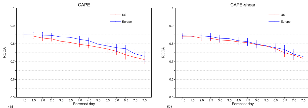
FIG. 3. ROCA skill score comparison between Europe and the United States for (a) EFI CAPE and PoP and (b) EFI CAPES and PoP. Damaging lightning and heavy precipitation reports from ESWD have been included in the verification dataset for Europe. Error bars denote 90% confidence intervals drawn from a bootstrap resampling technique with 1000 random samples.
