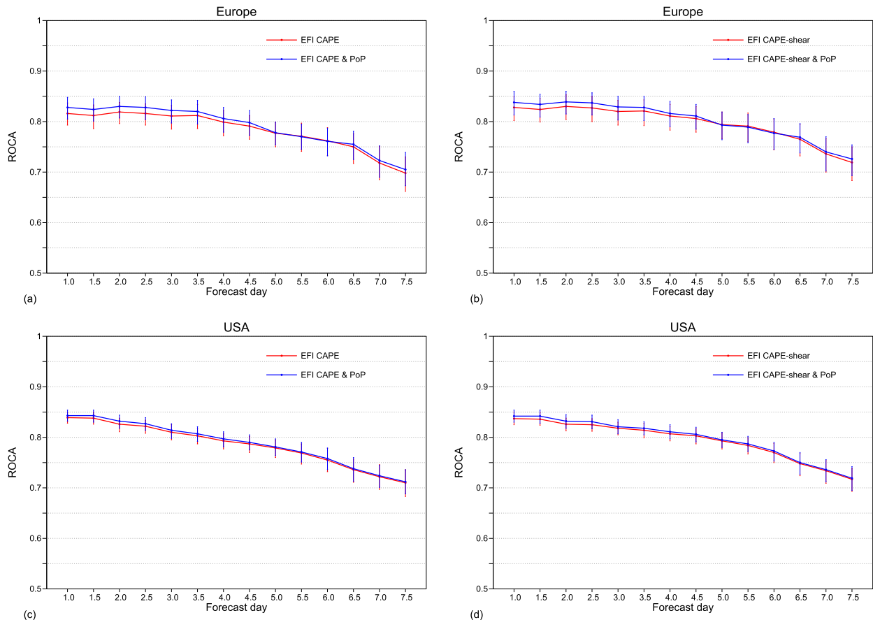
FIG. 2. ROCA comparison between the EFI only and the EFI-PoP for (a) CAPE over Europe, (b) CAPES over Europe, (c) CAPE over the United States and (d) CAPES over the United States. Reports of tornadoes, large hail, and strong wind gusts (wind gust reports flagged as nonconvective have been filtered out) are retained from ESWD for the best compatibility between the ESWD and SPC datasets of severe weather reports. A threshold of 5% is chosen for PoP. Error bars denote 90% confidence intervals drawn from a bootstrap resampling technique with 1000 random samples.
