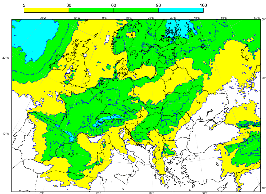
FIG. 13. ECMWF PoP for >1 \text{ mm (24 h)}^{-1} T + 120\text{--}144\text{-h} forecast. Here, \text{PoP} > 5\% is shaded with lines representing the 5%, 30%, 60%, and 90% probabilities.
