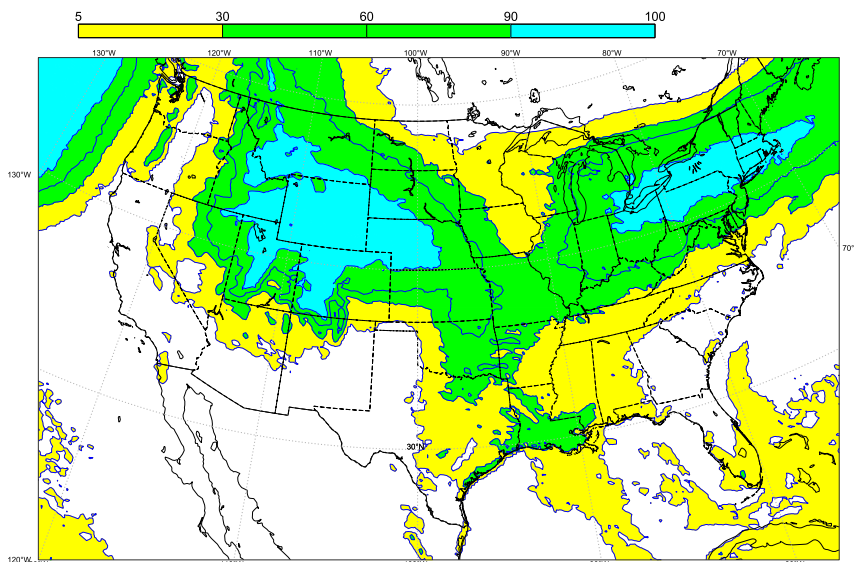
FIG. 8. ECMWF PoP for >1 \text{ mm (24 h)}^{-1} T + 96\text{--}120\text{-h} forecast. Here, PoP > 5\% is shaded with lines representing the 5%, 30%, 60%, and 90% probabilities.
