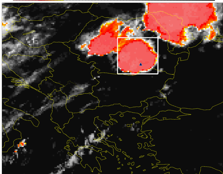
FIG. 14. (a) Sounding for Bucharest, Romania, at 1200 UTC 18 Jun 2016 and (b) Meteosat IR 10.8- \mu\text{m} satellite imagery at 2000 UTC 18 Jun 2016. A supercellular thunderstorm that produced large hail up to 5–6 cm according to the ESWD reports is shown inside the white rectangle. The triangle symbol within the rectangle denotes the location of the sounding in Bucharest shown in (a).
