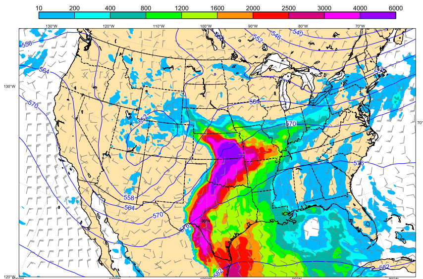
FIG. 5. ECMWF analysis at 1200 UTC 26 Apr 2016. Thick solid lines depict isohypses (dam) of geopotential height at 500 hPa. Shading represents CAPE ( J\ kg^{-1} ). Gray flags depict 10-m winds.
