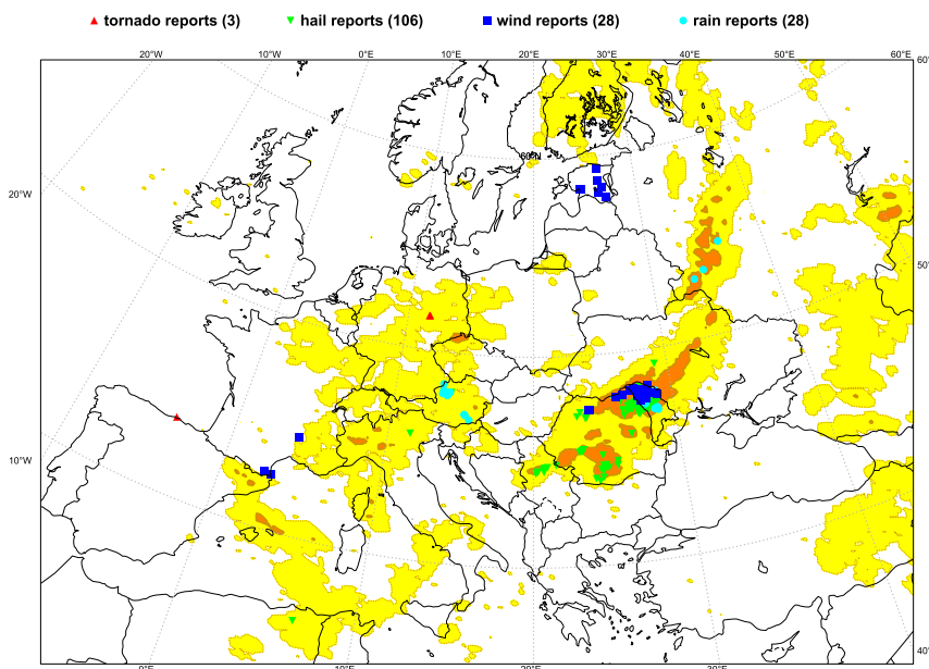
FIG. 11. ESWD reports (symbols) and ATDnet lightning activity (shading). The shading in orange denotes intense lightning activity above 0.2 \text{ flashes km}^{-2} (24 \text{ h})^{-1} .
