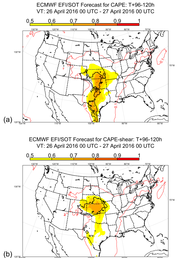
FIG. 7. ECMWF EFI/SOT T + 96 – 120 -h forecasts for (a) CAPE and (b) CAPE–shear. Dashed red line represents EFI of 0.1. Values of EFI above 0.5 are shaded. The solid black line is the SOT zero line enclosing positive SOT values.
