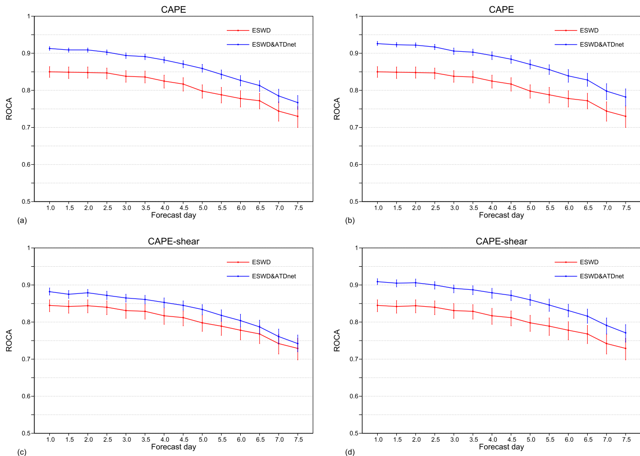
FIG. 4. ROCA comparison for Europe between datasets containing severe weather reports from ESWD only and a combination of ESWD reports and ATDnet lightning data for (a) EFI for CAPE with a lightning activity threshold of 0.2 \text{ flashes km}^{-2} (24 \text{ h})^{-1} , (b) EFI for CAPE with a lightning activity threshold of 0.5 \text{ flashes km}^{-2} (24 \text{ h})^{-1} , (c) EFI for CAPES with a lightning activity threshold of 0.2 \text{ flashes km}^{-2} (24 \text{ h})^{-1} , and (d) EFI for CAPES with a lightning activity threshold of 0.5 \text{ flashes km}^{-2} (24 \text{ h})^{-1} . ESWD reports include tornadoes, large hail, severe wind gusts, damaging lightning, and heavy convective rain. Error bars denote 90% confidence intervals drawn from a bootstrap resampling technique with 1000 random samples.
