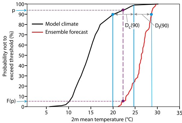
FIG. 1. CDFs of the M-climate (black curve) and real-time ENS (red curve) for 2-m mean temperature. The M-climate percentile p and ENS percentile F(p) are shown, with the vertical dashed line representing the difference [p - F(p)] in the EFI definition. Differences D_f(90) = P_c(99) - P_f(90) and D_c(90) = P_c(99) - P_c(90) define the SOT, where P_f(90) is the 90th percentile of the real-time ENS distribution, and P_c(90) and P_c(99) are the 90th and 99th percentiles of the M-climate distribution, respectively.
