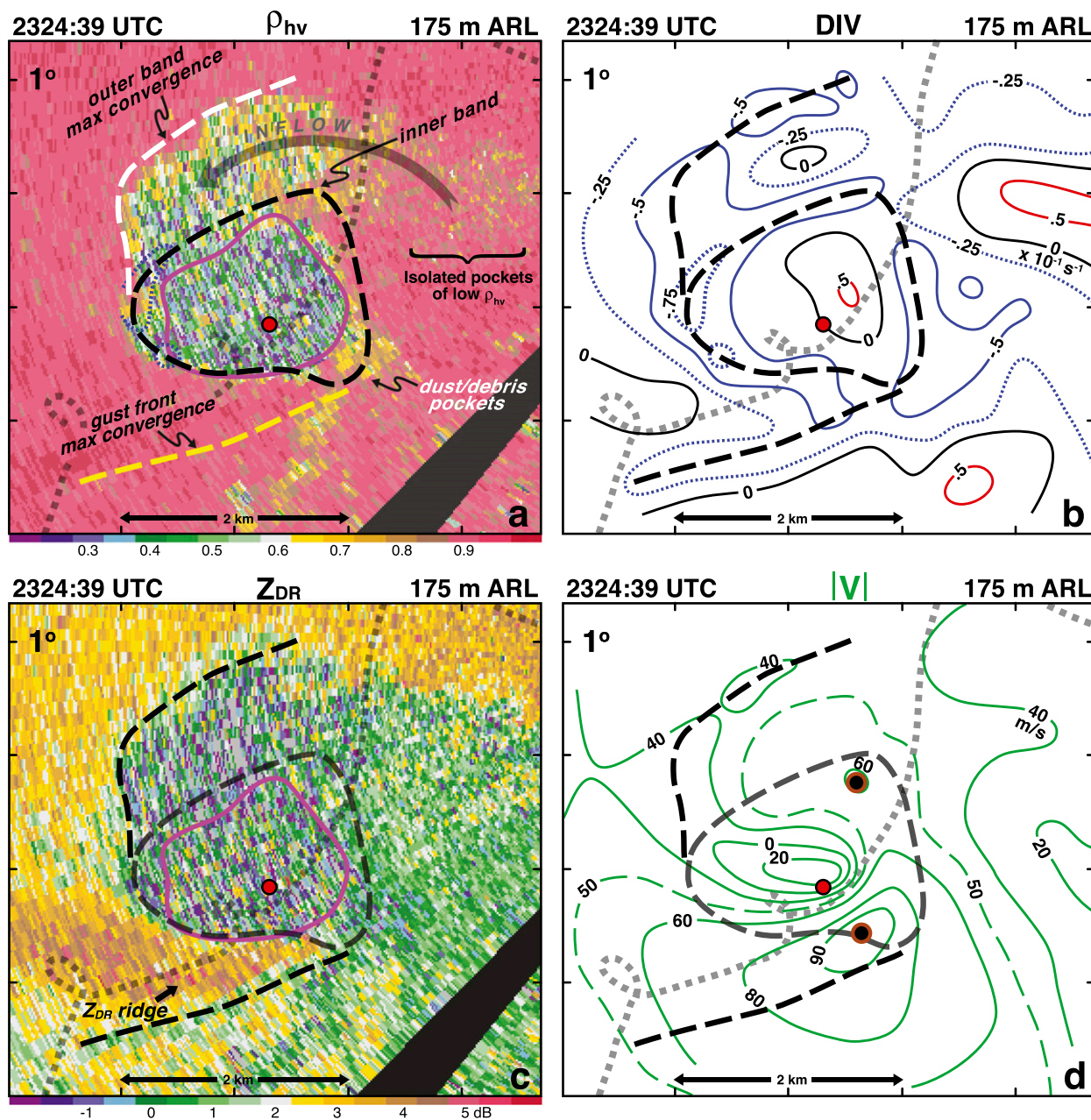
FIG. 19. (a) The \rho_{hv} at 2324:39 UTC ( 1^\circ elevation angle) from RaXPoL. The long, dashed lines (white, black, and yellow) represent zones of maximum low-level convergence. The 1 \times 10^{-1} \text{ s}^{-1} isopleth of vertical vorticity is drawn as a magenta line. (b) Low-level divergence fields ( \times 10^{-1} \text{ s}^{-1} ). Divergence and convergence isopleths are drawn as red and blues lines, respectively. The -0.25 and -0.75 \times 10^{-1} \text{ s}^{-1} isopleths of convergence have been added as dashed blue lines. The long, dashed lines represent zones of maximum low-level convergence. (c) The Z_{DR} at 2324:39 UTC ( 1^\circ elevation angle) from RaXPoL. The long, dashed lines represent zones of maximum low-level convergence. The 1 \times 10^{-1} \text{ s}^{-1} isopleth of vertical vorticity is drawn as a magenta line. (d) Magnitude of the ground-relative wind field. Isopleths of the wind speed are drawn as green lines. The 50 \text{ m s}^{-1} isopleth of wind speed has been added as a dashed green line. The brown circles in (d) denote the location of the maximum speed. The red dot is the final location of a storm chaser car that resulted in fatalities and is shown on all panels. Area shown in the figure is depicted in Fig. 2.
