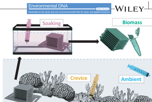
FIGURE 1 The four methods used in the DNA metabarcoding of cryptic coral reef habitat: biomass (accumulated biomass from ARMS fractions, pooled by unit, n = 6 ), soaking (aqueous DNA collected from soaking ARMS units in seawater aquaria, n = 6 ), crevices (eDNA collected from within reef crevices, n = 12 ), and ambient (eDNA from surface seawater collected from the back reef, n = 6 )
