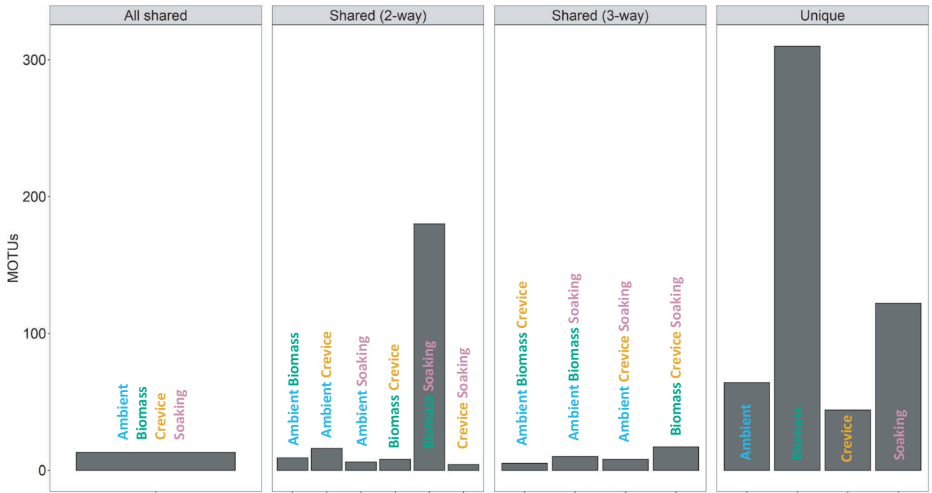
FIGURE 4 Total shared and unique metazoan and macroalgal molecular operational taxonomic units (MOTUs) detected by each sampling method (biomass, soaking, crevice, and ambient), identified using the five reference sequence databases
