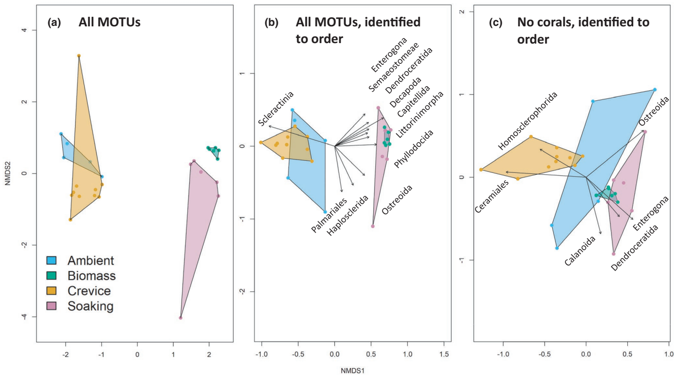
FIGURE 5 (a) Non-metric multidimensional scaling (NMDS, Bray–Curtis dissimilarity, relative abundance \geq 0.01\% ) of all metazoan and macroalgal molecular operational taxonomic units (MOTUs) from cryptic habitat communities. (b) NMDS (Bray–Curtis dissimilarity, relative abundance \geq 0.01\% ) of MOTUs identified to order level using the five reference sequence databases. (c) NMDS (Bray–Curtis dissimilarity, relative abundance \geq 0.01\% ) of MOTUs identified to order level, but with order Scleractinia removed. The direction and length of vectors are proportional to the degree of correlation as determined by the envfit function (permutations = 9999, p_{max} = 0.05 , Tables S4 and S5) in the vegan package (Oksanen et al., 2013). One ambient sample was dropped, as it did not contain any metazoan or macroalgal MOTUs
