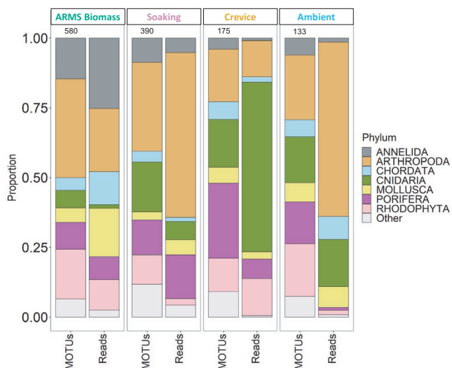
FIGURE 2 Proportional number of metazoan and macroalgal molecular operational taxonomic units (MOTUs, totals marked above each method) and DNA reads detected by each sampling method (biomass, soaking, crevice, and ambient) that were identified to the phylum level using the five reference sequence databases. Phyla that had <1.0% relative abundance (Echinodermata, Nemertea, Nematoda, Ochrophyta, Chlorophyta, Platyhelminthes, Gastrotricha, Xenacoelomorpha, Bryozoa, Rotifera, and Entoprocta) were grouped as “Other”
