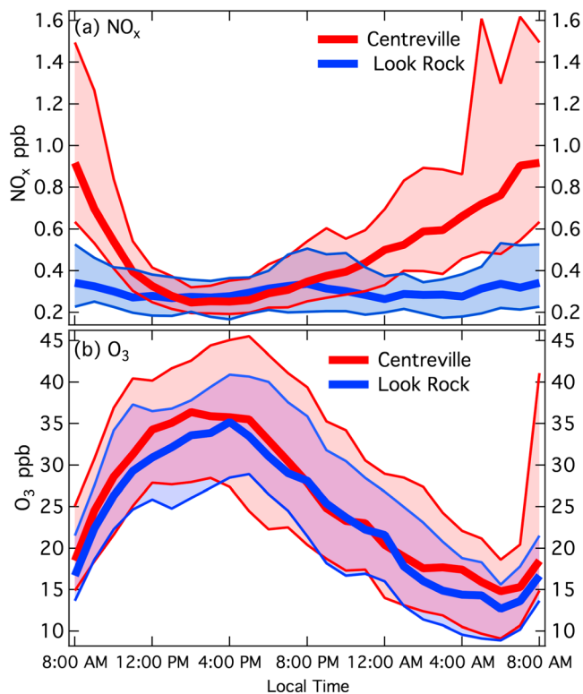
Figure 4. Diurnal plot of (a) \text{NO}_x and (b) \text{O}_3 at both sites. Medians, 25th percentiles, and 75 percentiles are shown on the figure.
