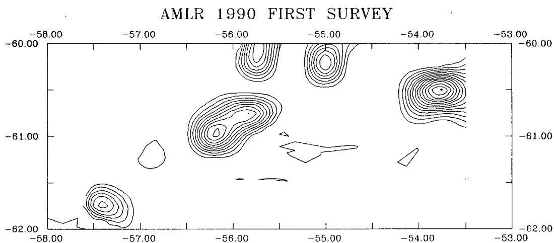
Figure 3.3 AMLR 1990 Survey 1 contour plot of the biomass distribution.
