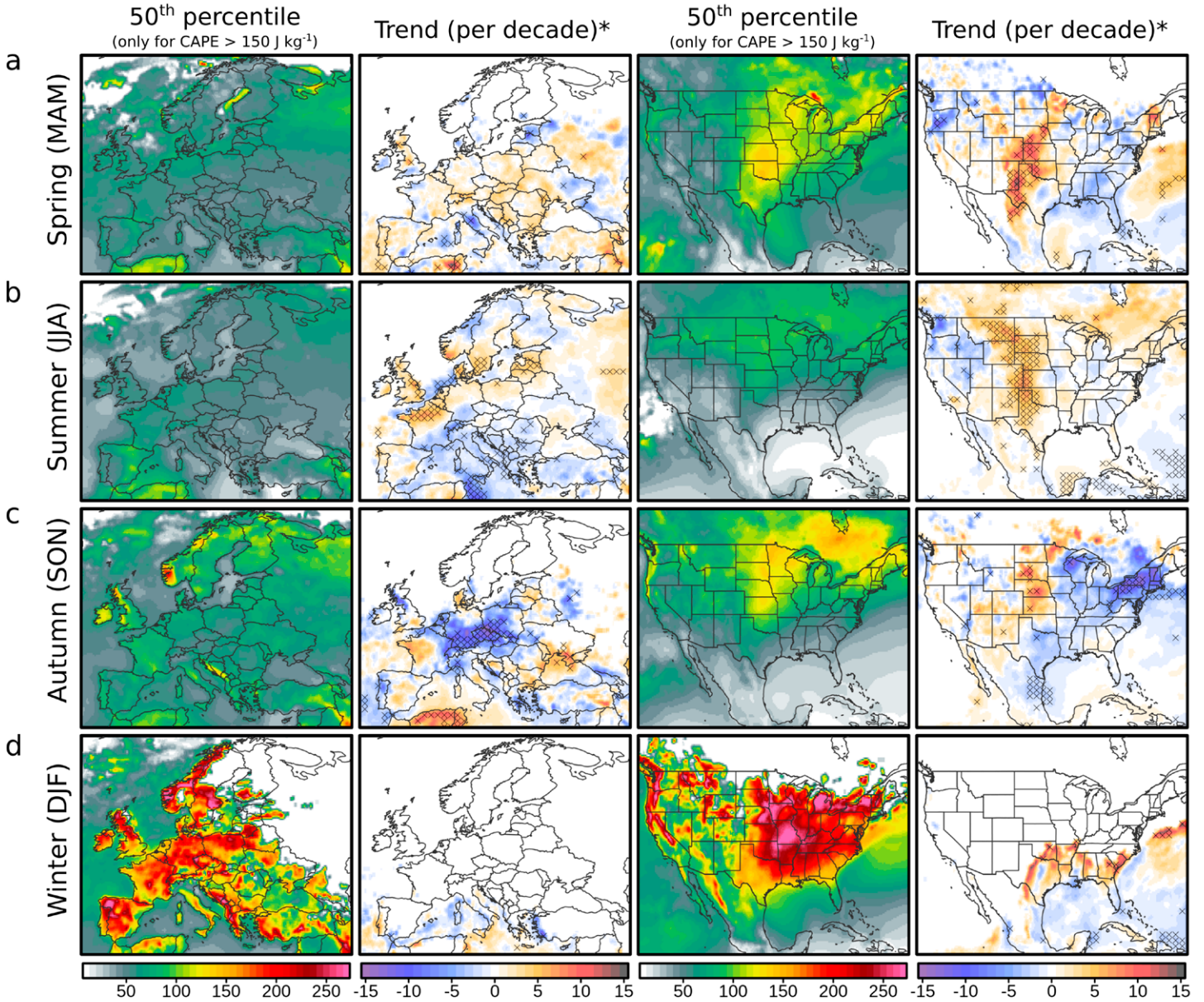
Fig. E1. As in Fig. 2d, but for seasons.
