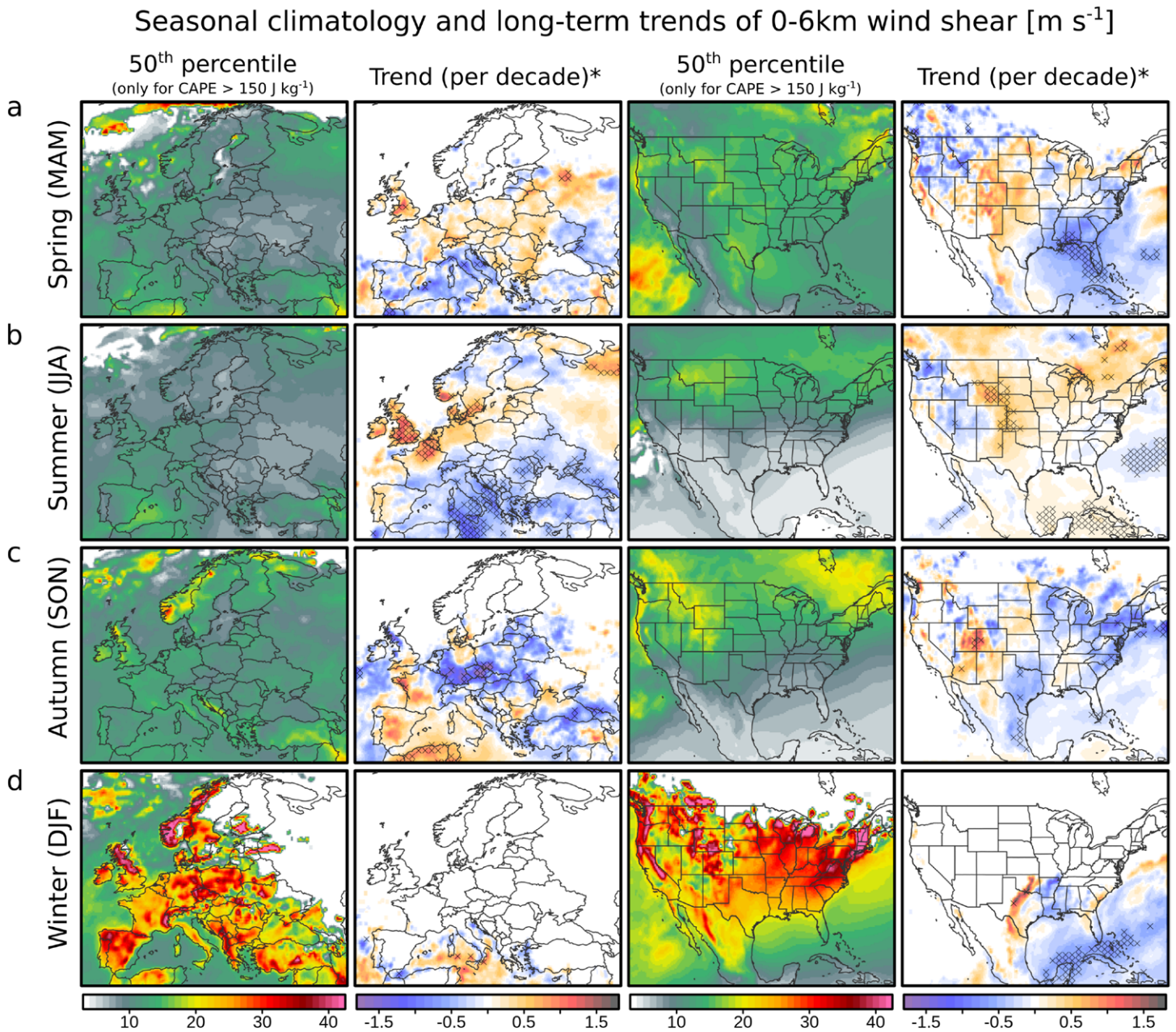
Fig. D1. As in Fig. 2c, but for seasons.
