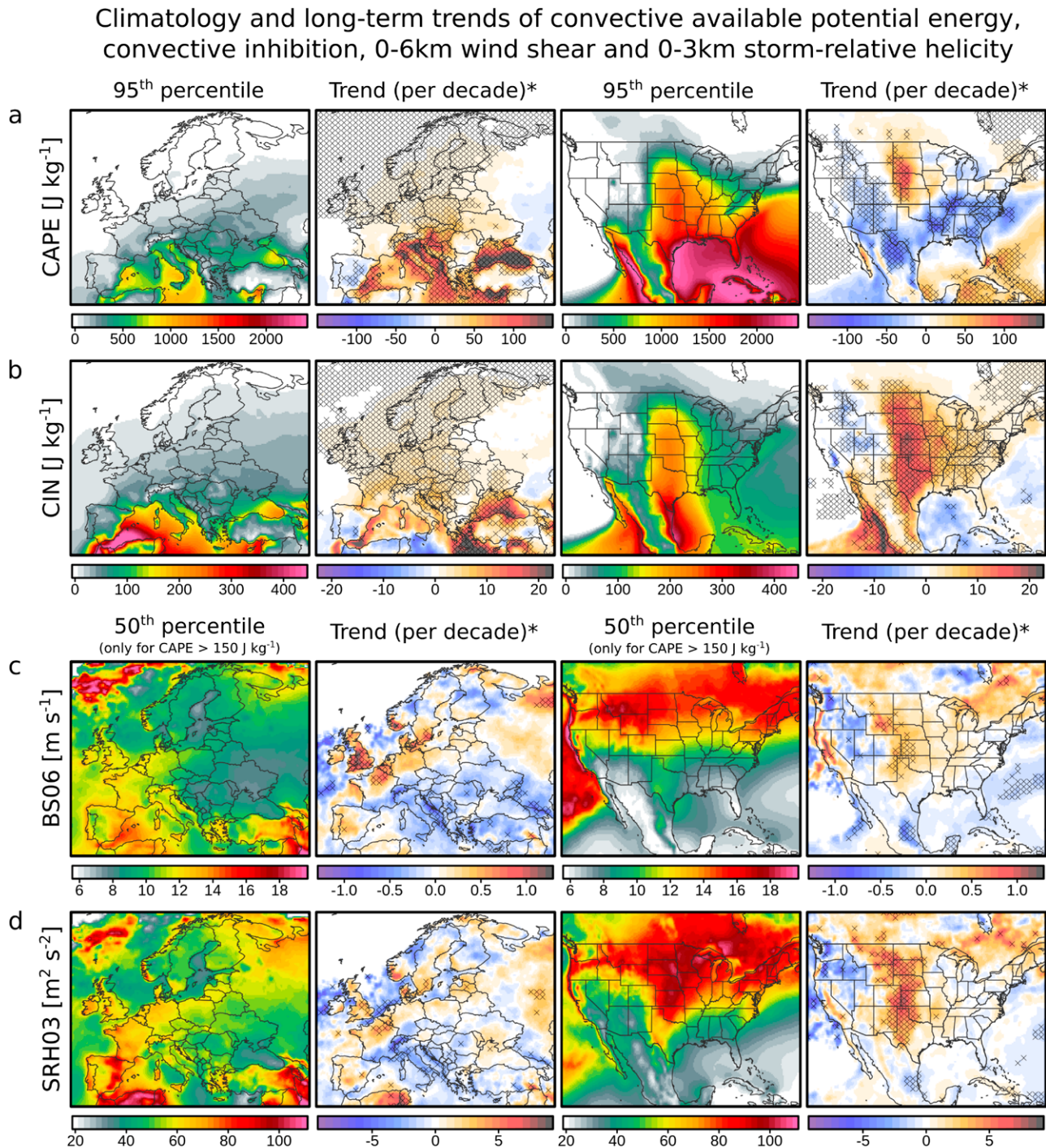
Fig. 2. As in Fig. 1, but for the 95th percentile of (a) convective available potential energy (CAPE), (b) absolute value of convective inhibition (CIN), and (c) 50th percentile of vertical wind shear (BS06) and (d) storm-relative helicity (SRH03). For BS06 and SRH03 only situations with CAPE > 150\text{ J kg}^{-1} are considered.
