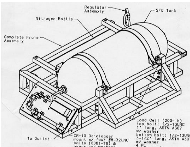
Figure 5. Aircraft dissemination system mounting frame.
