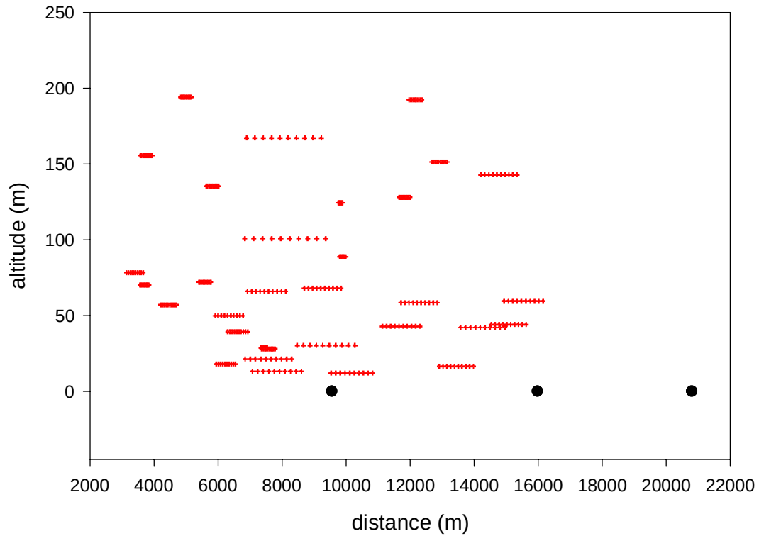
Figure I1. Test 11 continuous analyzer data. Altitude versus downwind distance. The red crosses are aircraft measurements. The black circles are the positions of sampling Lines 1, 2, and 3. The width is \pm 1\sigma from the position of peak concentration.
