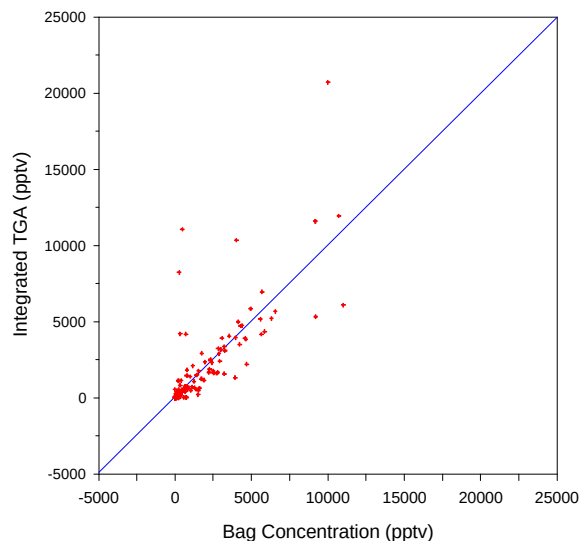
Figure 20. Integrated \text{SF}_6 concentration from continuous analyzers versus sample concentration from whole air samplers for all tests. The line is a fit to the data with an equation of y = (0.99 \pm 0.05)x + (112 \pm 135) , r^2 = 0.64 , N = 189 .
