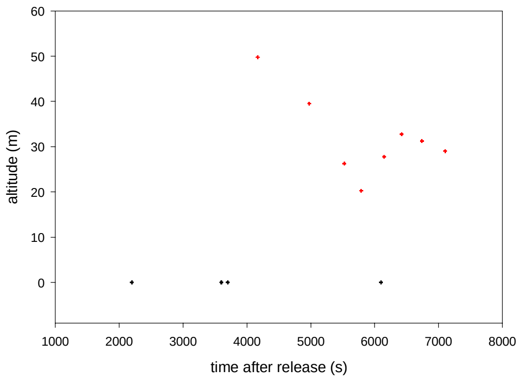
Figure B4. Test 1 continuous analyzer data. Altitude versus time after release. The red crosses are aircraft measurements. The black crosses are ground measurements at sampling Lines 1 and 2.
