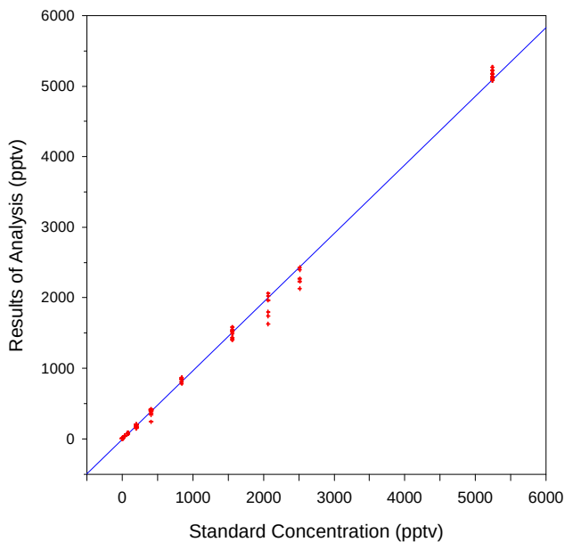
Figure 11. Results of the analysis of 127 spiked samples versus the concentration of the standards. The solid line is a linear fit to the data: y = (0.97 \pm 0.004)x + (13 \pm 7) , r^2 = 0.997 , N = 127 .
