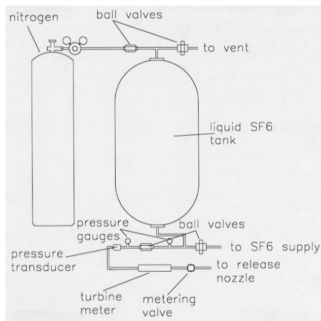
Figure 6. Components of the aircraft dissemination system.
