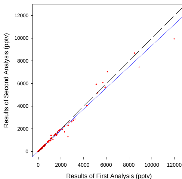
Figure 9. Comparison of reanalysis of samples. The solid line is a linear fit to the data: y = (0.93 \pm 0.01)x + (9 \pm 10) , r^2 = 0.98 , N = 205 . The dashed line is y = x .
