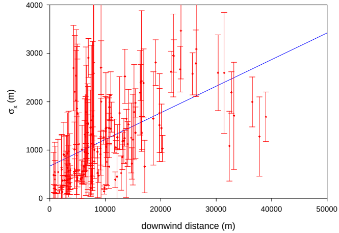
Figure 17. \sigma_x versus x . The data plotted are from the aircraft-based continuous analyzer. The solid line is a linear fit to the data with the equation \sigma_x = (0.05 \pm 0.006) x + (670 \pm 85) and a correlation coefficient of r^2 = 0.3 , N = 157 .
