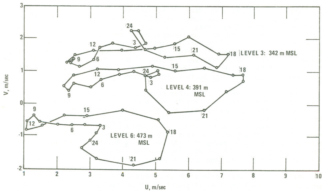
Figure 24. Average horizontal wind hodographs, Mt. Sutro Tower, September, 1974.
