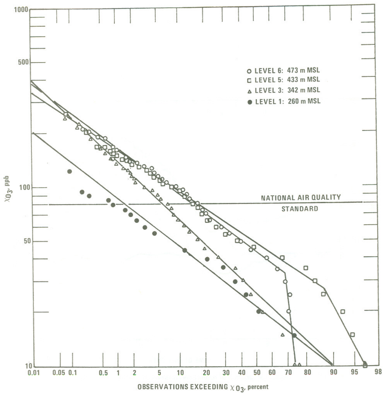
Figure 20. Cumulative frequency distribution of ozone concentrations, Mt. Sutro Tower, June 24 - September 24, 1974.
