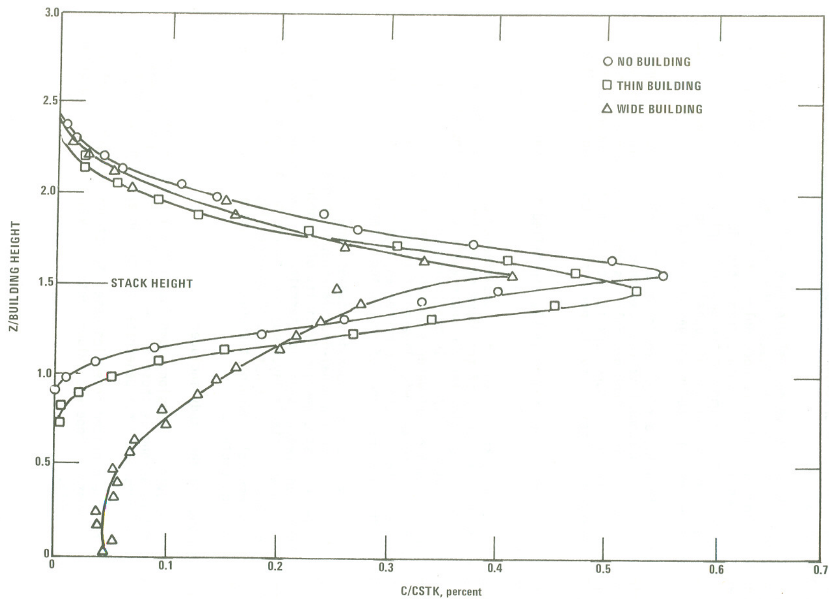
Figure 12. Influence of building on plume behavior. Stack height is 1.5 times the building height. Vertical concentration profiles taken 3 building heights downwind.
