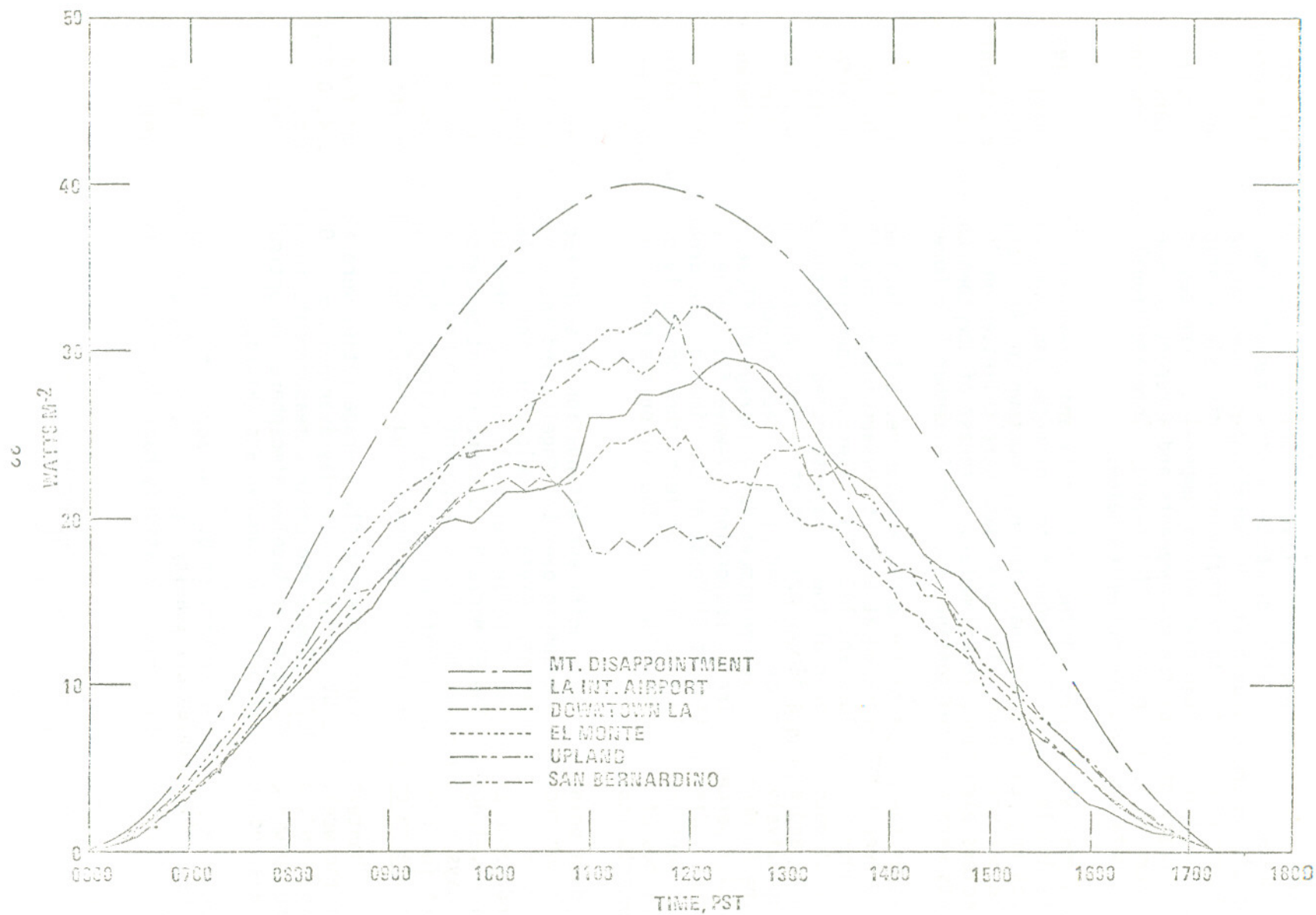
Figure 3. Measured ultraviolet flux (watts m -2 ) at five urban sites and one rural (Mt. Disappointment) site near Los Angeles during October 25, 1973.
