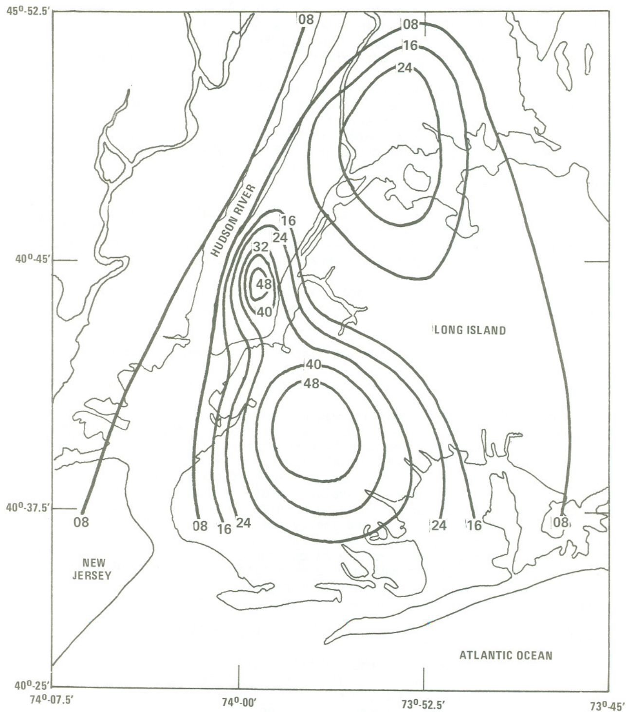
Figure 2. Example of \text{SO}_2 concentration (pphm) analysis for 1030 EST, December 6, 1966.
