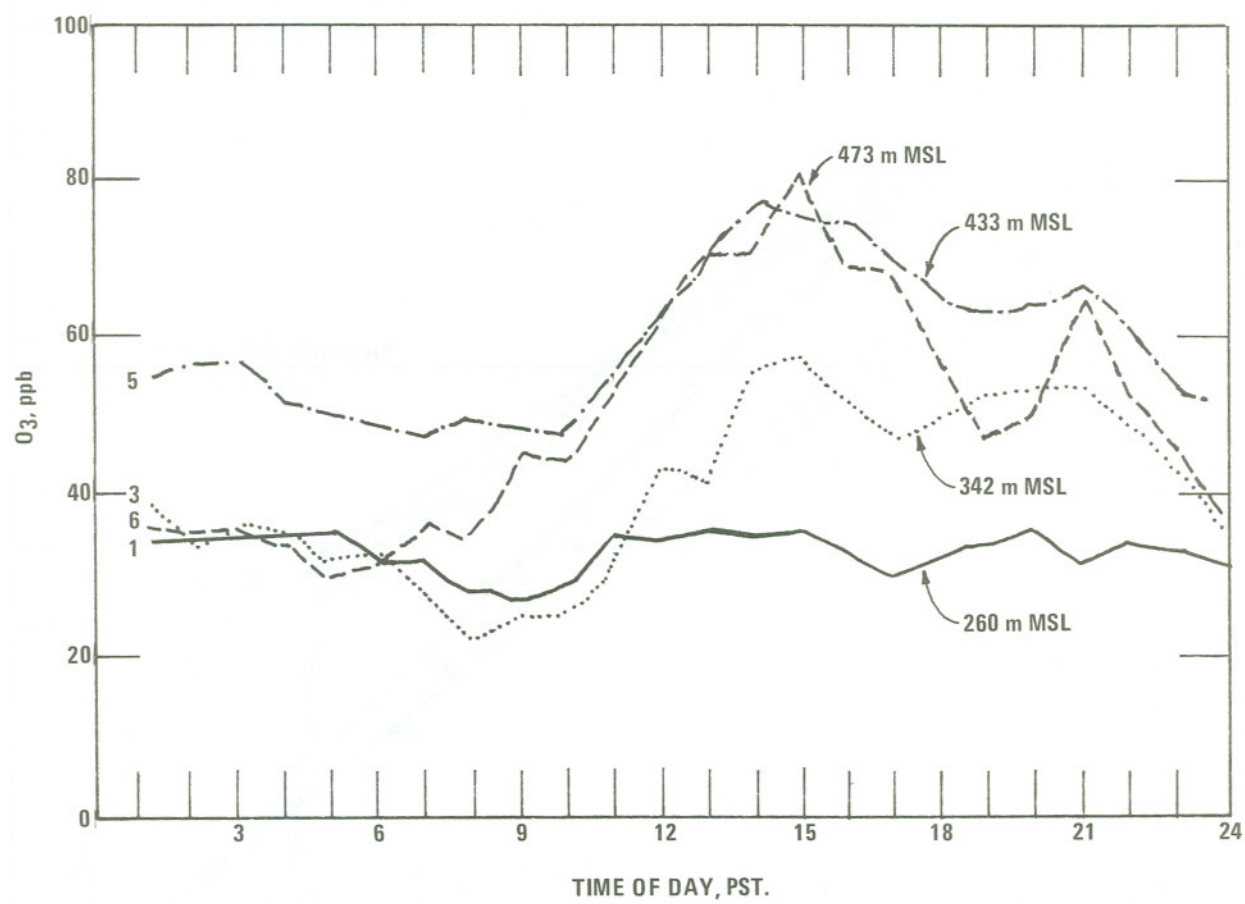
Figure 21. Average diurnal variation of ozone concentration, Mt. Sutro Tower, September, 1974.
