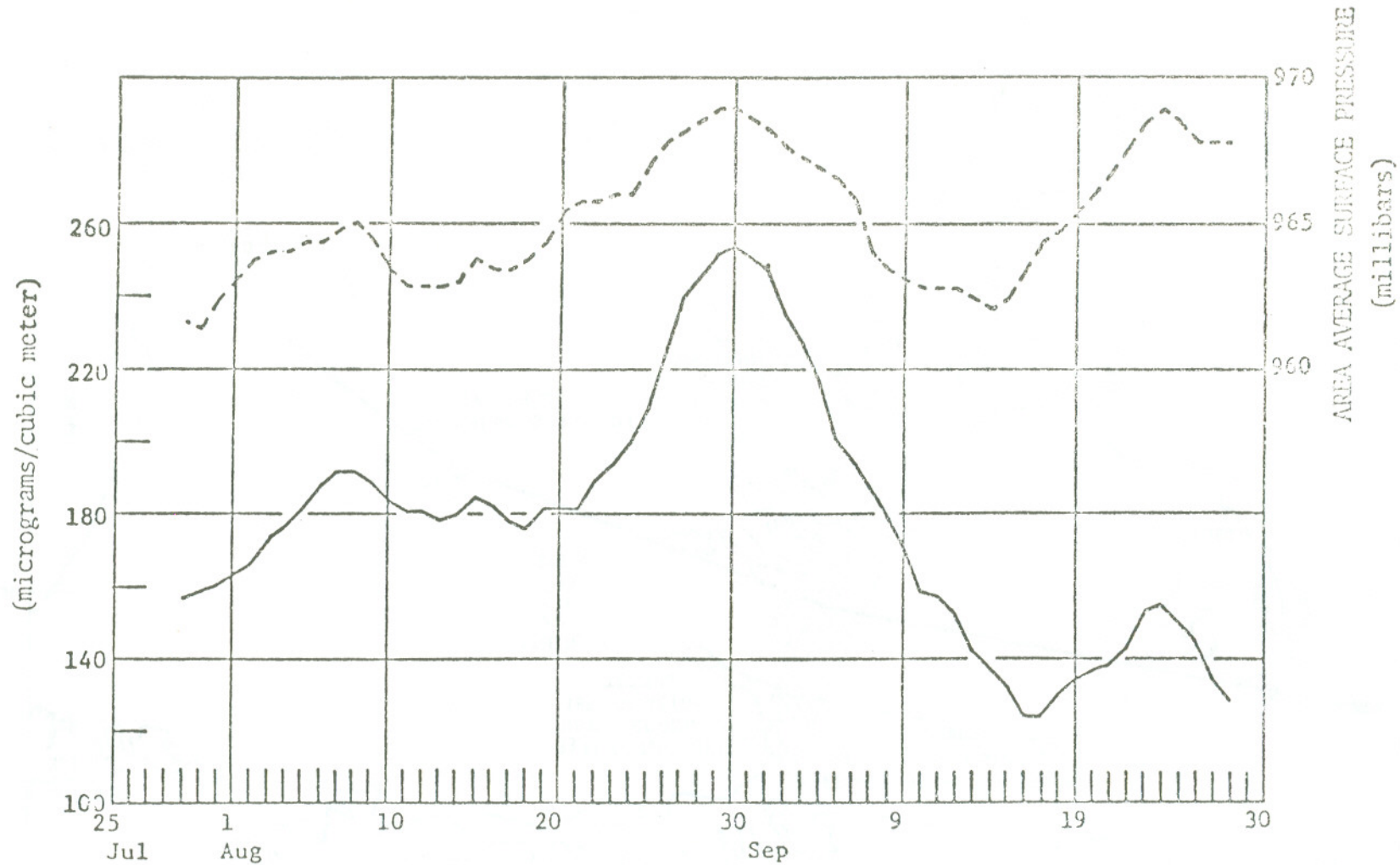
Figure 25. Smoothed variations of area average daily ozone - surface pressure, 1973 time sequence.
