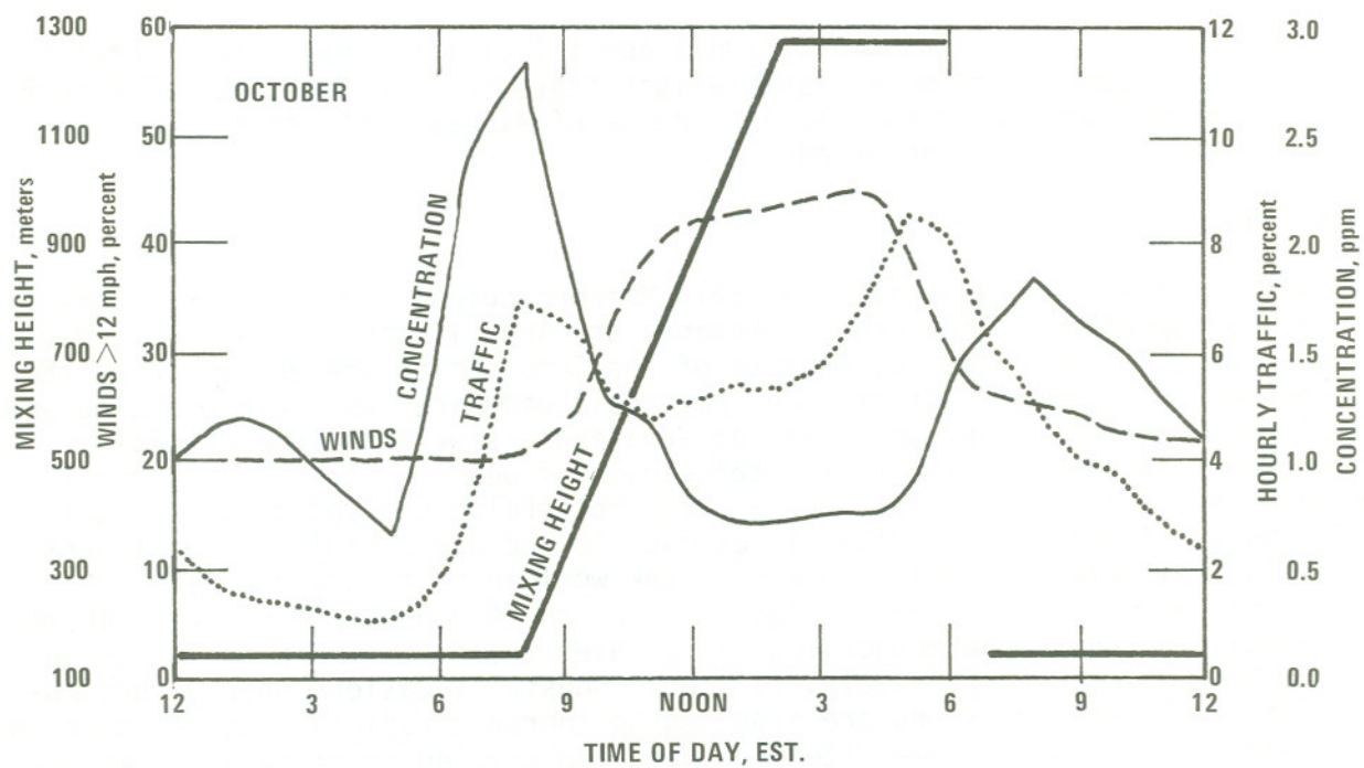
Figure 15. Diurnal variations of mixing heights, frequency of wind speeds greater than 12 mph, traffic flow and CO concentrations (hourly data plotted at hour ending time - eastern standard).
