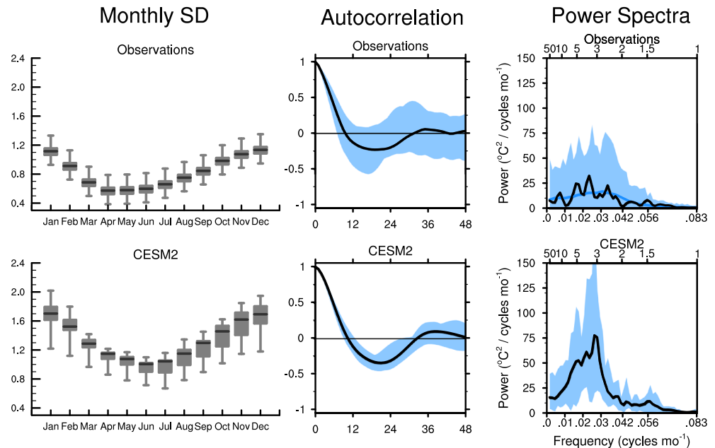
Figure 4. Monthly standard deviation (left panels), autocorrelation function (middle panels), and power spectra (right panels) of the detrended Niño-3.4 index during 1958–2014 for observations (ERSSTv5, top panels) and CESM2 historical simulations (bottom panels). The range of estimates for the CESM2 autocorrelation function and spectrum (light blue shading) are estimated using the 11-member ensemble of the CESM2 historical simulations, while the observational uncertainties are based on a 28,500-year LIM integration, yielding five hundred 57-year segments that are consistent with the statistics of the 1958–2014 period used to train the LIM. The statistics of the monthly standard deviations in the left panels are summarized through the use of boxplots and whiskers as in Figure 3. The blue curve in the top-right panel shows the average spectrum of the five hundred 57-year segments of the LIM output. Note the different vertical axes of the left and right panels between Figures 3 and 4.
