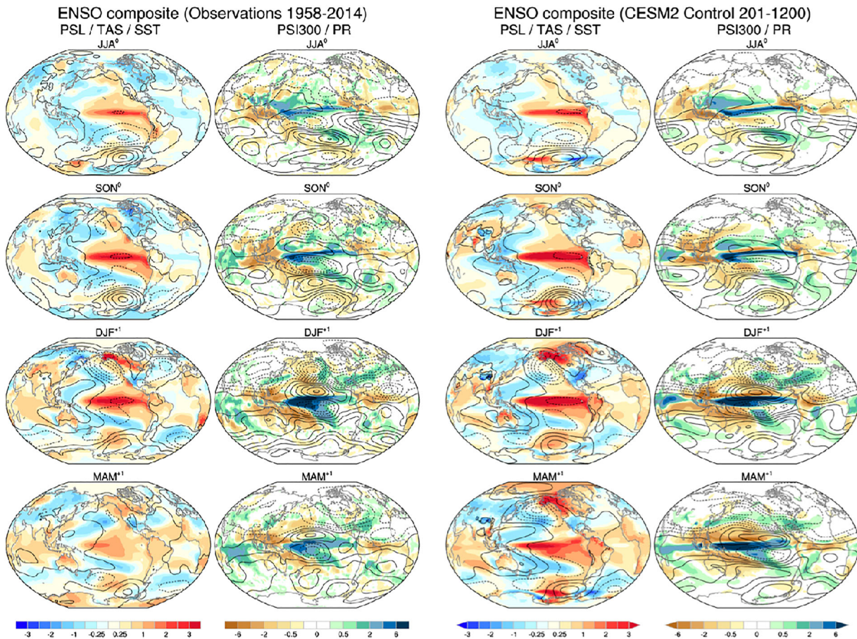
Figure 15. ENSO composite (positive minus negative) seasonal evolution from (top) JJA (year 0) through (bottom) MAM (year + 1) based on observations (left pair of columns) and CESM2 piControl (right pair of columns). The left column of each pair shows SST and terrestrial near-surface air temperature (color shading) and SLP (contours, negative values dashed, and contour interval of 2 hPa), and the right column of each pair shows precipitation ( \text{mm day}^{-1} ; color shading) and 300 hPa stream function (contours, negative values dashed, and contour interval of 3 \times 10^6 \text{ m}^2 \text{ s}^{-1} ) anomalies. The observed composite is based on years 1958–2014 except for precipitation and 300-hPa stream function which are for 1979–2014. The CESM2 composite is based on model years 201–1,200. See text for details.
