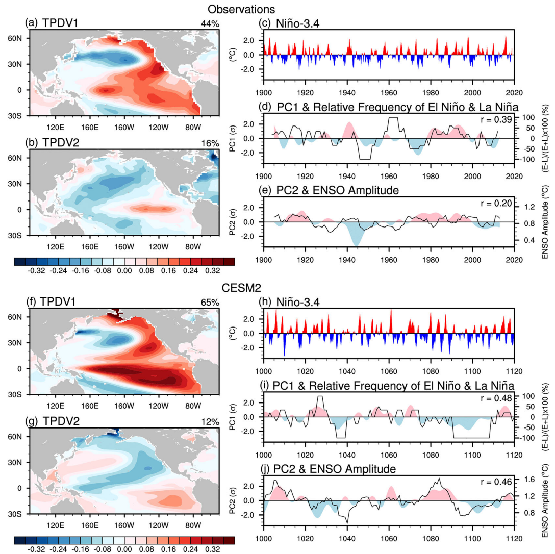
Figure 18. TPDV and ENSO modulations in (a–e) observations (ERSSTv5 over 1900–2018) and (f–j) CESM2 (model years 201–1,200). (a) SST anomaly pattern associated with TPDV1 obtained by regressing SST anomalies onto the standardized PC1 of 10-year low-pass-filtered SST variability in the tropical Pacific (23.5°S to 23.5°N, 120°E to 80°W). The fraction of total decadal variance explained by this mode is indicated in the top right. (b) As in (a) but for TPDV2. (c) Time series of the monthly Niño-3.4 index smoothed with a 3-month binomial filter (°C). (d) Time series of PC1 (standard deviation units; shaded curve) and the relative frequency of El Niño and La Niña events (%; black curve) defined as (E - L)/(E + L) \times 100 , where E and L are the numbers of El Niño and La Niña events in a moving 10-year window, respectively. El Niño and La Niña events are defined as in Figures 6 and 7, although consecutive El Niño or La Niña years are counted separately. The correlation coefficient of these time series is indicated in the upper right. (e) as in (d) but for PC2 and the ENSO amplitude (°C) defined as standard deviation of the Niño-3.4 index in a moving 10-year window. (f–j) As in (a)–(e) but for CESM2. Both observed and CESM2 SST data are linearly detrended prior to the analysis.
