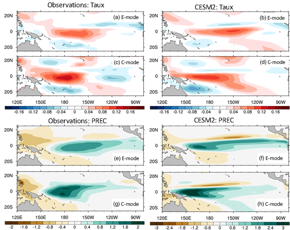
Figure 14. Patterns of anomalous zonal wind stress (a–d) and precipitation (e–h) associated with the E and C modes for observations (left) and CESM2 (right). The patterns are obtained by linearly regressing the zonal wind stress and precipitation anomalies on the E and C indices. The zonal wind stress ( \text{N/m}^2 ) is from the NCEP/DOE reanalysis, and precipitation ( \text{mm/day} ) is from the NOAA precipitation reconstruction data set.
