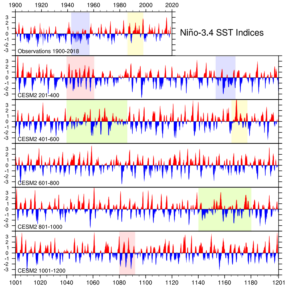
Figure 2. Time series of the monthly Niño-3.4 index for ERSSTv5 over the 1900–2018 period (top panel) and for CESM2, from model year 201 to 1,200 (Rows 2–6), with each row displaying a 200-year segment of the Niño-3.4 index. Vertical axis ranges from -4^{\circ}\text{C} to 4^{\circ}\text{C} in all panels. Shading is used to highlight periods with different characteristics of the Niño-3.4 index as described in the text.
