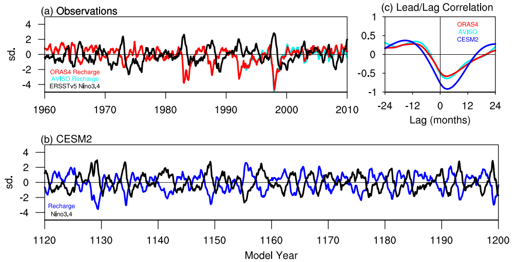
Figure 9. (a) Time evolution of the observed recharge-discharge and Niño-3.4 SST index over 1960–2010. The AVISO and ORAS4 estimates for the recharge are defined as the area-averaged sea surface height anomalies over 5°S to 5°N, 120°E to 155°W. AVISO coverage begins in 1993. (b) As in (a) but for CESM2 over years 1,120–1,200. The recharge is defined as the warm water volume integrated over 5°S to 5°N, 120°E to 155°W. All time series are standardized. (c) Lead-lag correlations of Niño-3.4 and the recharge-discharge in observations and CESM2 (model years 800–1,200). Positive (negative) lags indicates Niño-3.4 leads (lags) the recharge.
