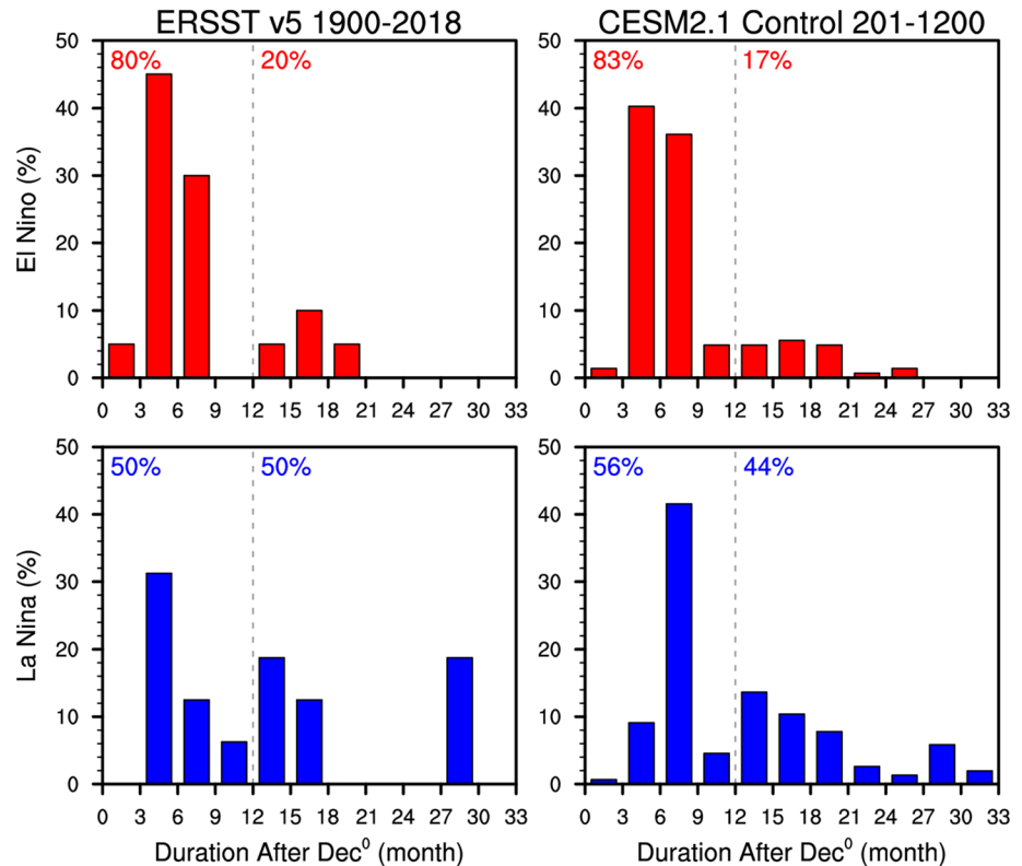
Figure 7. Frequency distribution (%) of (top row) El Niño and (bottom row) La Niña duration (in months) for (left column) observations (detrended ERSSTv5 1900–2018) and (right column) CESM2 control simulation (model years 201–1,200). The El Niño (La Niña) duration is defined as the number of months for which the Niño-3.4 index remains above 0.25 standard deviations (below -0.25 standard deviations) after December of year 0. The number of El Niño (La Niña) events in each 3-month bin is divided by the total number of El Niño (La Niña) events. The numbers near the top of each panel indicate the fraction of events that terminate in year + 1 (left numeral) and persist through year + 1 (right numeral).
