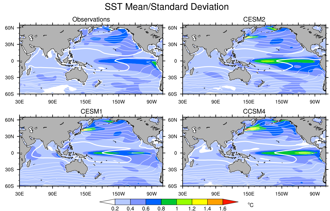
Figure 1. Mean SST (white contours) and SST monthly standard deviation (color shading) for detrended ERSSTv5 over 1900–2018 (top left), and 1,000-year segments of the preindustrial control simulations of CESM2 (top right), CESM1 (bottom left), and CCSM4 (bottom right). Contour interval is 3°C and the thick white contour indicates the 27°C isotherm.
