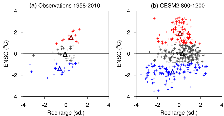
Figure 10. Scatterplot of the standardized March recharge-discharge with the following December Niño-3.4 SST anomaly in (a) observations and (b) CESM2 years 800–1,200. Blue markers indicate La Niña events, black markers indicate neutral, and red markers indicate El Niño events. The threshold for El Niño (La Niña) is exceedance of the + (–) one standard deviation of the observed Niño-3.4 SST anomaly over 1958–2010. Bold triangles indicate the average over each of the three ENSO categories.
