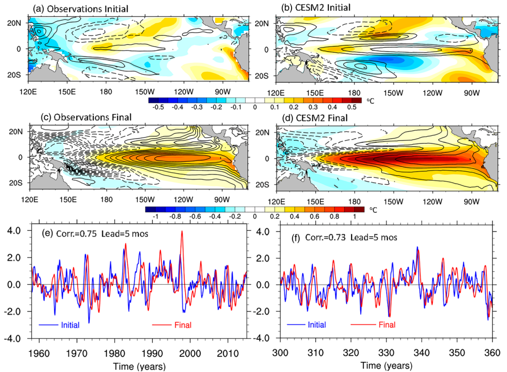
Figure 11. Initial (a, b) and final (c, d) optimal structures obtained with LIMs trained on observations (a, c, and e) and CESM2 (b, d, and f). Shading is for SST and contours are for SSH (contour interval is 0.5 cm for the initial and 1 cm for the final optimal structures, respectively). Bottom panels show the time series associated with the initial (blue) and final (red) optimal structures for the observations (left), and a 60-year segment of CESM2 (right). The observational (CESM2) LIM is trained over the period 1958–2014 (model years 201–1,200).
