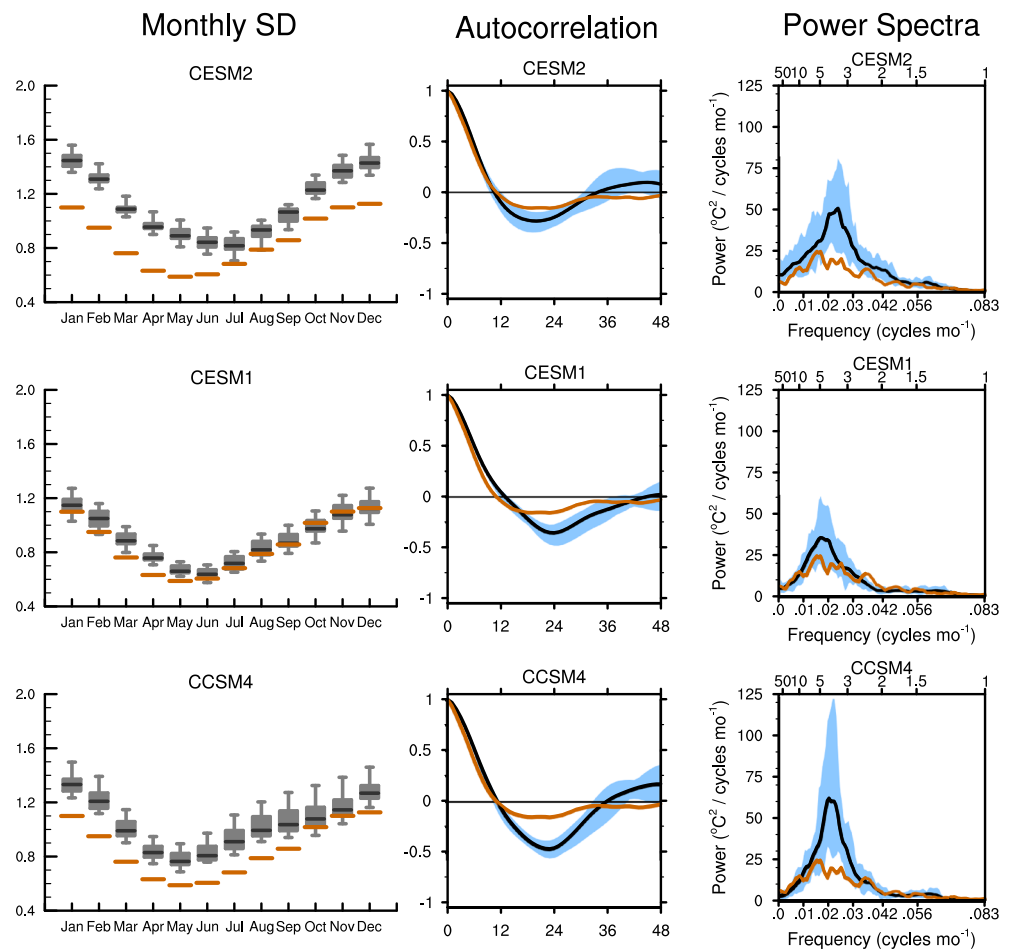
Figure 3. Monthly standard deviations (left panels), autocorrelation functions (middle panels, x axis showing lags in months), and power spectra (right panels) of the detrended Niño-3.4 index for the piControl simulations of CESM2 (top row), CESM1 (middle row), CCSM4 (bottom row), and ERSST.v5 (red lines). The range of estimates for the models were obtained by dividing their 1,000-year Niño-3.4 records in 18,119-year partially overlapping segments. The light blue shading in the middle (right) panels shows the minimum and maximum values of the autocorrelation (spectral estimate) at each lag (frequency). The statistics of the monthly standard deviations in the left panels are summarized through the use of boxplots and whiskers showing the minimum values (whiskers minima), first quartiles (lower edge of the boxes), median (black lines), third quartiles (upper edge of the boxes), and maximum values (whiskers maxima) of the standard deviations for each month.
