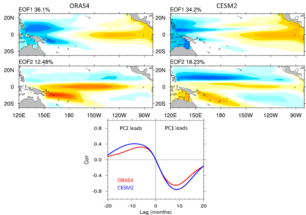
Figure 8. Leading EOFs of SSH for ORAS4 (1958–2014, left panels) and CESM2 (model years 201–1,200, right panels). Top panels show EOF1 for the two data sets, middle panels show EOF2, and bottom panel displays the lag correlation between the associated PCs, with PC1 leading PC2 for positive lags. In both ORAS4 (red line) and CESM2 (blue line), the lag correlations indicate that EOF1, associated with the peak of the positive ENSO phase, leads the negative phase of EOF2, that is, a discharged equatorial Pacific thermocline. Conversely, a recharged state (positive EOF2) leads to the positive phase of EOF1, that is, the development of an El Niño event.
