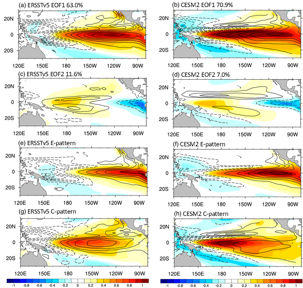
Figure 13. Linear regression of the SST anomalies ( ^{\circ}\text{C} , shading) and SSH anomalies (cm, contours) on PC1 (a, b), PC2 (c, d), E-index (e, f), and C-index (g, and h). The observational PCs were obtained from EOF analysis of 1900–2018 ERSSTv5 SST anomalies in the 10^{\circ}\text{S} to 10^{\circ}\text{N} tropical Pacific domain, while the CESM2 PCs were computed from EOF analysis of the model SST anomalies over model years 201–1,200 and over the same 10^{\circ}\text{S} to 10^{\circ}\text{N} tropical Pacific domain. SSH observations are from the ORAS4 reanalysis, and the corresponding regressions are based on the 1958–2015 period. Contour interval for SSH is 1 cm. The variance explained by the SST EOFs in the 10^{\circ}\text{S} to 10^{\circ}\text{N} domain is shown above the panels displaying the EOF patterns.
