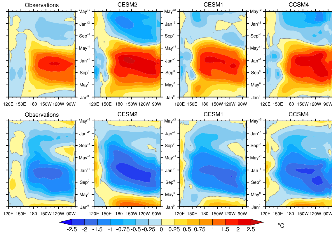
Figure 6. Longitude time sections of composite SST anomalies along the equator ( 3^{\circ}\text{S} to 3^{\circ}\text{N} ) for (top) El Niño and (bottom) La Niña based on observations (ERSSTv5 over 1900–2018, left panels), CESM2 (model years 201–1,200, second column), CESM1 (model years 1,201–2,200, third column), and CCSM4 (model years 301–1,300, right panels). See text for details of the compositing methodology.
