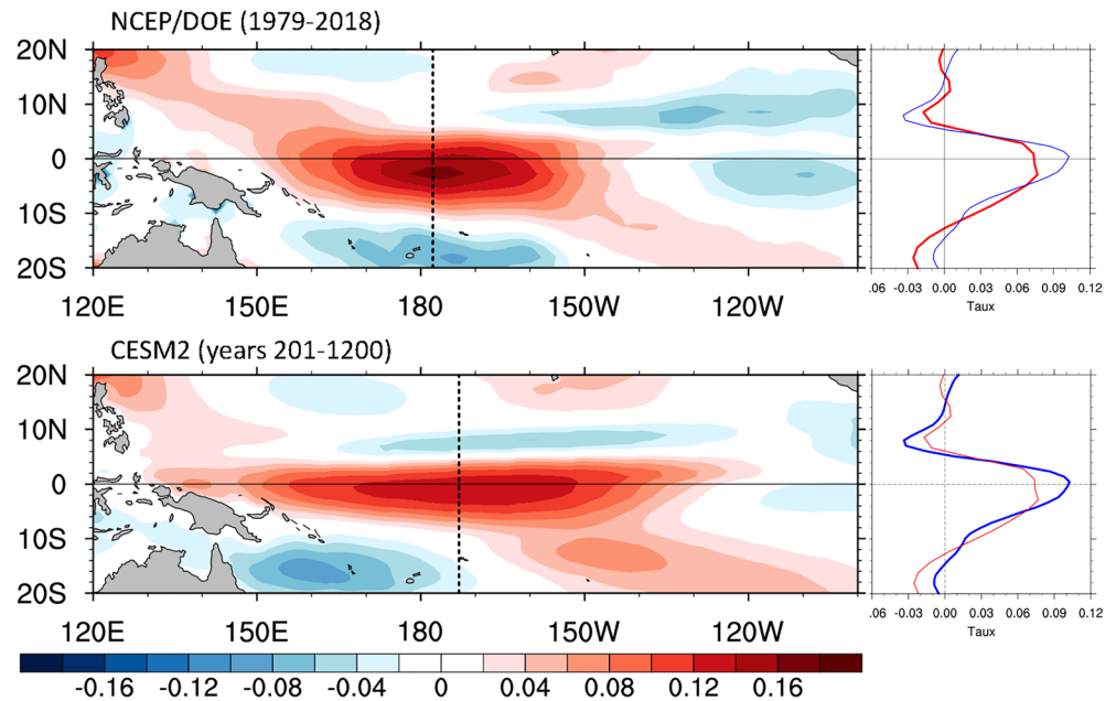
Figure 5. Regression of zonal wind stress upon the normalized Niño-3.4 index for observations (zonal wind stress from the NCEP/DOE reanalysis over 1979–2018, and Niño-3.4 index from detrended ERSSTv5 over the same time period, top-left) and CESM2 (years 201–1,200, bottom left) as a function of longitude and latitude, and their zonal average (right panels). Dashed line in the left panels shows the “center of mass” of the positive zonal wind stress anomalies computed as the equatorial (2°S to 2°N) zonal wind stress anomaly weighted longitude between 140°E and 120°W. Right panels show the zonal average of the zonal wind stress, from 20°S to 20°N, with red used for the observations and blue used for CESM2. The latitudes of zero crossing in the right panels are used to define the meridional scale L_y of the anomalous zonal wind stress for both observations and model. L_y is 18.8° of latitude for the observations and 20° for CESM2.
