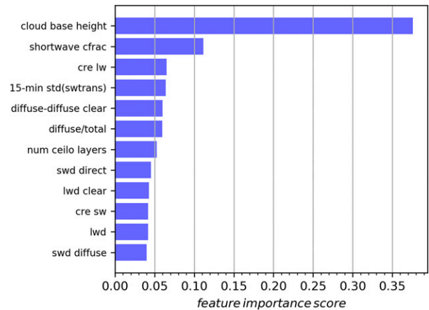
FIG. 4. Feature importance scores determined from the subset of training data at ARM SGP during 2014–17.
