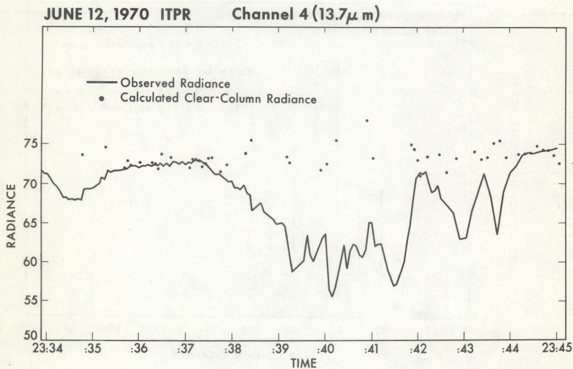
Figure V-4.--Observed radiances (solid line) and calculated clear-column (dots) for the ITPR 13.7\text{-}\mu\text{m} \text{CO}_2 channel.
