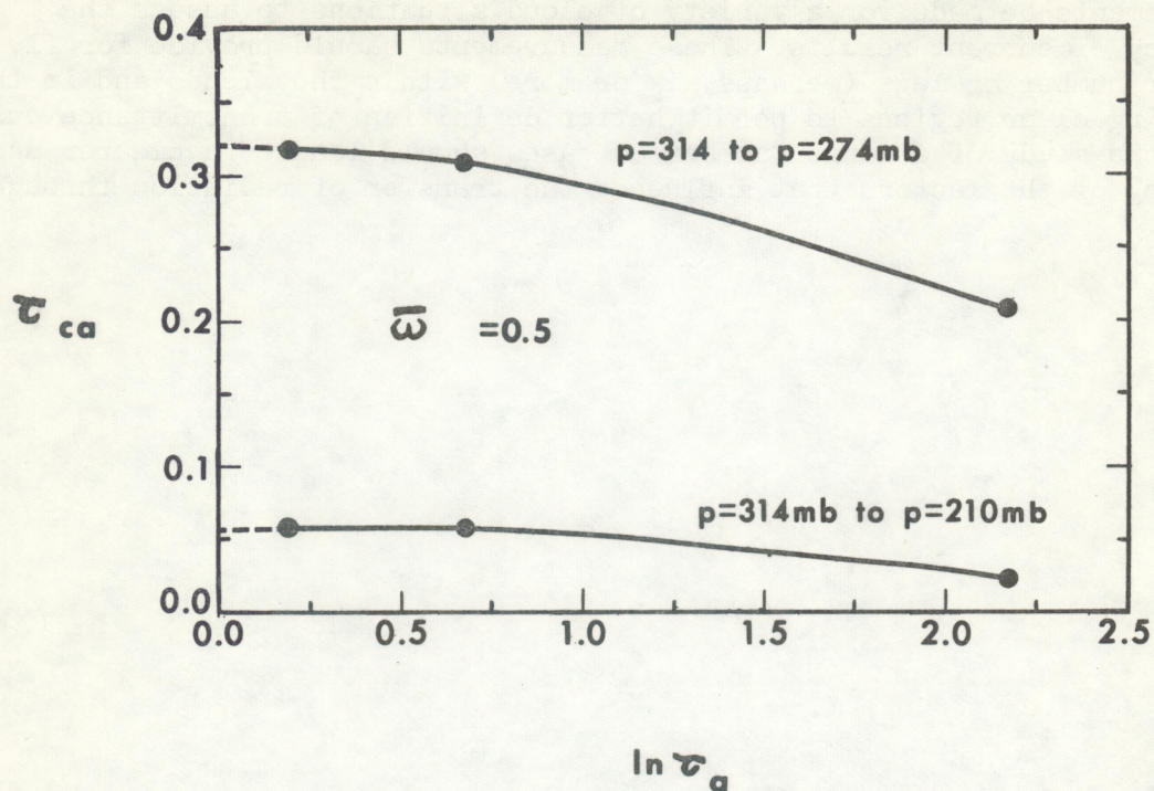
Figure VII-8.--Cloud transmittance ( \tau_{ca} ) for flight 10 vs the negative of the logarithm of the clear air transmittance ( -\ln \tau_a for the thickest layer in flight 2).
