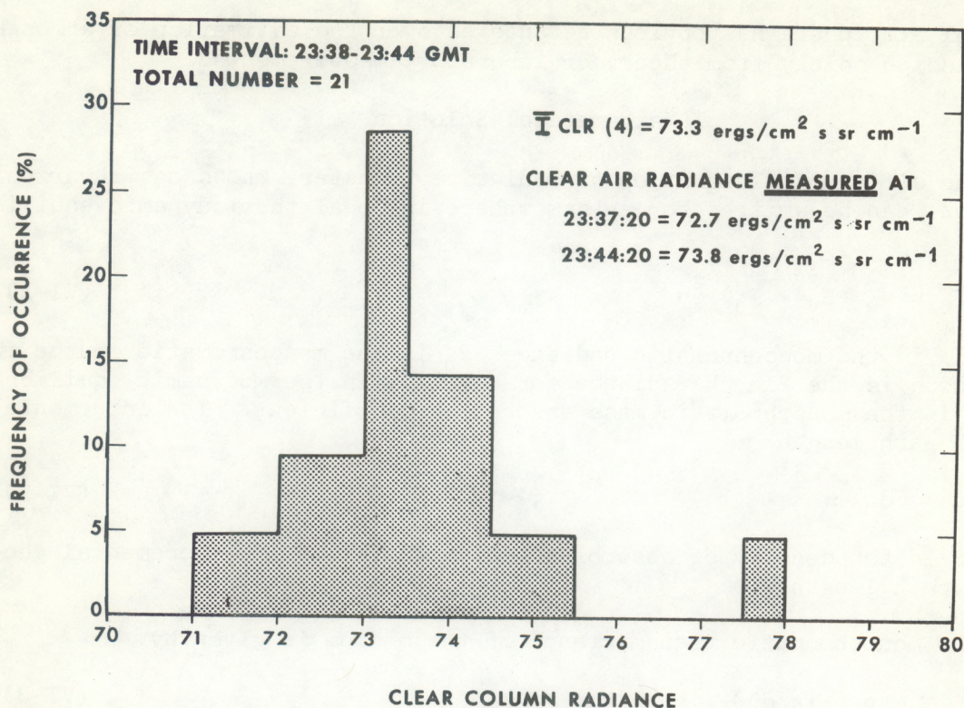
Figure V-7.--Histogram of clear-column radiances deduced from cloud-contaminated radiance measured in the 13.7\text{-}\mu\text{m} \text{CO}_2 channel.
