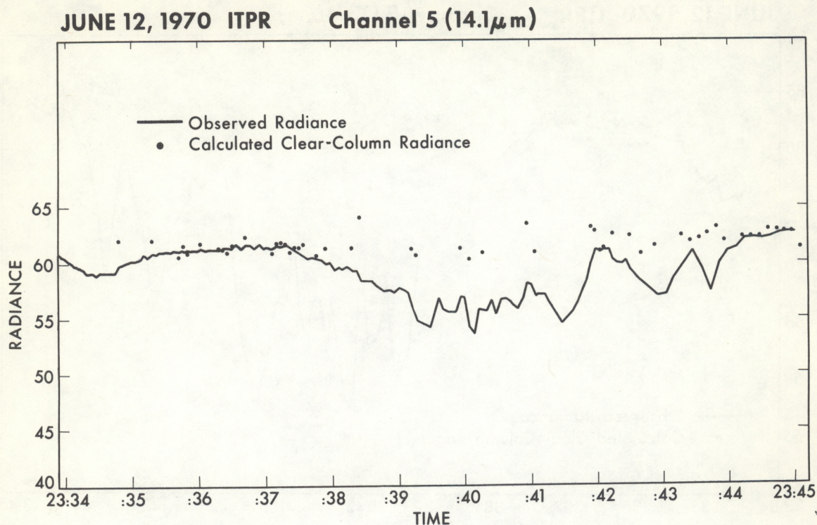
Figure V-5.--Observed radiances (solid line) and calculated clear-column radiance (dots) for the ITPR 14.1\text{-}\mu\text{m} \text{CO}_2 channel.
