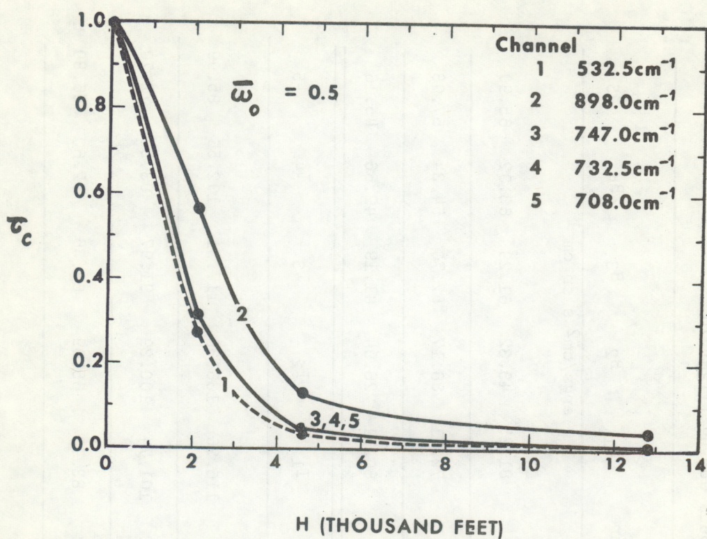
Figure VII-5.--"Pure" cloud transmittance ( \tau_c ) vs the elevation (H) above the base of the cloud (Flight 2).
