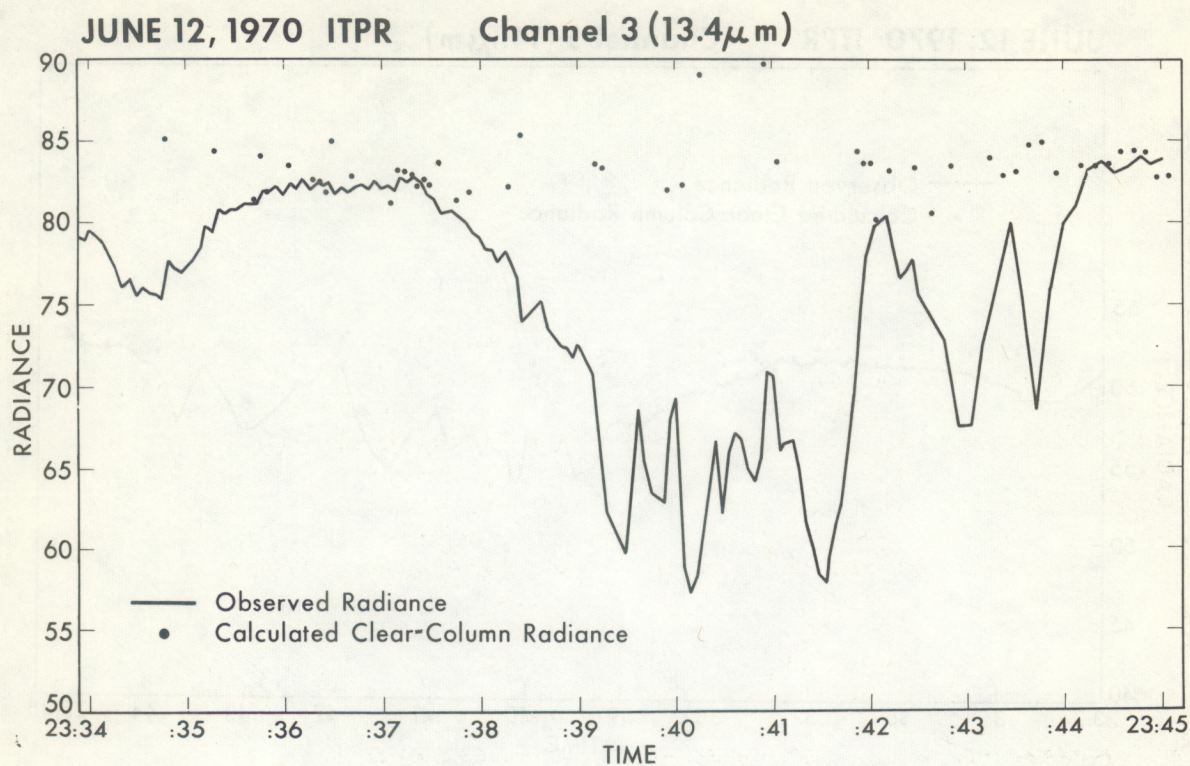
Figure V-3.--Observed radiances (solid line) and calculated clear-column radiance (dots) for the ITPR 13.4\text{-}\mu\text{m} \text{CO}_2 channel.
