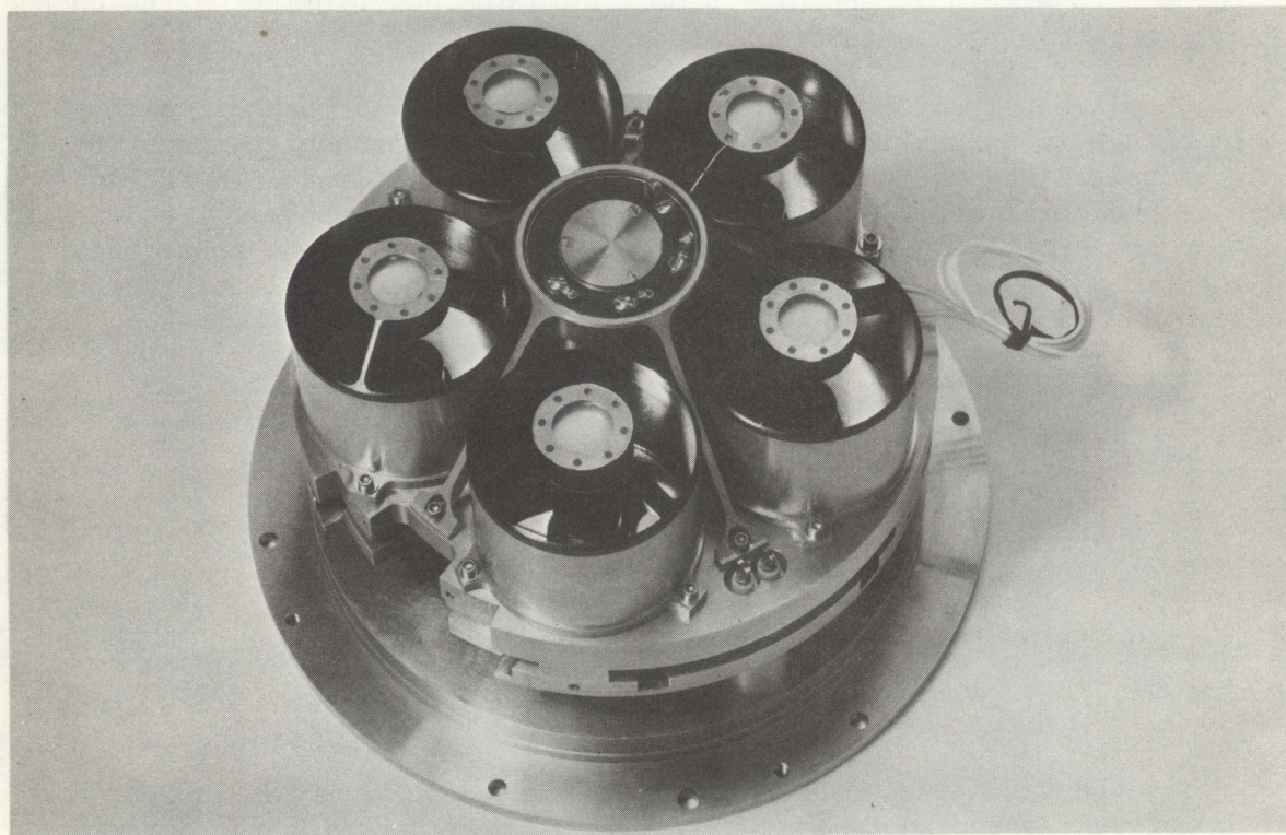
Figure II-5.--ITPR optics deck containing the channel telescopes.
