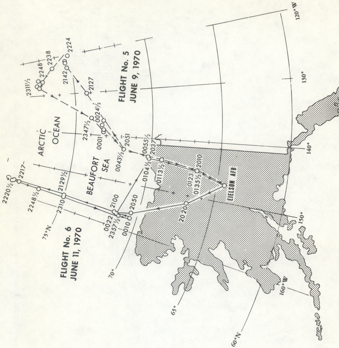
Figure I-3.--Ground tracks for Convair-990 Flights No. 5 and 6.
