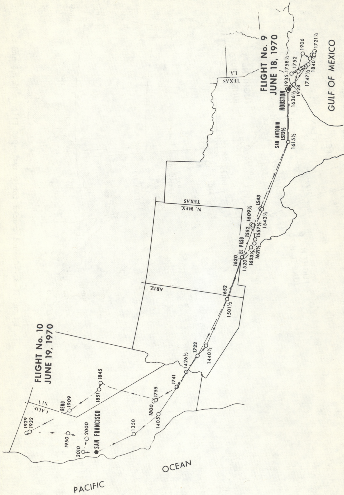
Figure I-4.---Ground-tracks for Convair-990 Flights No. 9 and 10.
