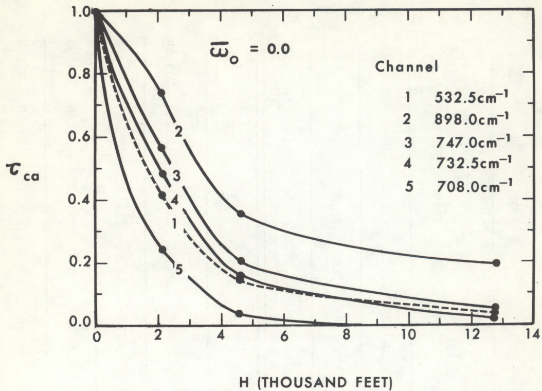
Figure VII-1.--Cloud transmittance ( \tau_{ca} ) vs the elevation (H) above the base of the cloud (Flight 2).
