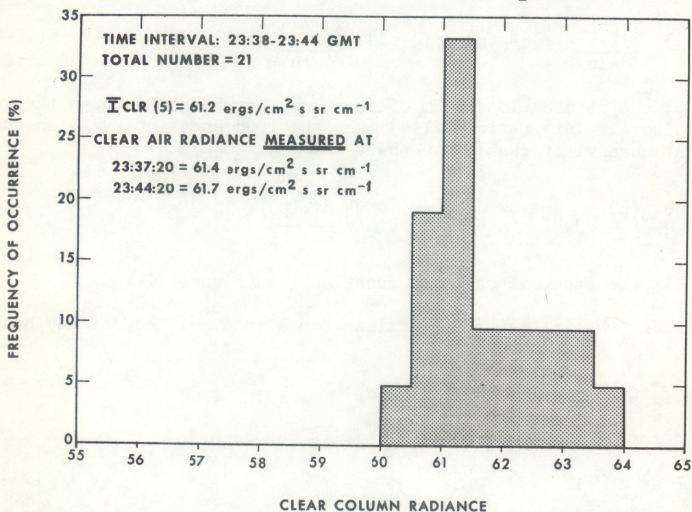
Figure V-8.--Histogram of clear-column radiances deduced from cloud contaminated radiances measured in the 14.1\text{-}\mu\text{m} \text{CO}_2 channel.
