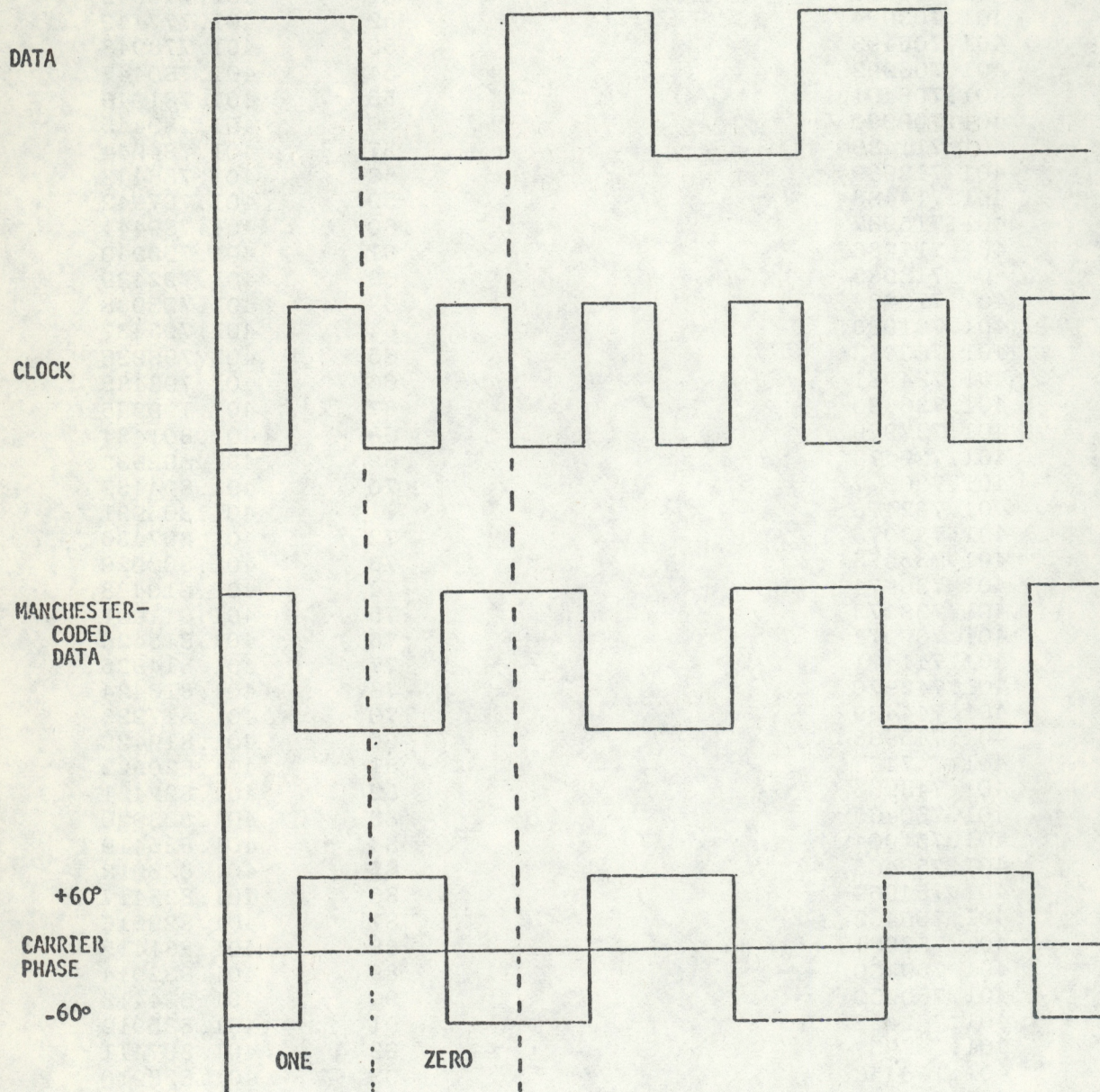
Figure 1.--Modulation Definition.
