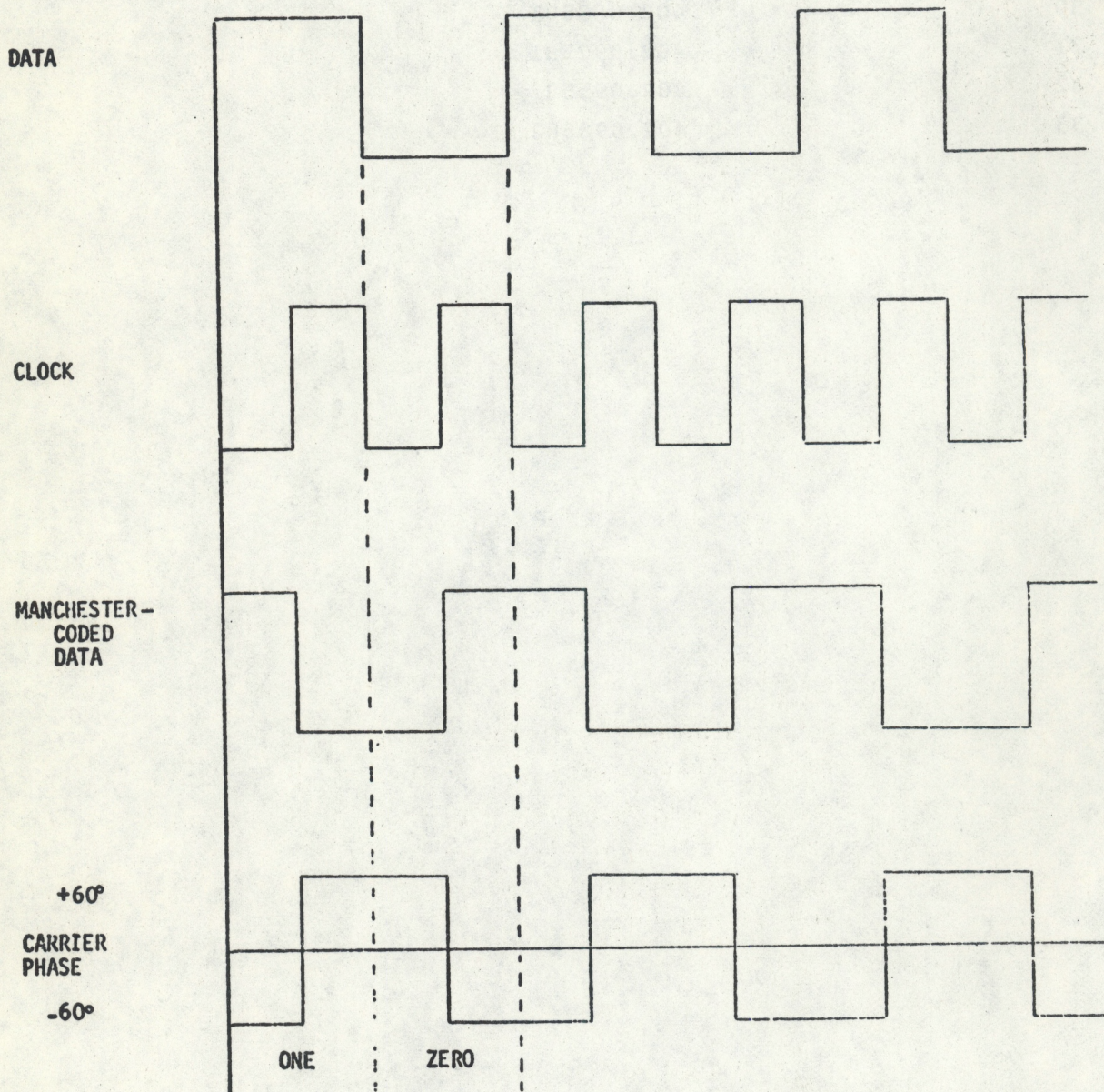
Figure 1.--Modulation Definition.
