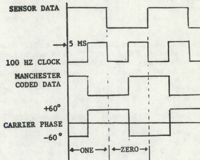
Figure 6.--Modulation Definition.
