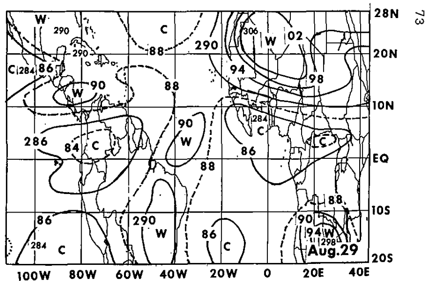
Figure 39--Same as Figure 34 except this is for 850-mb temperature.
