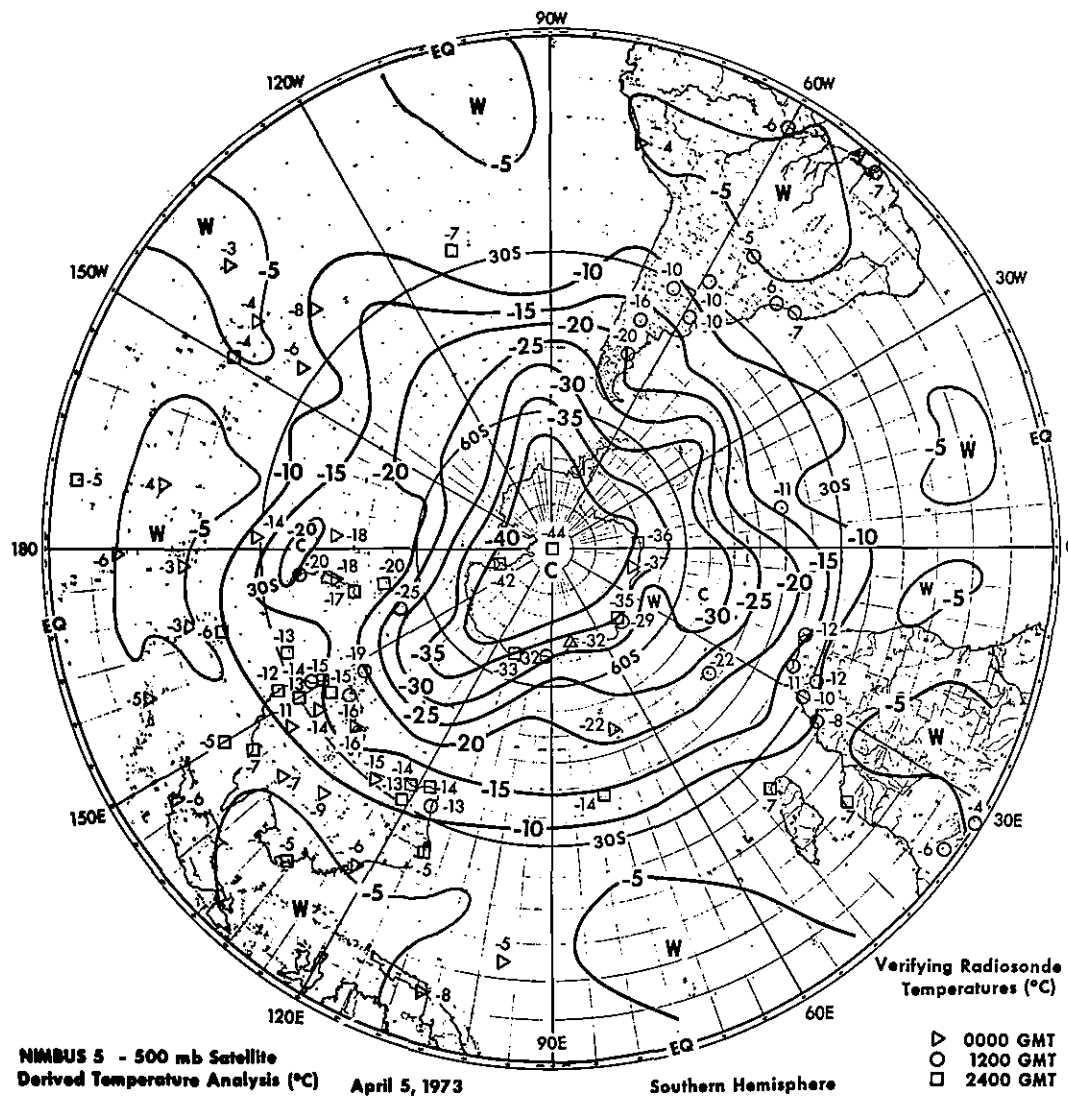
Figure 14--Southern Hemisphere 500-mb temperature analysis based solely on Nimbus-5 radiance data on April 5, 1973. Available radiosonde observations are shown to verify the Nimbus-5 data. ▷, 0000 GMT; ○, 1200 GMT; □, 2400 GMT.
