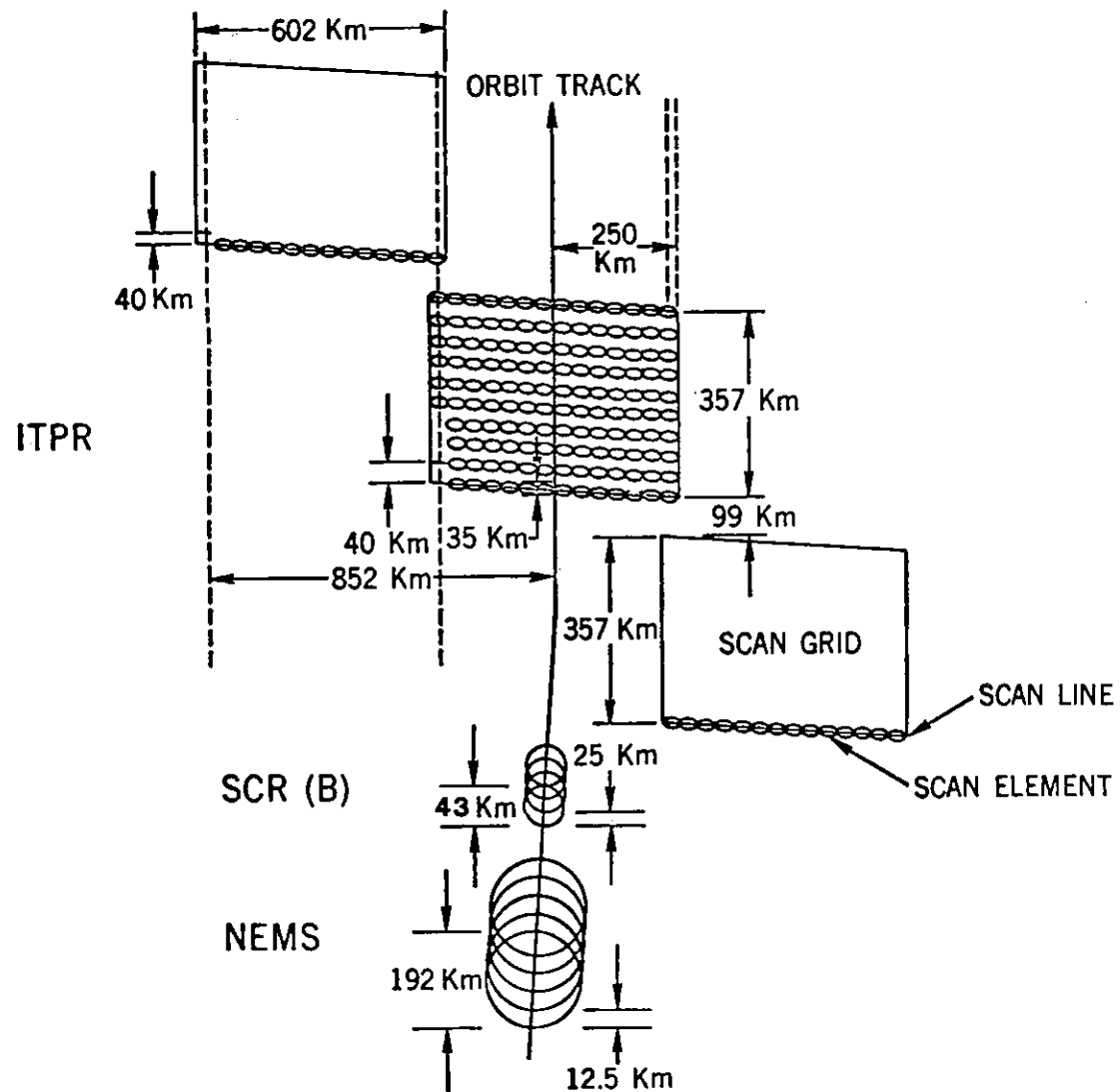
Figure 3--The earth fields of view for the ITPR, NEMS and SCR instruments.
