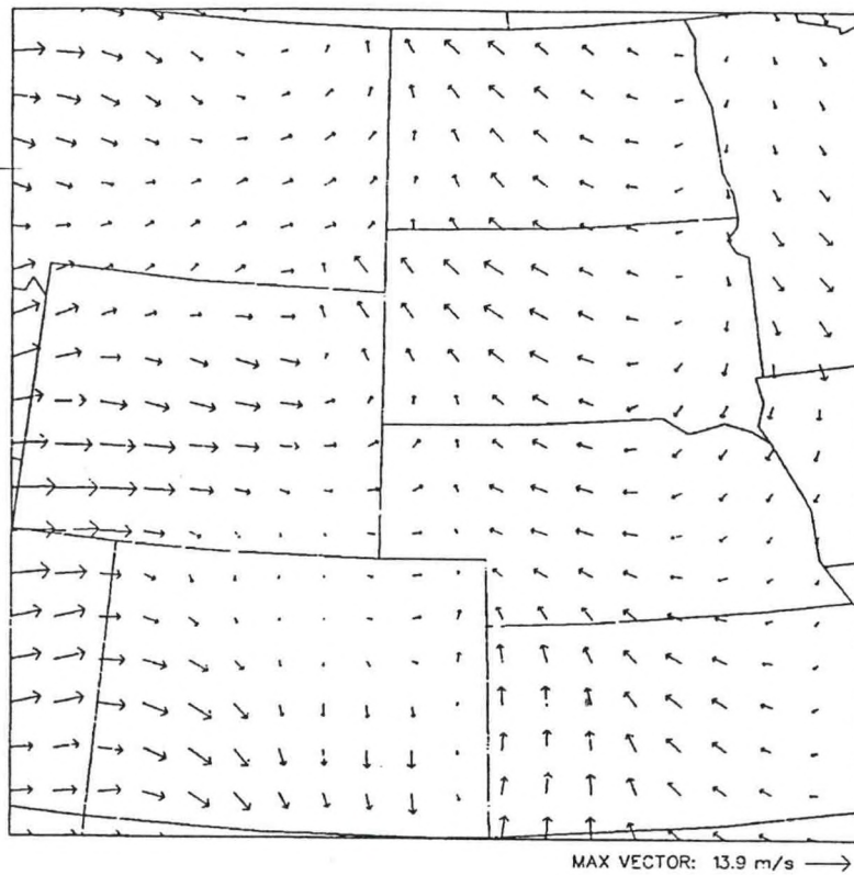
Figure 4. Interpolated surface wind vectors ( \text{m s}^{-1} ) for 2200 UTC 29 June 1994. Calculations performed using WXP (Purdue Weather Processor via Unidata) based on the surface data in Figure 2 (less the manually plotted stations).
