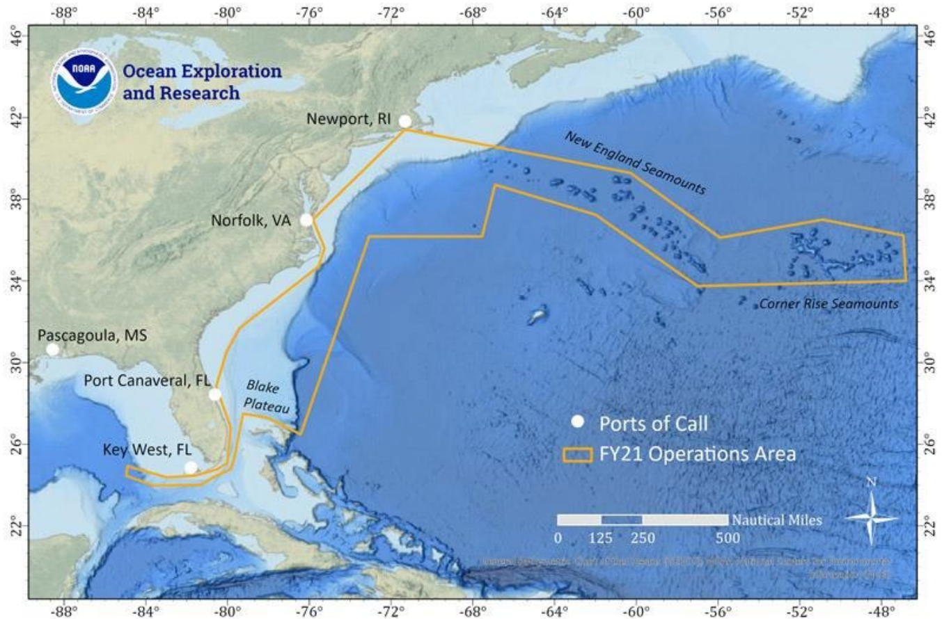
Overview map of the field operations area for NOAA OER expeditions in FY2021.
