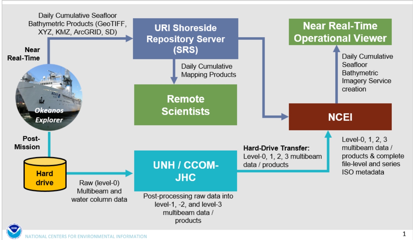
Figure 3. Okeanos Explorer Multibeam Data Pipeline.
