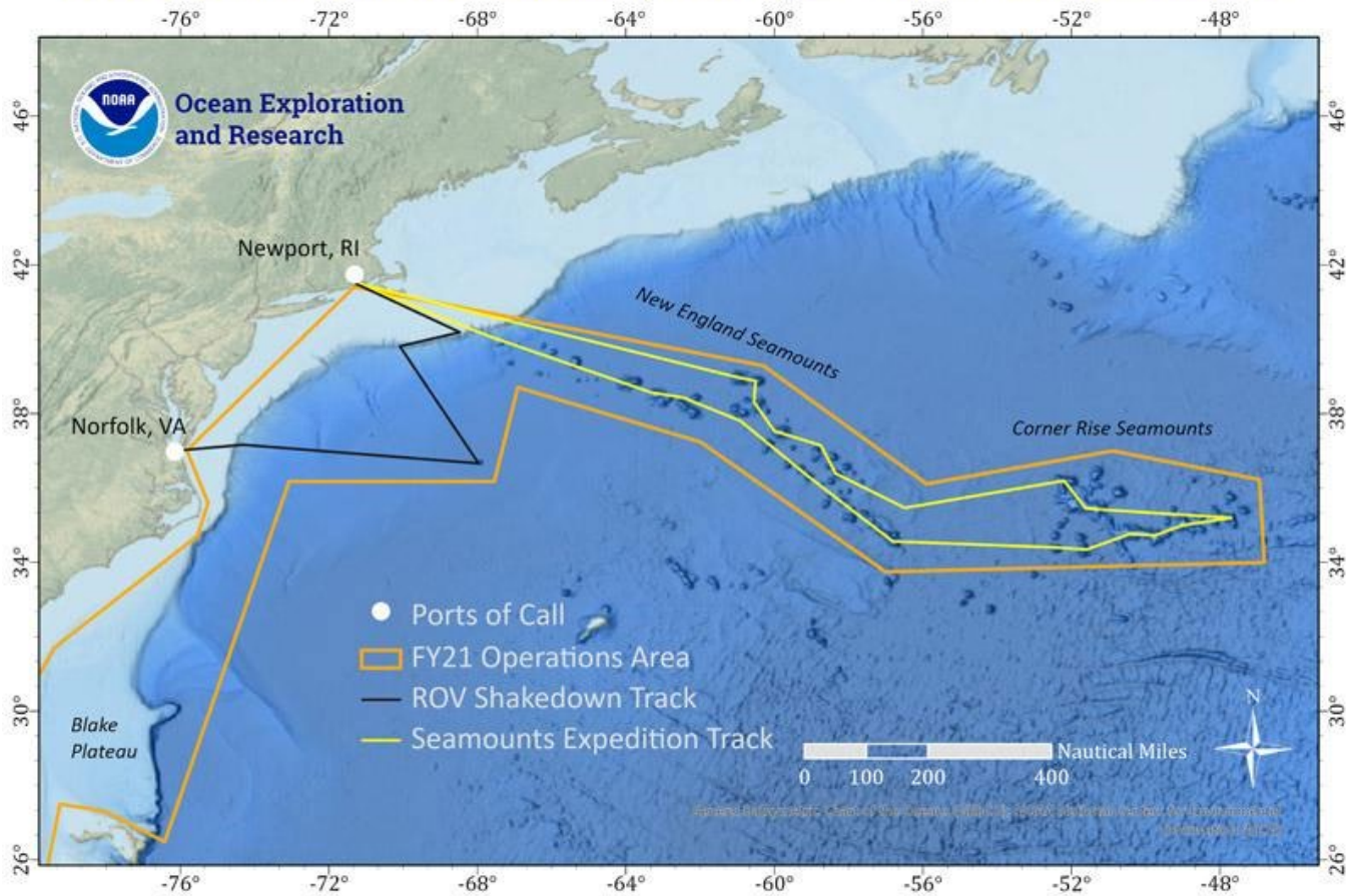
Figure 3. Map showing the operations area (orange polygon) and approximate expedition track lines for the ROV shakedown expedition (black line) and the 2021 North Atlantic Stepping Stones: New England and Corner Rise Seamounts expedition (yellow line). Exploratory mapping and ROV work will focus on the New England Seamounts and Corner Rise Seamounts offshore of the eastern United States.
