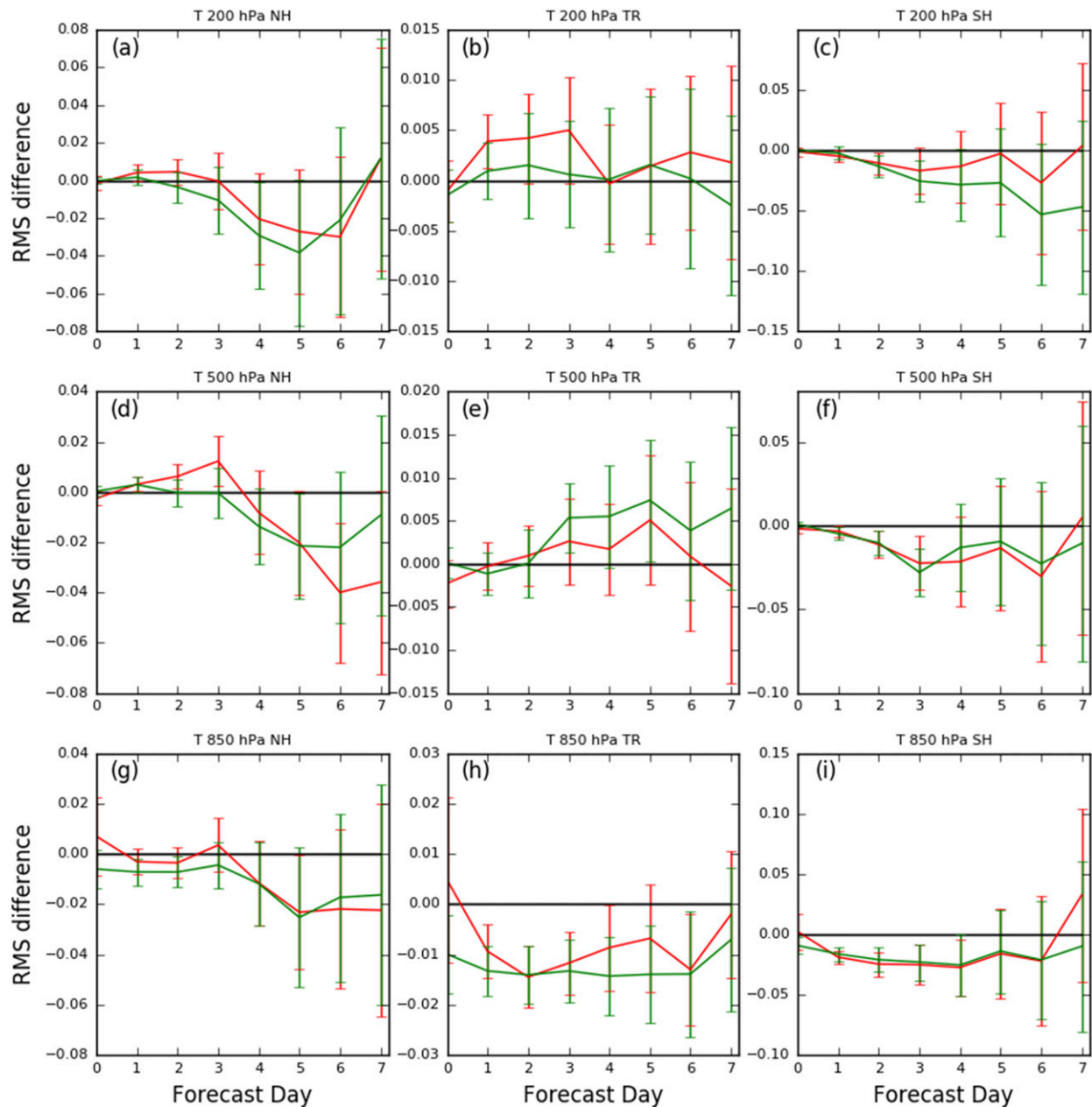
FIG. 17. The change in temperature RMS forecast error (K) with respect to the CNTL for ALLQ (red) and ALLQ_cycle_hydro (green) in the (left) Northern Hemisphere, (center) tropics, and (right) Southern Hemisphere at (a)–(c) 200, (d)–(f) 500, and (g)–(i) 850 hPa. The verification period is from 26 Jun to 31 Aug 2017. The error bars indicate the 95% confidence interval. Reduced RMS error indicates better forecast.
