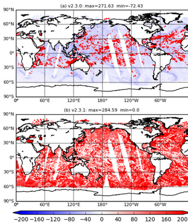
FIG. 3. Emissivity Jacobian (K) of AMSU-A (including NOAA-I5, NOAA-I8, NOAA-I9, and MetOp-A) channel 2 calculated from the CRTM (a) before and (b) after the code error correction.
