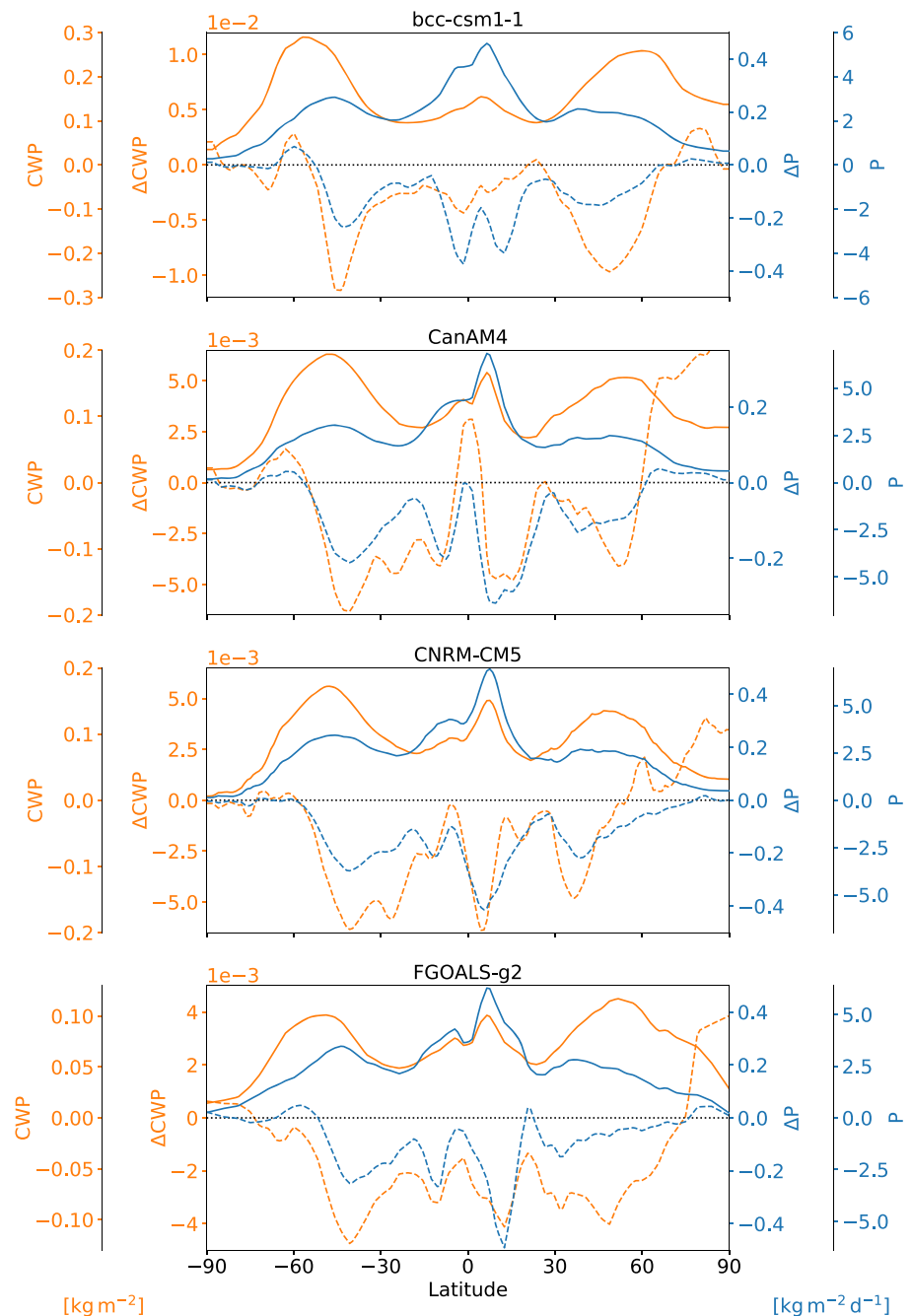
Figure 1. Latitudinal profiles of cloud water path (CWP) and precipitation (P) in the base state (solid) and the changes following rapid adjustment (dashed) diagnosed from the AMIP and AMIP4×CO 2 experiments produced by the bcc-csm1-1, CanAM4, CNRM-CM5, and FGOALS-g2 models.
