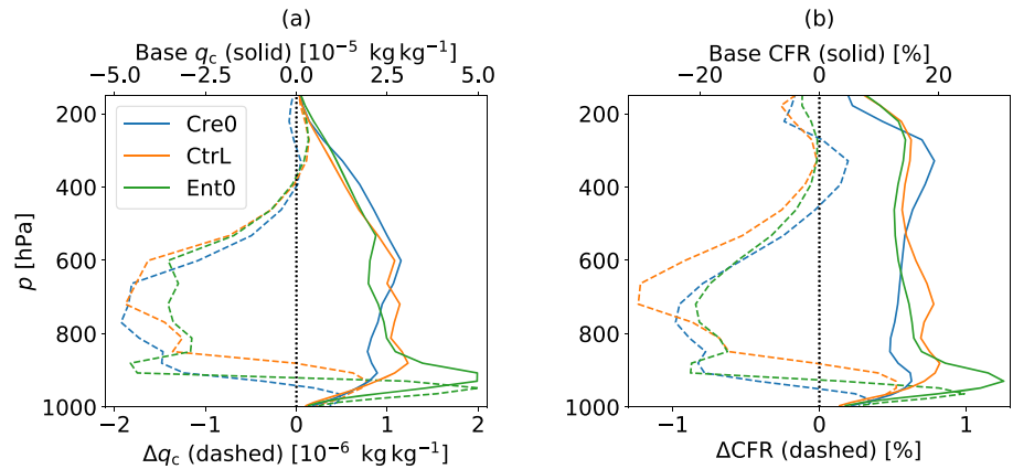
Figure 6. Vertical profiles of the global average (a) cloud water mixing ratio q_c and (b) cloud fraction (CFR) in the base state (solid) and the changes following rapid adjustment under 4\times\text{CO}_2 (dashed) in the HiRAM aqua planet simulations.
