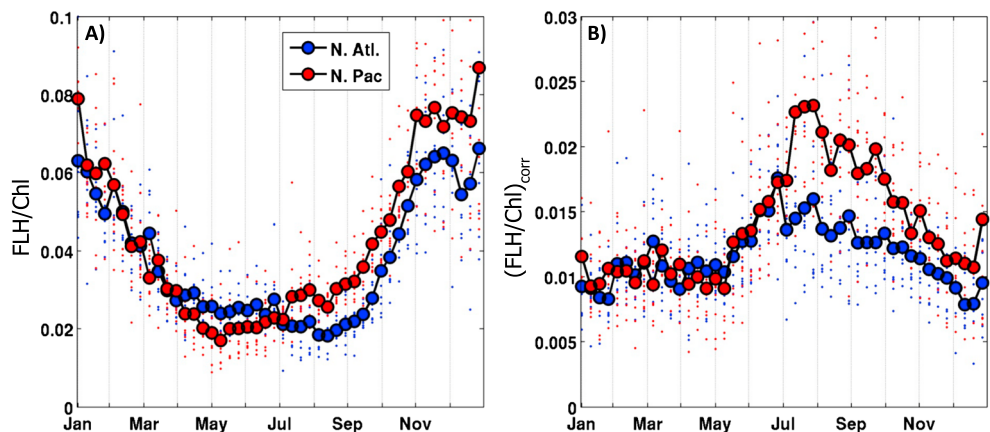
Figure 6. Climatological annual cycles in chlorophyll fluorescence efficiency as an indication of iron stress in the North Atlantic (large blue circles) and North Pacific (large red circles). (a) FLH/Chl fluorescence line height (FLH) normalized to Chl. (b) FLH/Chl corrected for effects of photoacclimation and nonphotochemical quenching. Climatologies were constructed from weekly (8 day) composites of MODIS data over a 10 year period (2003–1012) averaged over 5^{\circ} \times 10^{\circ} boxes shown in Figure 1. Small points represent all 8 day data from the 10 year study period.
