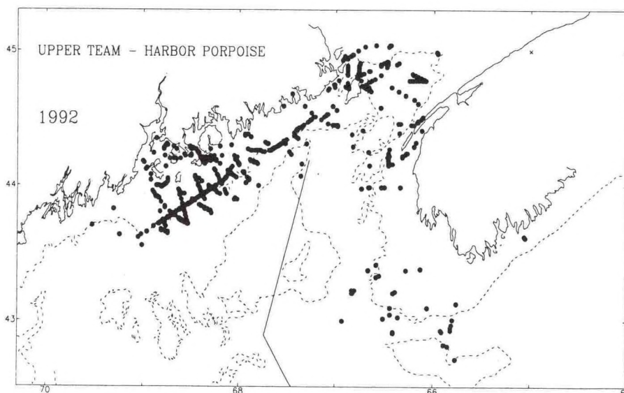
Figure 39.2. Map of area of operation for 1992 harbor porpoise survey showing harbor porpoise sightings recorded by one of two teams which was located in the upper crew's nest of the R/V Abel-J.
