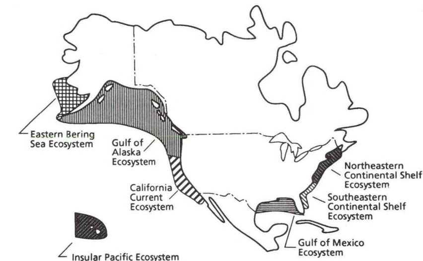
Figure 8. The seven large marine ecosystems of the United States, including the insular Pacific Hawaiian Islands.
