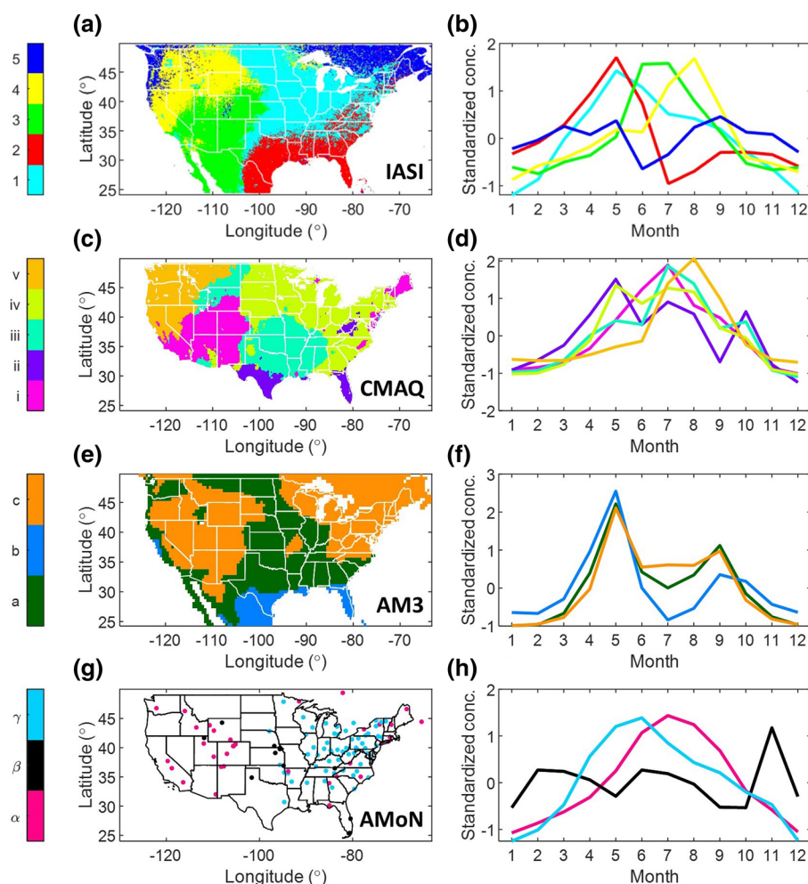
Figure 3. IASI, CMAQ, AM3, and AMoN NH 3 seasonality clusters map (a), (c), (e), and (g) and standardized NH 3 concentrations for each cluster (b), (d), (f), and (h).
