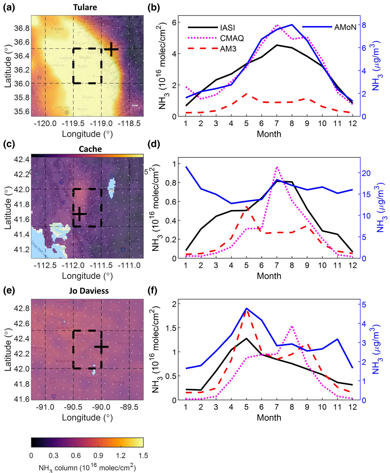
Figure 4. Comparison of NH 3 seasonality in hotspots regions. Panels (a), (c), and (e) are the annual averaged IASI oversampled NH 3 column concentrations. The bold black dashed box indicates the selected hotspot regions. The black cross shows the nearby AMoN site. Black dashed lines represent AM3 grid boxes, and white dots represent the center of CMAQ grids. (b), (d), and (f) are the NH 3 seasonality derived from the IASI oversampling NH 3 column, CMAQ, and AM3 modeled NH 3 columns (left axis), and AMoN NH 3 concentration (right axis). Map data from Google Earth.
