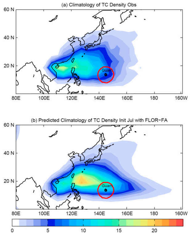
FIG. 17. The (a) observed (GuamTC = 5.1) and (b) predicted (FLOR-FA, GuamTC = 5.7) TC density climatology in the peak season (JASO) in the WNP [color shading, occurrences (TC_{season})^{-1} ]. The black symbol and the red outer circle denote Guam and its 500-km buffer zone.
