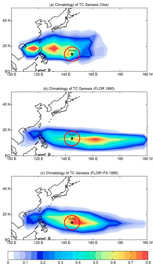
FIG. 2. As in Fig. 1, but for TC genesis in the peak season.
