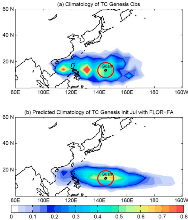
FIG. 18. The (a) observed and (b) predicted (FLOR-FA; initialized in July) TC genesis climatology in the peak season (JASO) for 1980–2014 in the WNP [color shading, occurrences (TCseason) -1 ]. The black symbol and the red outer circle denote Guam and its 500-km buffer zone.
