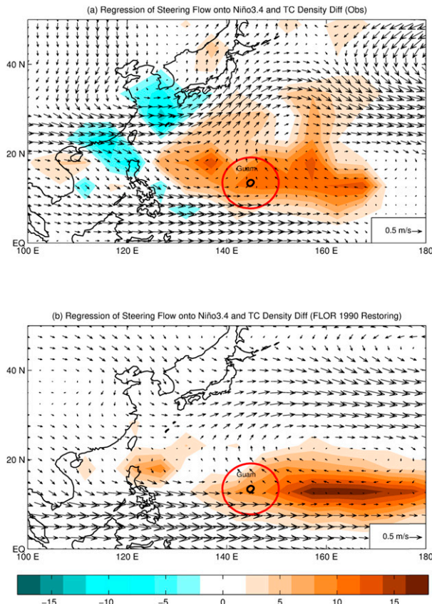
FIG. 16. Regression of steering flow (vectors, m s^{-1} \text{ } ^\circ C^{-1} , see legend at bottom right of each panel) onto the Niño-3.4 index and TC density difference (color shading, El Niño minus La Niña) in the (a) observations and (b) SST-nudging experiments with FLOR 1990. The black circle and the outer red circle denote Guam and its 500-km buffer zone.
