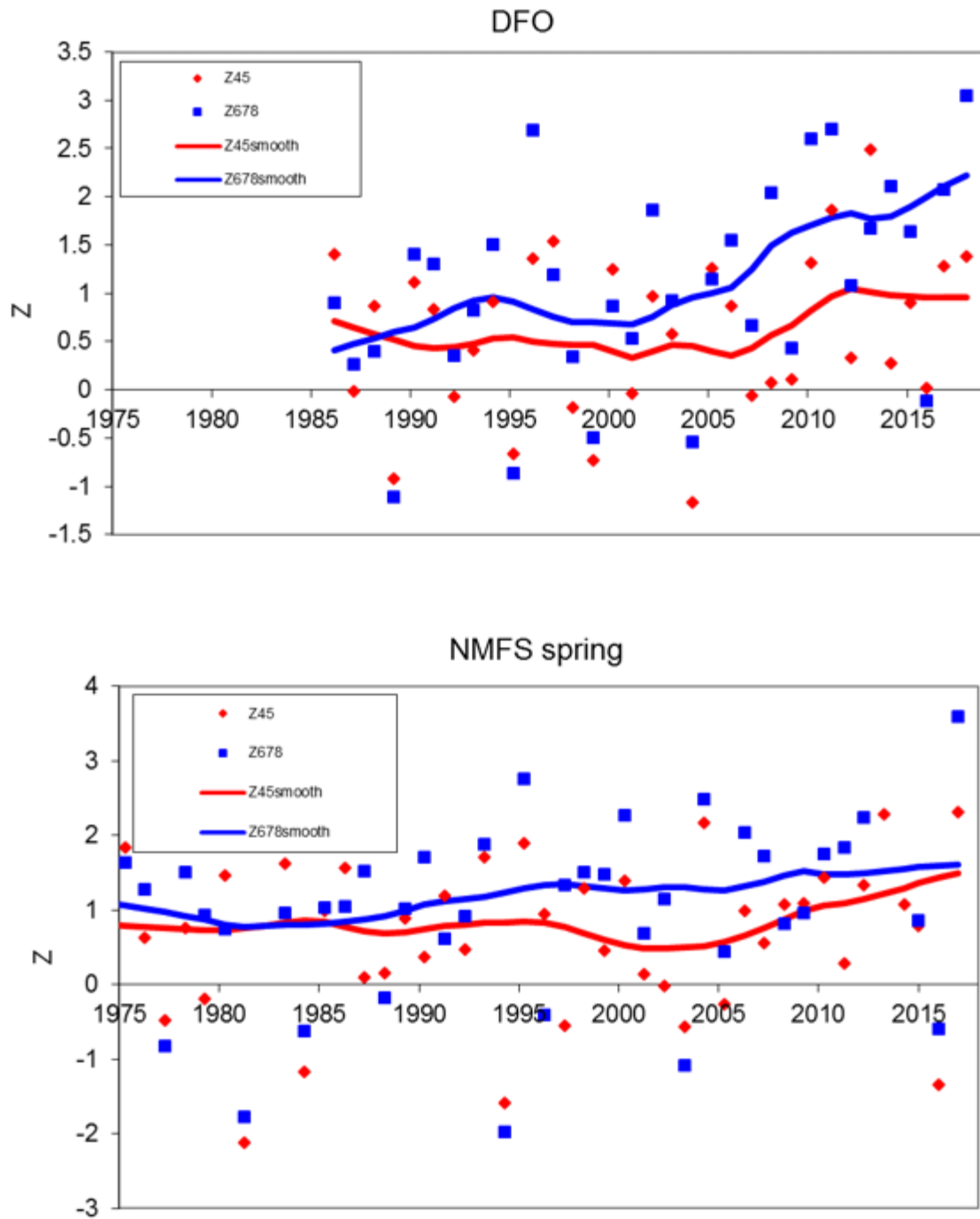
Figure A5. Total mortality (Z) calculated using the DFO spring and NMFS spring surveys data for Eastern Georges Bank Cod. Due to Covid-19 restrictions ages were unavailable for the 2020 DFO spring survey and the 2020 NMFS survey was cancelled.
