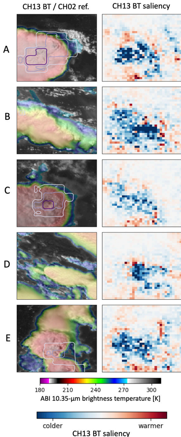
FIG. 18. Saliency plots for ABI CH13 brightness temperature (BT) for five false negative storms. The images in the first column are CH13 BT/CH02 reflectance “sandwich” imagery with GLM flash-extent density contours for 10, 20, and 40 flashes per 5 min overlaid in shades of purple. The predicted probability for each image patch was <1\% .
