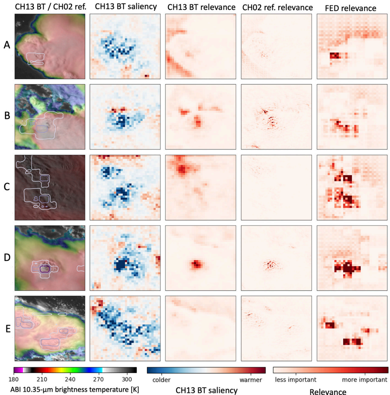
FIG. 17. As in Fig. 15, but for five false positive storm samples from the validation dataset. The predicted probability for each image patch was >87\% .
