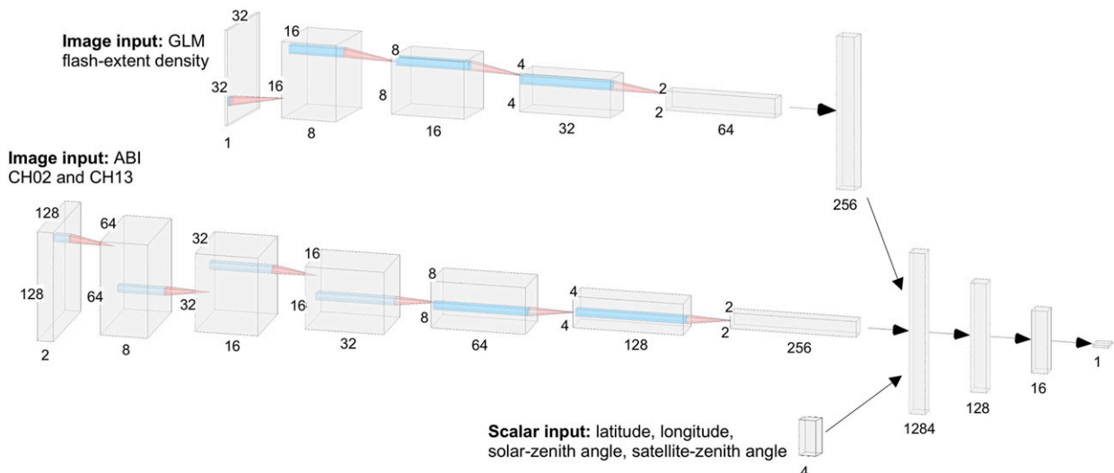
FIG. 4. Schematic of the convolutional neural network described in this paper. The blue boxes and pink pyramids represent 3 \times 3 pixel convolutional filters acting over the feature maps (or input images, initially). The dimensions for the gray boxes indicate the horizontal dimensions (the equal dimensions in each box) and the number of feature maps after 2D-convolutional and maximum pooling layers are applied (or the number of input grids, initially). In the case where one dimension is present, it is the length of the 1D vector. After several blocks of convolutions and poolings, the encoded ABI and GLM features are then “flattened,” or made into a 1D vector, and concatenated with the scalar input vector. The concatenated vector is processed through several fully connected layers to generate a probability of intense convection. This image was created at http://alexlenail.me/NN-SVG/AlexNet.html .
