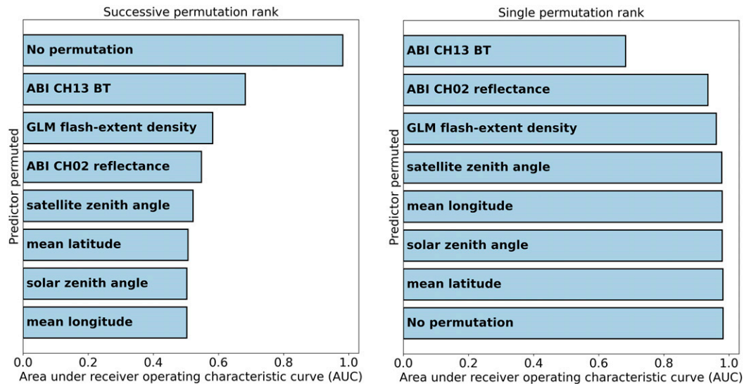
FIG. 19. The (left) successive permutation rank test and (right) single permutation rank test for the trained convolutional neural network of this paper, using 36 900 daytime-only storm samples from the validation dataset. “No permutation” represents the original AUC without any predictors permuted. For both panels, predictors increase in importance moving from the bottom to the top. ABI = Advanced Baseline Imager; GLM = Geostationary Lightning Mapper; BT = brightness temperature.
