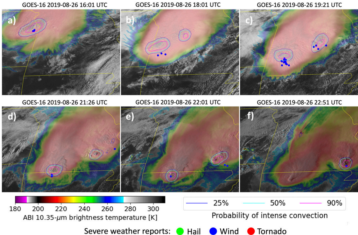
FIG. 11. As in Fig. 10, but for storms in Missouri on 26 Aug 2019. Severe weather reports (filled circles) occurred within 60 min after the satellite scan time.
