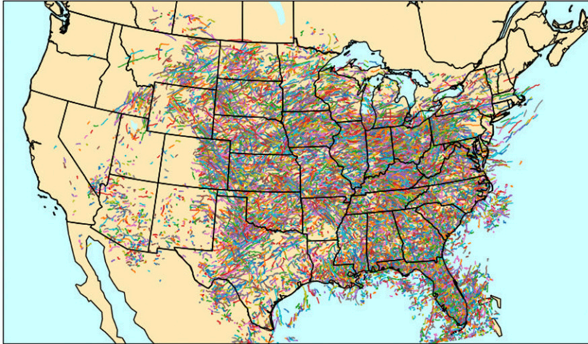
FIG. 1. All 14 746 thunderstorm tracks for the training, validation, and testing datasets. The different colors are used to help distinguish individual storm tracks.
