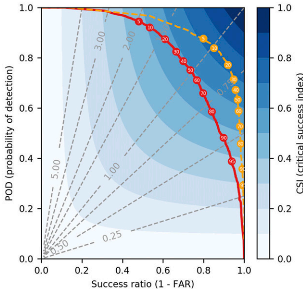
FIG. 8. Performance diagram for the validation and testing datasets (solid red and dashed orange lines, respectively). Intersections with the dashed gray lines indicate the frequency bias. Red and orange circles represent the locations of select probability values. Python code from Lagerquist and Gagne (2019) was used to help create the plot.
