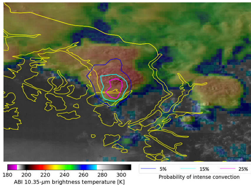
FIG. 14. As in Fig. 10, but for storms in the Alaska Panhandle on 28 Jun 2019. Note that the contoured probabilities are for the 5%, 15%, and 25% thresholds.
