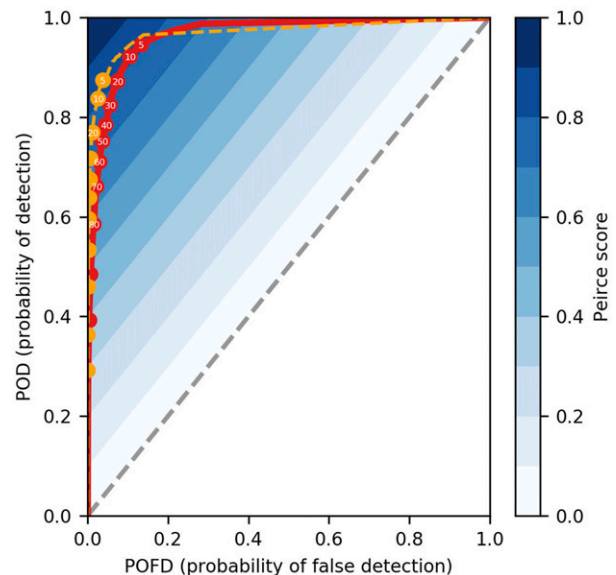
FIG. 7. ROC curve and Peirce score for the validation and testing datasets (solid red and dashed orange lines, respectively). Red and orange circles represent the locations of select probability values (5%, every 10% from 10% to 90%, and 95%). Python code from Lagerquist and Gagne (2019) was used to help create the plot.
