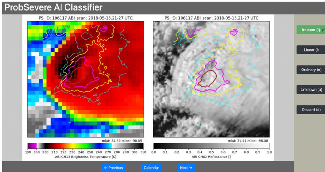
FIG. 3. Example images in the tool that was used to create the labeled dataset of “intense” and “ordinary” convection classes. A different version of these images, without overlays, text, and color bars, was used for training, validation, and testing. Contours are NEXRAD reflectivity from the Multi-Radar Multi-Sensor (MRMS) system. The 30- (cyan), 40- (yellow), 50- (magenta), and 60-dBZ (brown) reflectivity contours are shown. The human-assigned labels are uploaded to a database.
