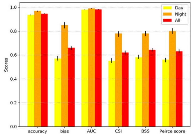
FIG. 6. As in Fig. 5, but for the testing data. The metrics were computed based on a probability threshold of 51% (which maximized validation data CSI).
