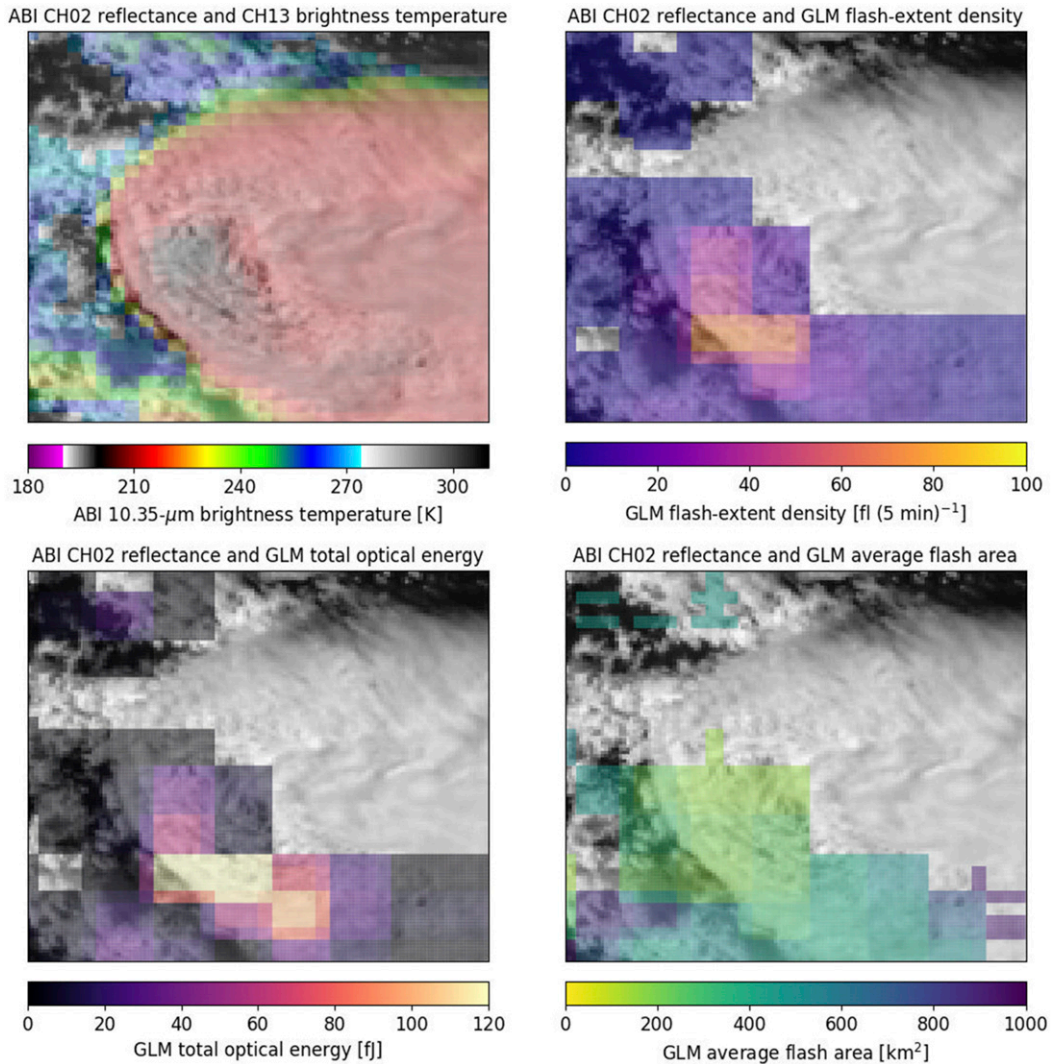
FIG. 2. GOES-16 ABI and GLM imagery of a supercell in central Texas. ABI 0.64- \mu\text{m} background image overlaid with a (top left) semitransparent 10.3- \mu\text{m} brightness temperature image, (top right) GLM flash-extent density, (bottom left) GLM total optical energy, and (bottom right) GLM average flash area.
