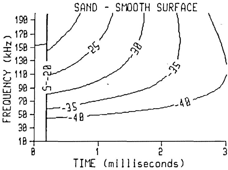
Figure 4. Contour plots of expected echo intensity versus time and frequency for Smooth Surface, Rough Surface (same as Coarse Sand in Figure 3), and Very Rough Surface.
