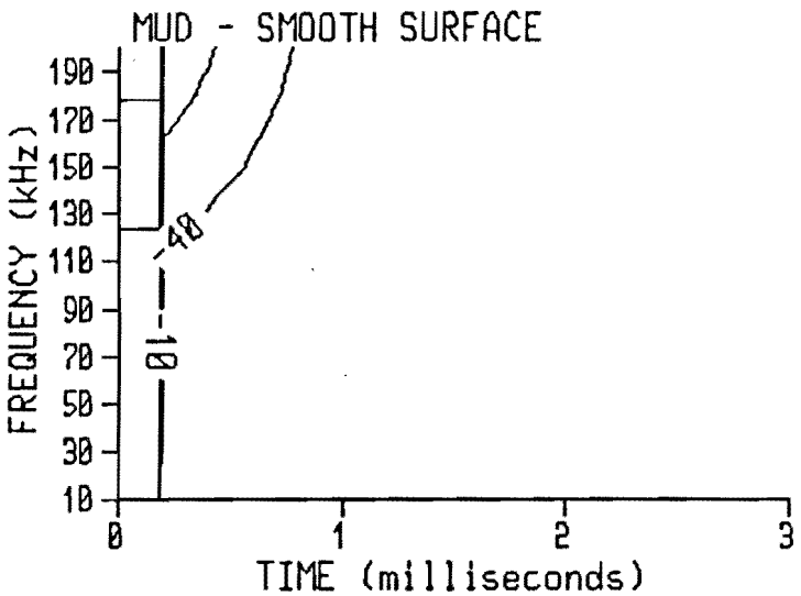
Figure 3. Contour plots of expected echo intensity versus time and frequency for Smooth Mud, Fine Sand and Coarse Sand.
