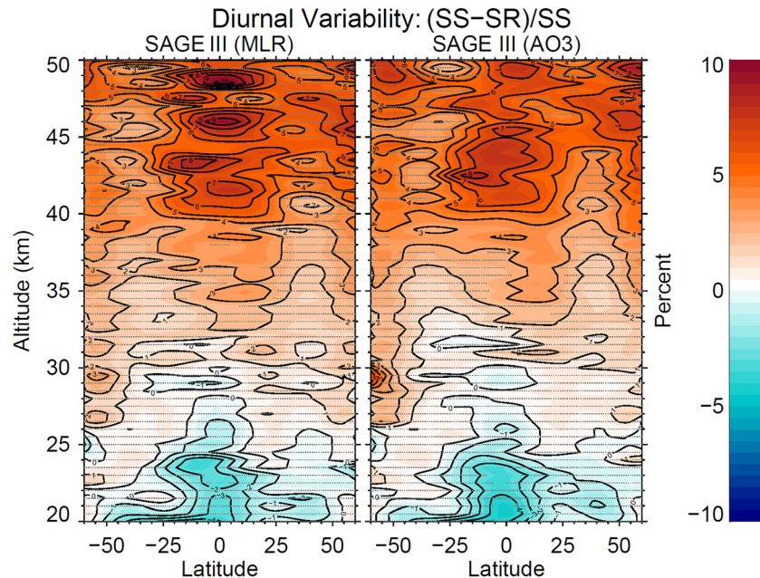
Figure 6. Mean differences between SAGE III/ISS sunrise (SR) and sunset (SS) ozone values from regression model analysis. Results from both MLR (left) and AO3 (right) algorithms are shown. The percentage difference is expressed as (SS-SR)/SS * 100\% . The very fine resolution stippling denotes regions that are not statistically significant at the two-sigma level.
