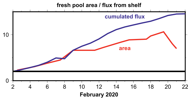
Figure 10. The area of the deep ocean sector with S < 35 pss and with depth larger than 100-m (in red; area expressed in 10^4 km 2 ); the cumulated flux is the horizontal area with S < 35 pss fed by advection from the shelf, estimated assuming horizontal dynamics, no mixing and conservation of surface salinity (in blue).
