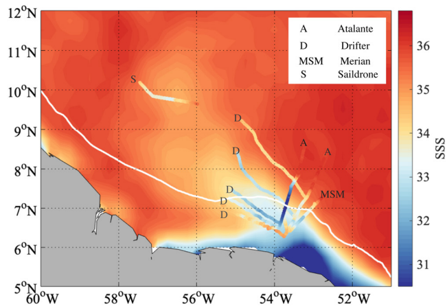
Figure 2. Average for February 2–19, 2020 of the daily salinity fields based on SMOS and SMAP satellite data, overlaid with the data collected by the various observing platforms within the fresh plume (A for R/V Atalante on February 2 and 5, Maria S. Merian (MSM) for R/V MSM on February 2; D for drifters on February 2–7 and S for Sairdron during February 16–18). The different tracks/trajectories are color-coded with observed surface salinity.
