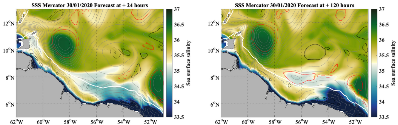
Figure 4. Mercator PSY2V4 model SSS (color) and sea level (gray contours) forecast and eddy detection made on the January 30, 2020 for January 31, 2020 (left) and February 4, 2020 (right). The eddy detection is shown by dashed contours (red for anticyclones and black for cyclones; Laxenaire et al., 2018). The shelf break is represented by the 100-m bathymetry contour (white line).
