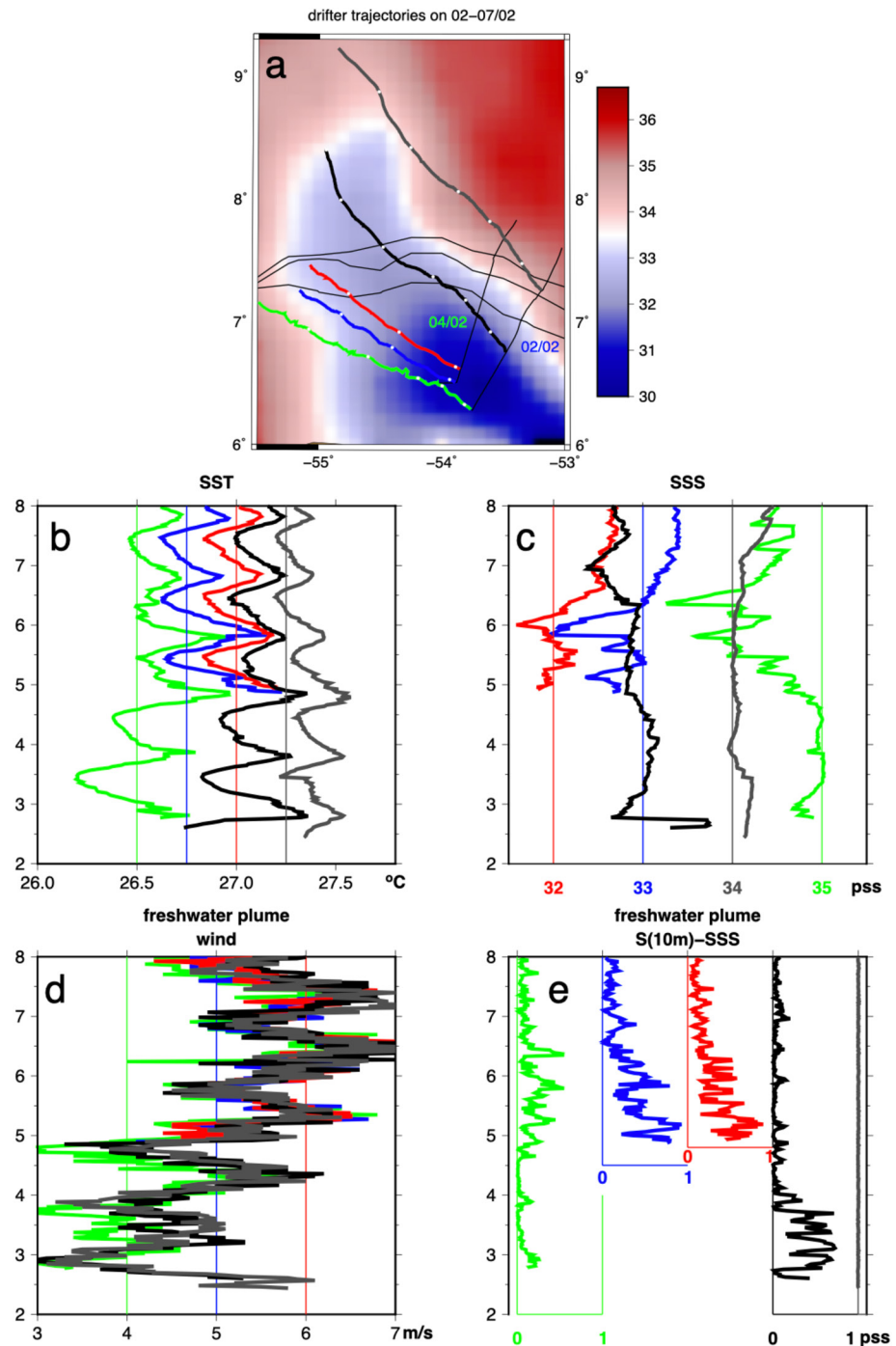
Figure 6. The drifter time series from February 2nd to 7th. Top panel, the trajectories (with dots each day at 0 GMT), as well as the SSS map for February 7. Below, four panels as a function of time (vertical axis in February days) for sea surface temperature (b, top left), sea surface salinity (c, top right), measured winds (d, bottom left in m/s), and salinity stratification S(10\text{ m})-S(0.2\text{ m}) (e, lower right). The curves are color-coded for the different drifters based on panel (a) (panel (e), the colored vertical straight lines correspond to no-stratification for that drifter).
