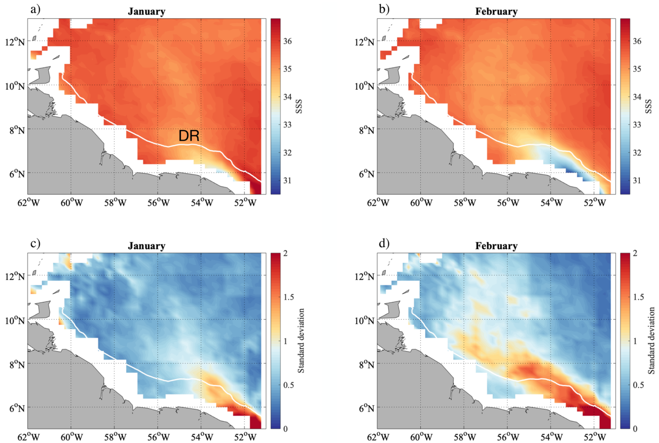
Figure 1. Average salinity and its standard deviation based on weekly satellite sea surface salinity (Climate Change Initiative products) in 2010–2019. Upper panels: averages for January and February, and lower panels the corresponding standard deviations. DR indicates Demerara Rise location.
