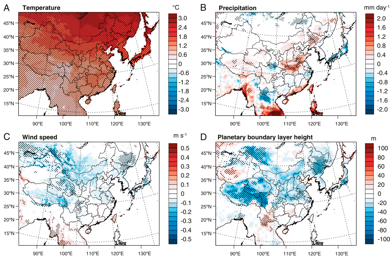
Fig. 1. Projected multiyear mean changes in major meteorological variables over East Asia. Projected mean changes in surface air temperature ( A ), precipitation ( B ), surface wind speed ( C ), and planetary boundary layer height ( D ) over East Asia are shown from current (2006 to 2010) to future (2046 to 2050) years under RCP4.5. The dots denote areas where changes are statistically significant at the 90% level, as determined by a Student's 2-sample t test.
