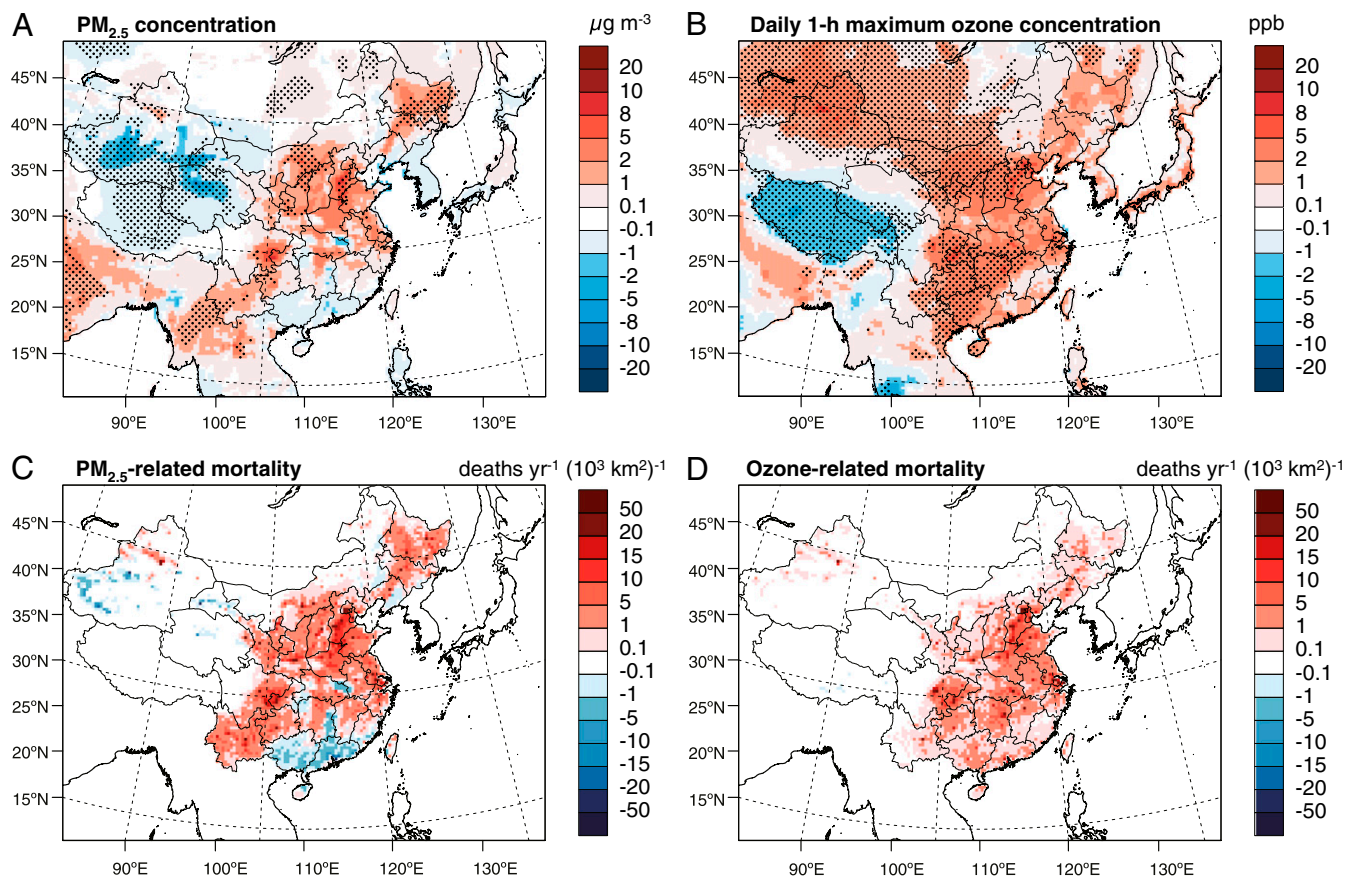
Fig. 2. Projected multiyear mean changes in air quality due to climate change and the associated health impacts in China. Projected changes in mean annual PM_{2.5} concentrations (A) and the ozone season average of daily 1-h maximum ozone (B) over East Asia related to climate change under RCP4.5 are shown from current (2006 to 2010) to future (2046 to 2050) years. The estimated changes in annual mortality in China due to the climate-related changes in PM_{2.5} (C) and ozone (D) exposure are shown. The dots in A and B denote areas where changes are statistically significant at the 90% level, as determined by a Student's 2-sample t test.
