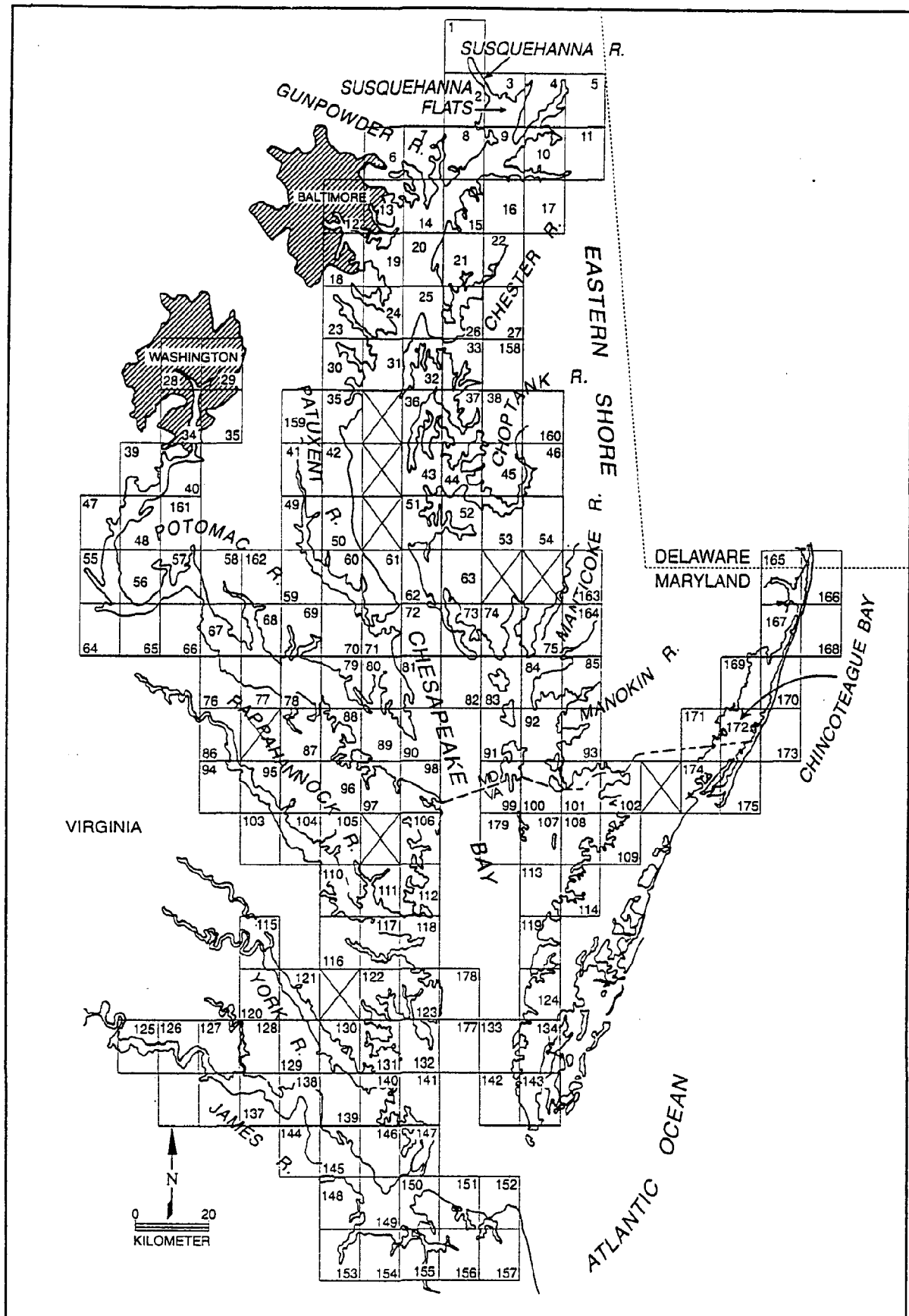
Figure 5. Location of USGS 7.5 minute quadrangles in the Chesapeake Bay, its tributaries, and in Chincoteague Bay with corresponding code numbers . (See Table 2 for quad names.)
