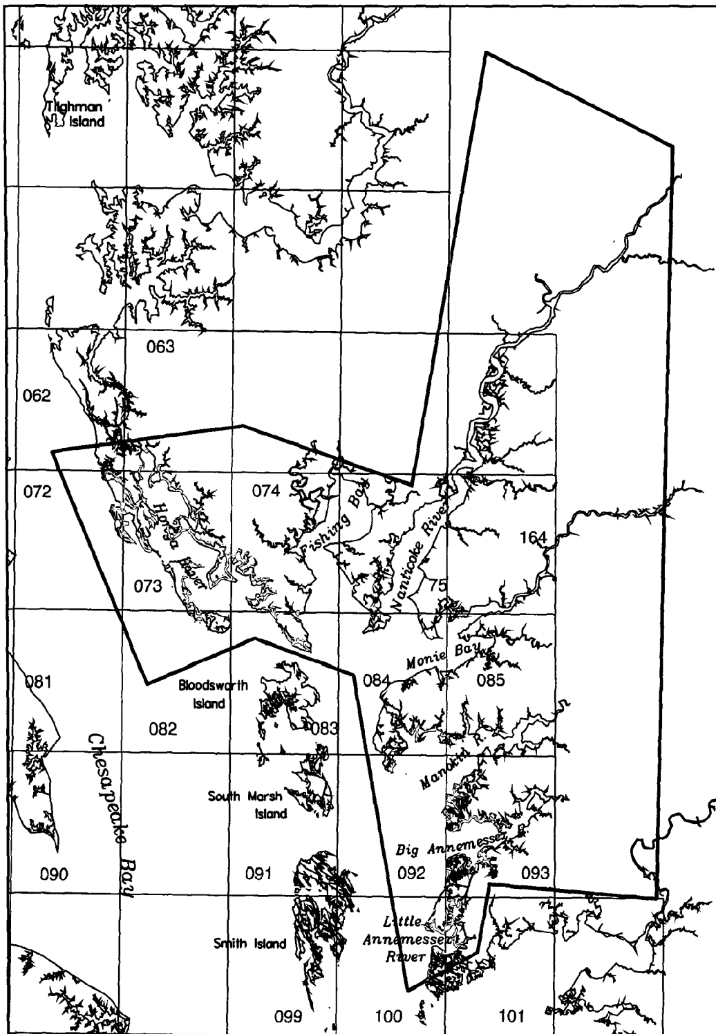
Figure 19. Distribution of SAV in the Middle Eastern Shore in 1992 (Section 12).
