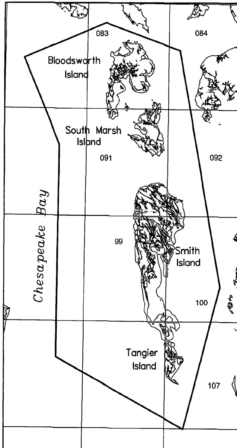
Figure 20. Distribution of SAV in the Mid-Bay Island Complex in 1992 (Section 13).
