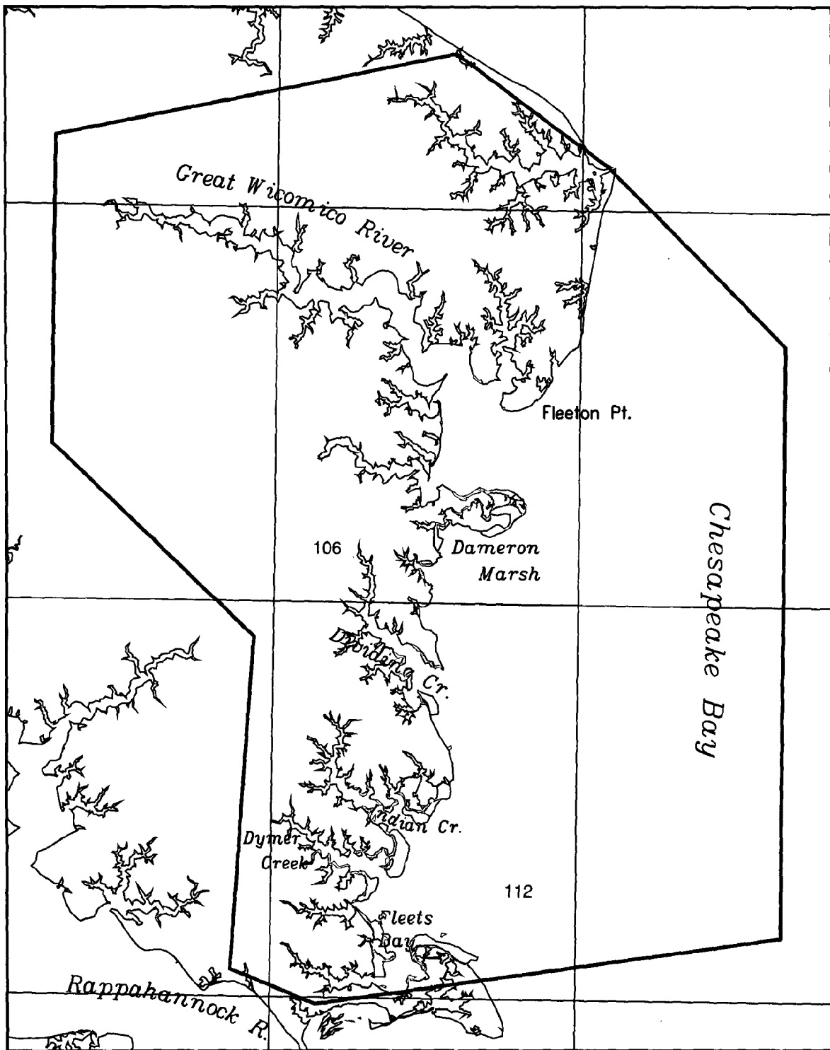
Figure 22. Distribution of SAV in the Reedville Region in 1992 (Section 15).
