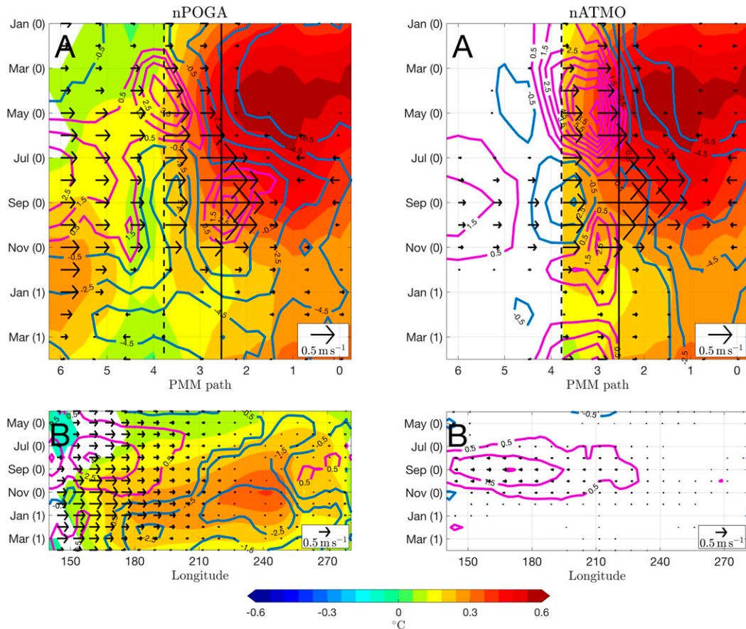
FIG. 6. (left) nPOGA and (right) nATMO ensemble mean Hovmöllers composited on the PMM_{CV} index (see text), and following paths A and B shown in Fig. 5. Shading denotes SSTAs ( ^{\circ}\text{C} ), colored contours indicate latent heat flux anomalies ( \text{W m}^{-2} ; positive downward), and arrows represent the zonal component of the 10 m wind ( \text{m s}^{-1} ). The solid black line indicates the edge of the SST restoring region (see section 2), and the dashed black line indicates the edge of the buffer zone. Results are shown only when significant at the 95% confidence level.
