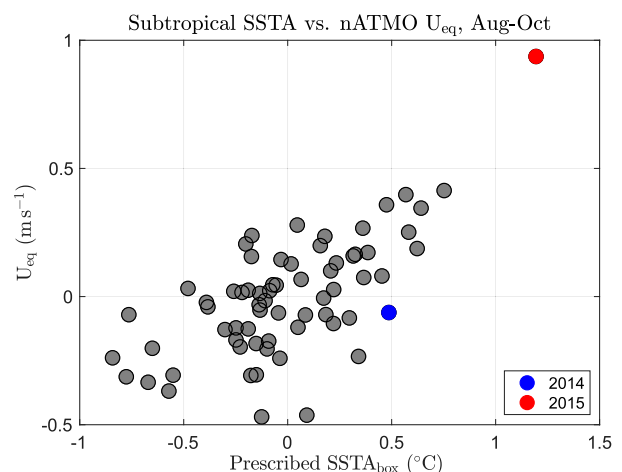
FIG. 9. Scatter of SSTA ( ^{\circ}\text{C} ) used to force nATMO, averaged in the subtropical black box in Fig. 8a (x axis), vs nATMO ensemble mean zonal wind anomalies ( \text{m s}^{-1} ) averaged in the equatorial black box in Fig. 8b (y axis). Blue and red dots represent values for 2014 and 2015, respectively.
